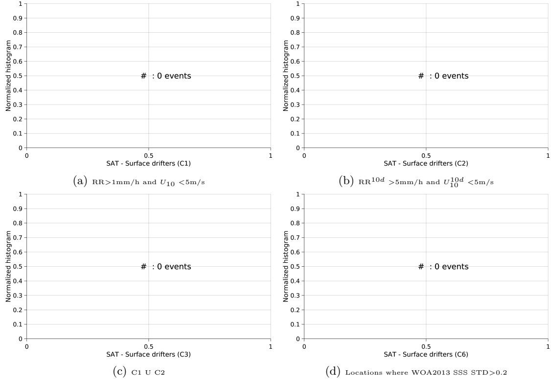
Figure 12: Normalized histogram of \Delta SSS (SMAP-L3-RSS-V2-8DAY-RUNNING-40KM - Surface drifters) for 6 different subdatasets corresponding to: RR > 1\text{mm/h} and U_{10} < 5\text{m/s} (a), RR^{10d} > 5\text{mm/h} and U_{10}^{10d} < 5\text{m/s} (b), C1 \cup C2 (c), Locations where WOA2013 SSS STD > 0.2 (d).
