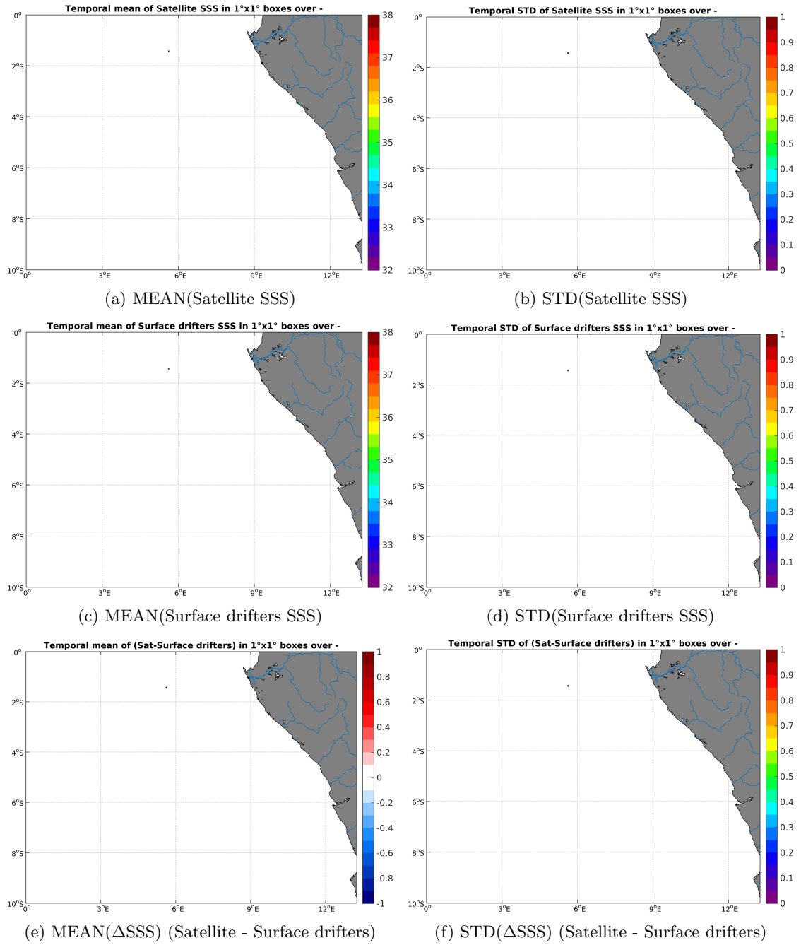
Figure 5: Temporal mean (left) and STD (right) of SSS from SMAP-L3-RSS-V2-8DAY-RUNNING-40KM (top), Surface drifters (middle), and of \Delta SSS (Satellite - Surface drifters). Only match-up pairs are used to generate these maps.
