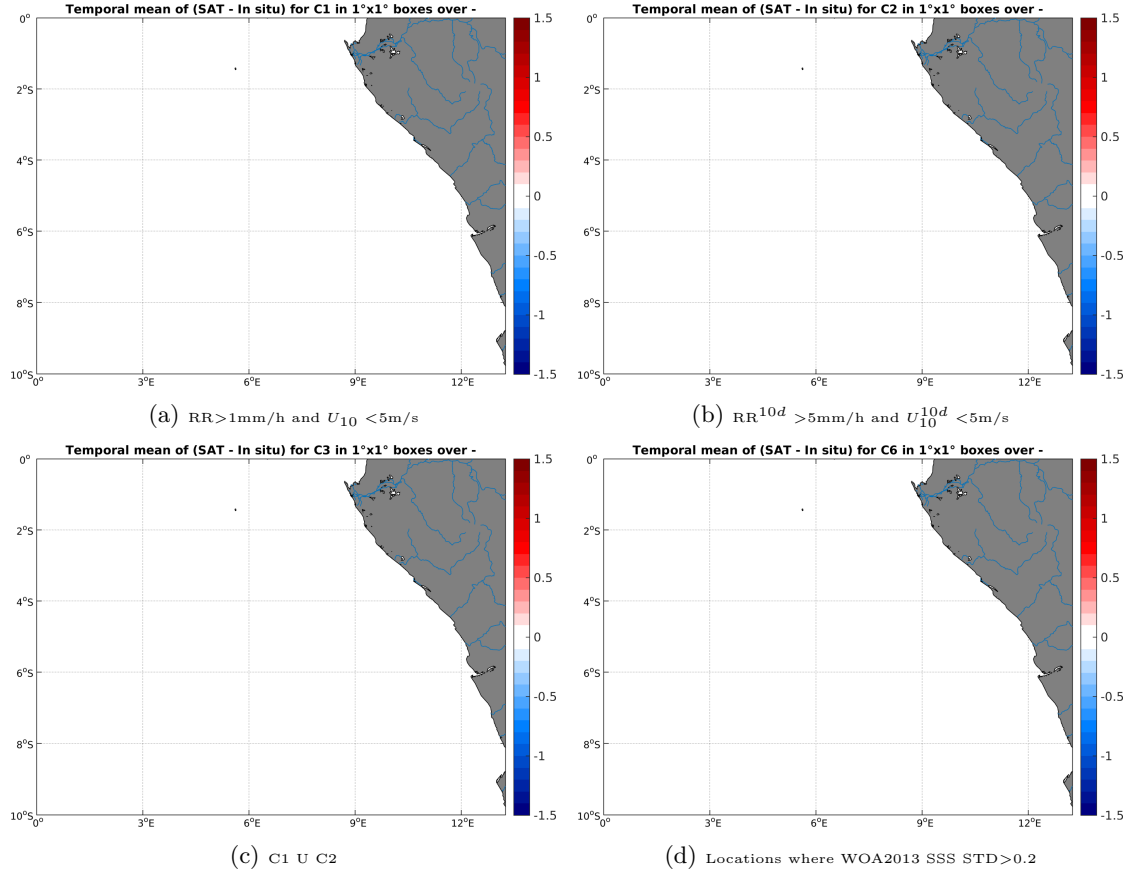
Figure 11: Temporal mean gridded over spatial boxes of size 1^\circ \times 1^\circ of \Delta SSS (SMAP-L3-RSS-V2-8DAY-RUNNING-40KM - Surface drifters) for 4 different subdatasets corresponding to: RR > 1\text{mm/h} and U_{10} < 5\text{m/s} (a), RR^{10d} > 5\text{mm/h} and U_{10}^{10d} < 5\text{m/s} (b), C1 U C2 (c), Locations where WOA2013 SSS STD > 0.2 (d).
