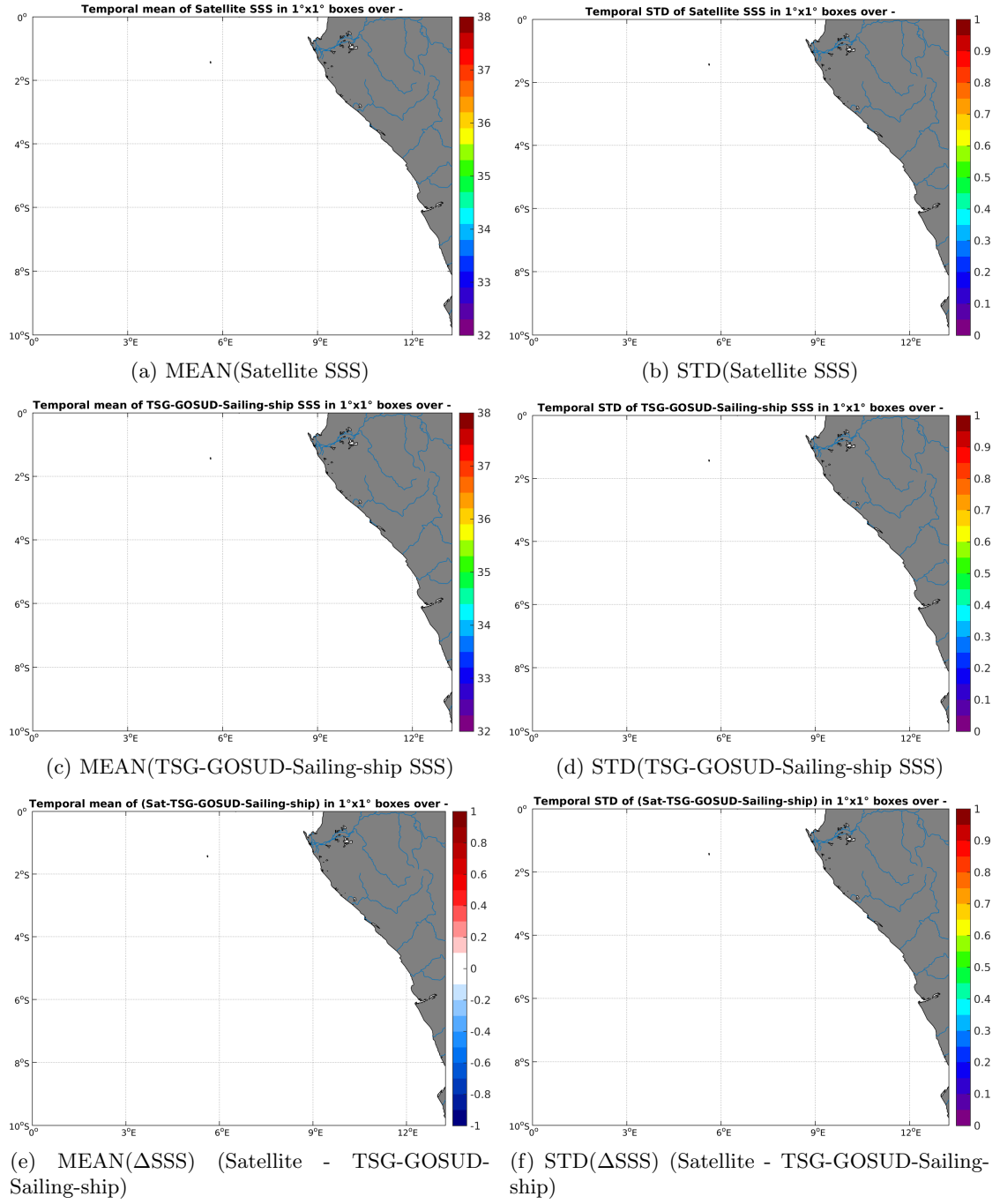
Figure 6: Temporal mean (left) and STD (right) of SSS from SMAP-L3-RSS-V2-8DAY-RUNNING-70KM (top), TSG-GOSUD-Sailing-ship (middle), and of \Delta SSS (Satellite - TSG-GOSUD-Sailing-ship). Only match-up pairs are used to generate these maps.
