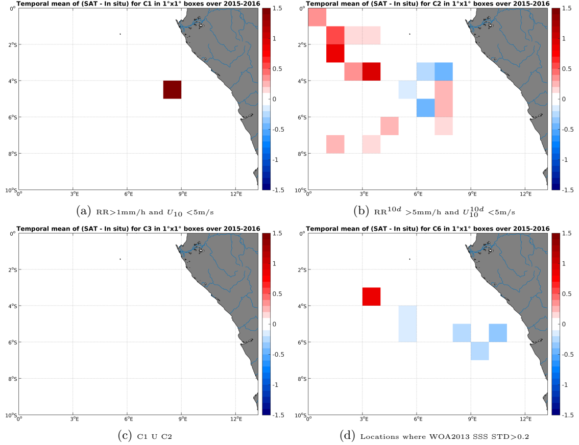
Figure 12: Temporal mean gridded over spatial boxes of size 1^\circ \times 1^\circ of \Delta SSS (SMAP-L3-RSS-V2-8DAY-RUNNING-70KM - TSG-GOSUD-Research-vessel) for 4 different subdatasets corresponding to: RR > 1 mm/h and U_{10} < 5 m/s (a), RR 10d > 5 mm/h and U_{10}^{10d} < 5 m/s (b), C1 U C2 (c), Locations where WOA2013 SSS STD > 0.2 (d).
