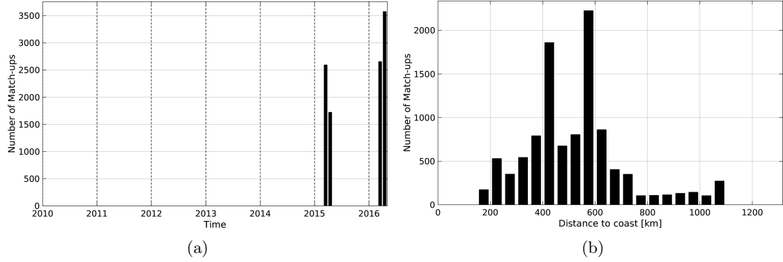
Figure 1: Number of match-ups between TSG-GOSUD-Research-vessel and SMAP-L3-RSS-V2-8DAY-RUNNING-70KM SSS as a function of time (a) and as function of the distance to coast (b) over the Congo river plume Pi-MEP region and for the full satellite product period.
