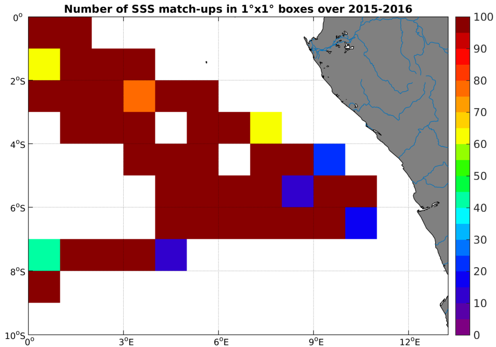
Figure 4: Number of SSS match-ups between TSG-GOSUD-Research-vessel SSS and the SMAP-L3-RSS-V2-8DAY-RUNNING-70KM SSS product for the Congo river plume Pi-MEP region over 1^\circ \times 1^\circ boxes and for the full satellite product period.
