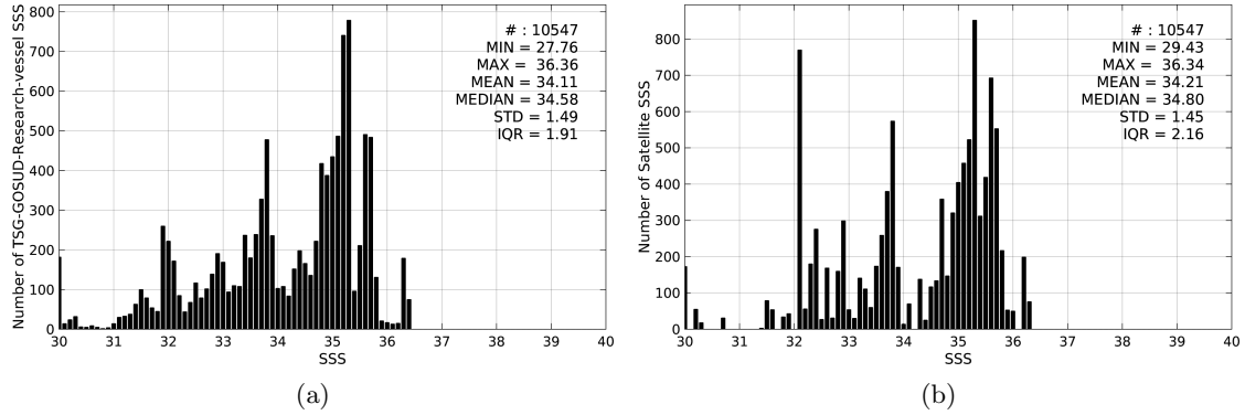
Figure 2: Histograms of SSS from TSG-GOSUD-Research-vessel (a) and SMAP-L3-RSS-V2-8DAY-RUNNING-70KM (b) considering all match-up pairs per bins of 0.1 over the Congo river plume Pi-MEP region and for the full satellite product period.
