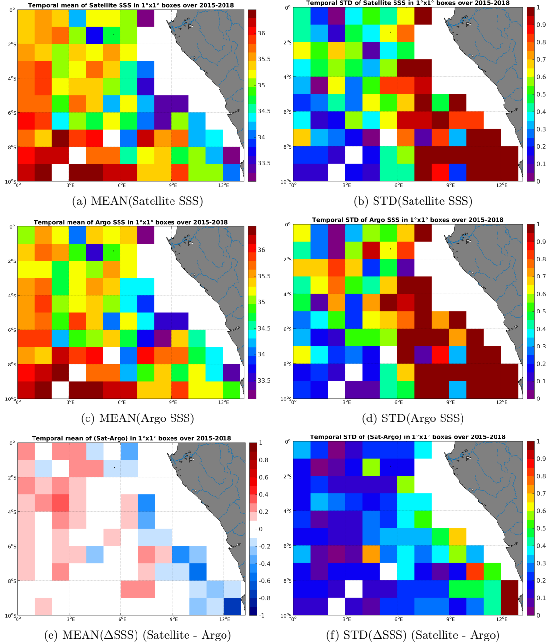
Figure 6: Temporal mean (left) and STD (right) of SSS from SMAP-L3-RSS-V2-8DAY-RUNNING-70KM (top), Argo (middle), and of \Delta SSS (Satellite - Argo). Only match-up pairs are used to generate these maps.
