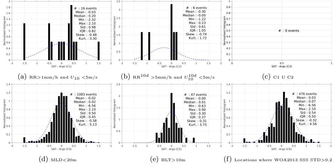
Figure 13: Normalized histogram of \Delta SSS (SMAP-L3-RSS-V2-8DAY-RUNNING-70KM - Argo) for 6 different subdatasets corresponding to: RR > 1\text{mm/h} and U_{10} < 5\text{m/s} (a), RR^{10d} > 5\text{mm/h} and U_{10}^{10d} < 5\text{m/s} (b), C1 \cup C2 (c), MLD < 20\text{m} (d), BLT > 10\text{m} (e), Locations where WOA2013 SSS STD > 0.2 (f).
