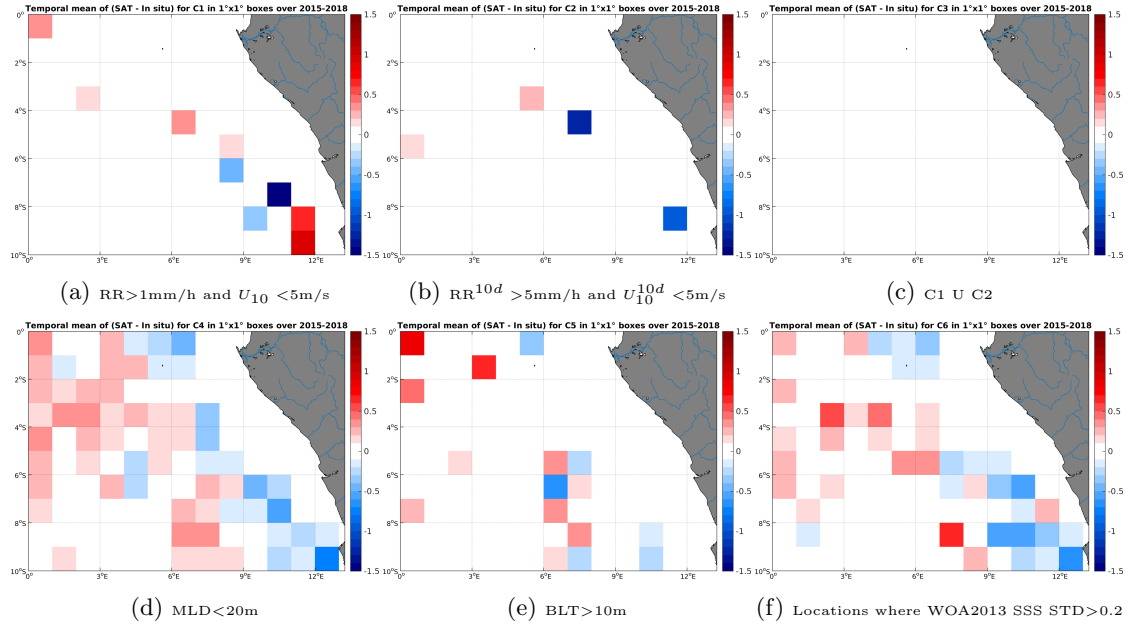
Figure 12: Temporal mean gridded over spatial boxes of size 1^\circ \times 1^\circ of \Delta SSS (SMAP-L3-RSS-V2-8DAY-RUNNING-70KM - Argo) for 6 different subdatasets corresponding to: RR > 1mm/h and U_{10} < 5 m/s (a), RR^{10d} > 5 mm/h and U_{10}^{10d} < 5 m/s (b), C1 U C2 (c), MLD < 20m (d), BLT > 10m (e), Locations where WOA2013 SSS STD > 0.2 (f).
