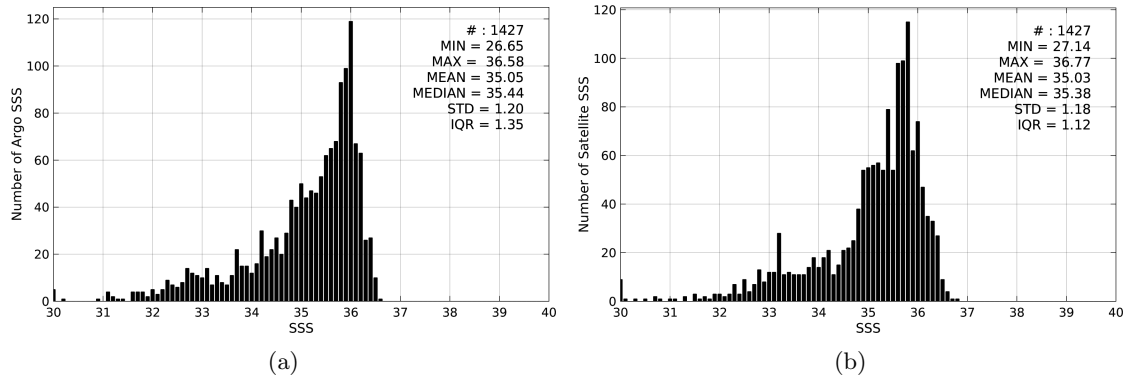
Figure 2: Histograms of SSS from Argo (a) and SMAP-L3-RSS-V2-8DAY-RUNNING-70KM (b) considering all match-up pairs per bins of 0.1 over the Congo river plume Pi-MEP region and for the full satellite product period.
