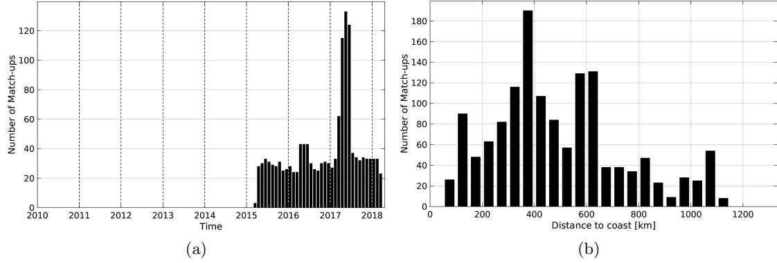
Figure 1: Number of match-ups between Argo and SMAP-L3-RSS-V2-8DAY-RUNNING-70KM SSS as a function of time (a) and as function of the distance to coast (b) over the Congo river plume Pi-MEP region and for the full satellite product period.
