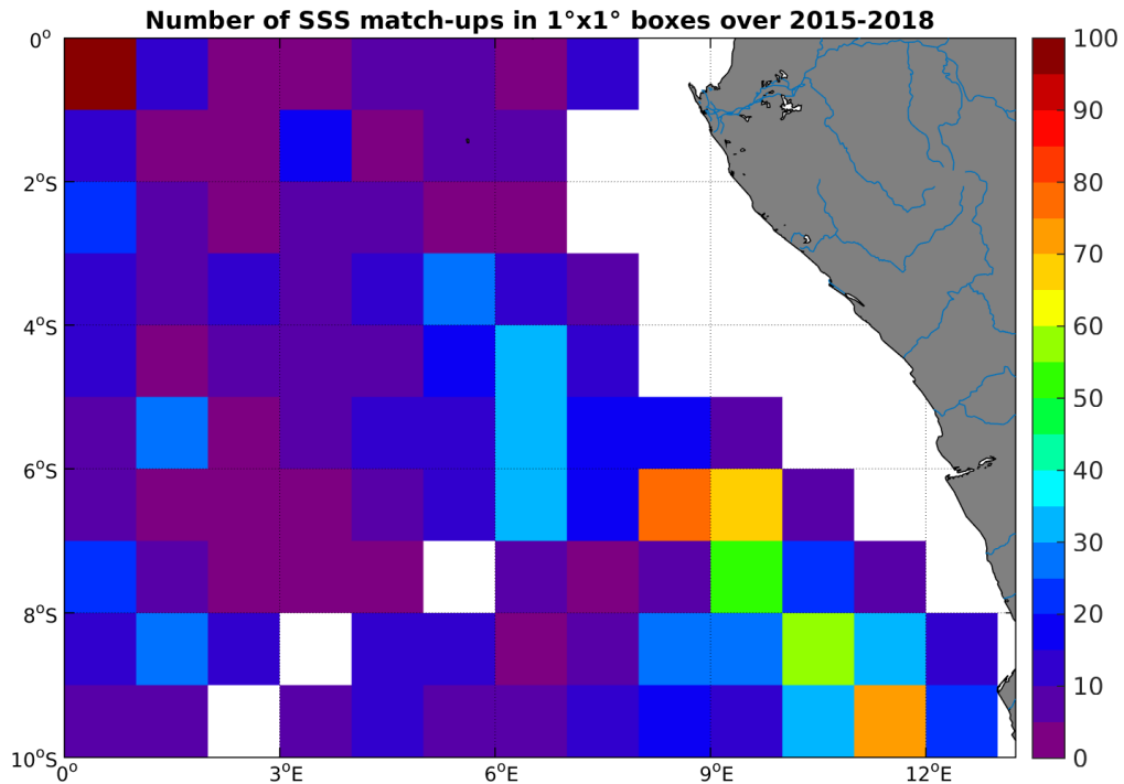
Figure 4: Number of SSS match-ups between Argos SSS and the SMAP-L3-RSS-V2-8DAY-RUNNING-70KM SSS product for the Congo river plume Pi-MEP region over 1^\circ \times 1^\circ boxes and for the full satellite product period.
