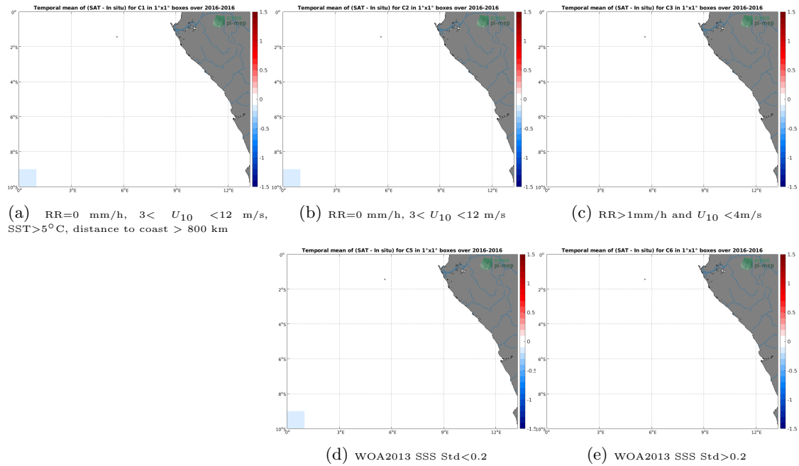
Figure 12: Temporal mean gridded over spatial boxes of size 1^{\circ}\times 1^{\circ} of \Delta\text{SSS} (SMAP SSS L3 v5.0 - Monthly (JPL) - TSG (Polarstern)) for 5 different subdatasets corresponding to:RR=0 mm/h, 3 < U_{10} < 12 m/s, SST >5^{\circ}\text{C} , distance to coast > 800 km (a), RR=0 mm/h, 3 < U_{10} < 12 m/s (b), RR >1 mm/h and U_{10} < 4 m/s (c), WOA2013 SSS Std <0.2 (d), WOA2013 SSS Std >0.2 (e).
