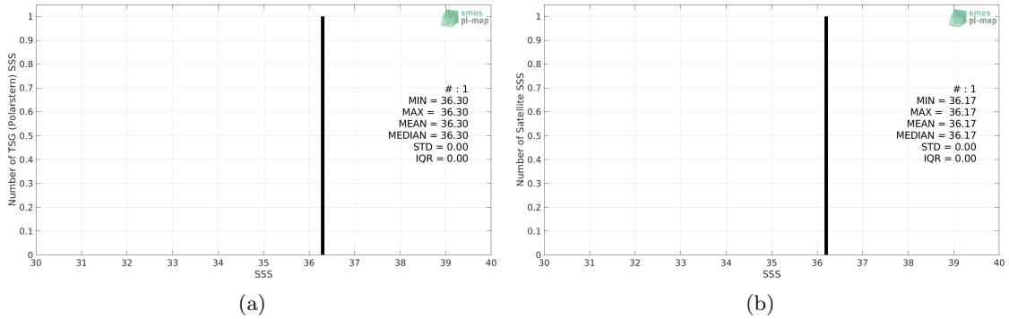
Figure 2: Histograms of SSS from TSG (Polarstern) (a) and SMAP SSS L3 v5.0 - Monthly (JPL) (b) considering all match-up pairs per bins of 0.1 over the Congo river plume Pi-MEP region and for the full satellite product period.
