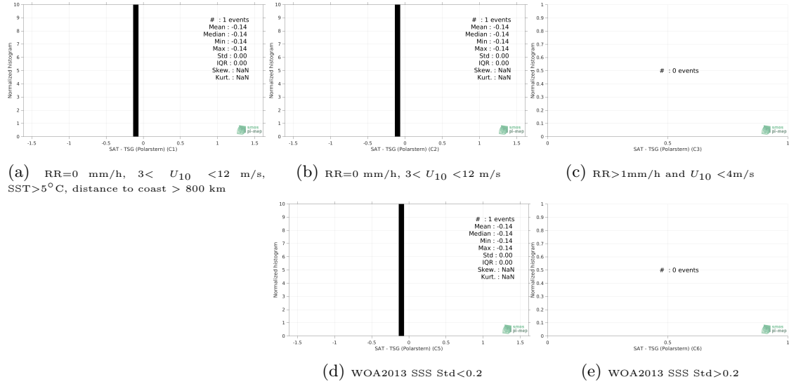
Figure 13: Normalized histogram of \Delta\text{SSS} (SMAP SSS L3 v5.0 - Monthly (JPL) - TSG (Polarstern)) for 5 different subdatasets corresponding to: RR=0 mm/h, 3 < U_{10} < 12 m/s, SST > 5^\circ\text{C} , distance to coast > 800 km (a), RR=0 mm/h, 3 < U_{10} < 12 m/s (b), RR > 1\text{mm/h} and U_{10} < 4\text{m/s} (c), WOA2013 SSS \text{Std} < 0.2 (d), WOA2013 SSS \text{Std} > 0.2 (e).
