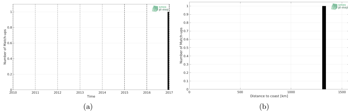
Figure 1: Number of match-ups between TSG (Polarstern) and SMAP SSS L3 v5.0 - Monthly (JPL) SSS as a function of time (a) and as function of the distance to coast (b) over the Congo river plume Pi-MEP region and for the full satellite product period.
