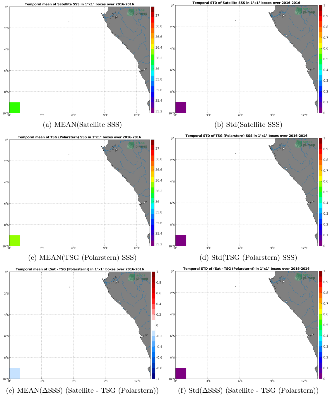
Figure 6: Temporal mean (left) and Std (right) of SSS from SMAP SSS L3 v5.0 - Monthly (JPL) (top), TSG (Polarstern) (middle), and of \Delta SSS (Satellite - TSG (Polarstern)). Only match-up pairs are used to generate these maps.
