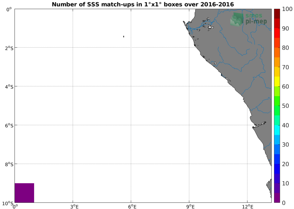
Figure 4: Number of SSS match-ups between TSG (Polarstern) SSS and the SMAP SSS L3 v5.0 - Monthly (JPL) SSS product for the Congo river plume Pi-MEP region over 1^\circ \times 1^\circ boxes and for the full satellite product period.
