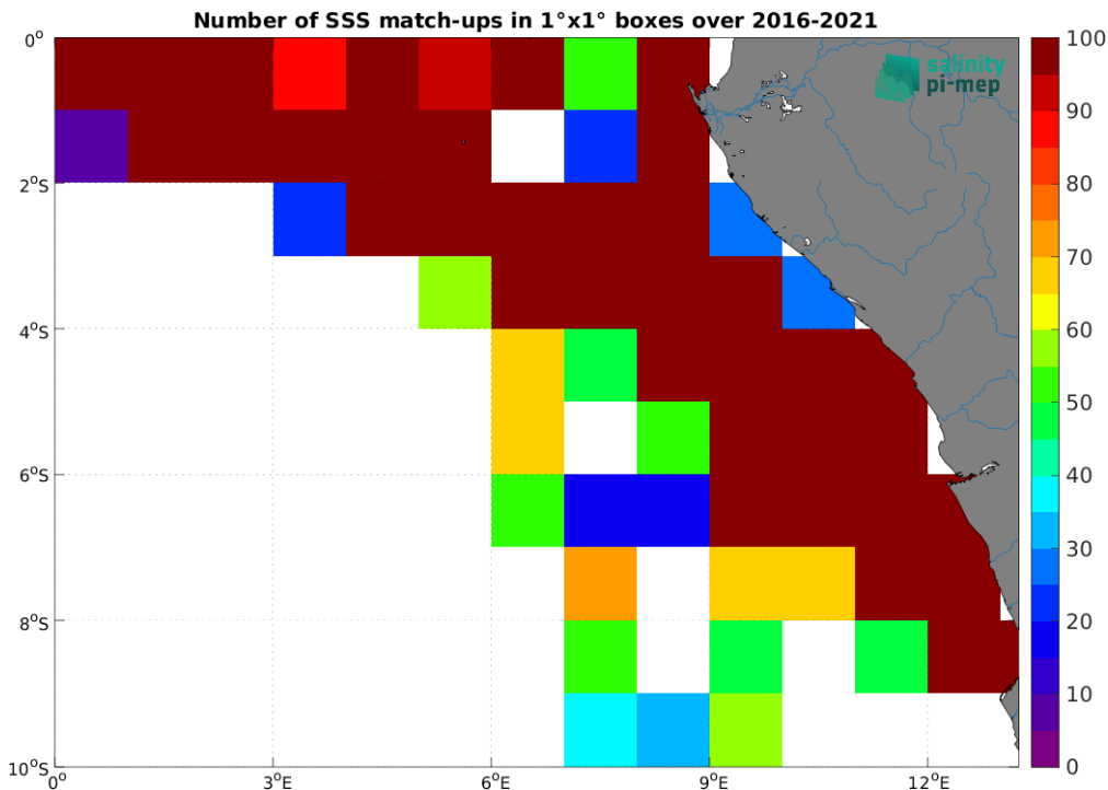
Figure 5: Number of SSS match-ups between TSG (LEGOS-DM) SSS and the SMAP SSS L3 v5.0 - Monthly (JPL) SSS product for the Congo river plume Pi-MEP region over 1^{\circ} \times 1^{\circ} boxes and for the full satellite product period.
