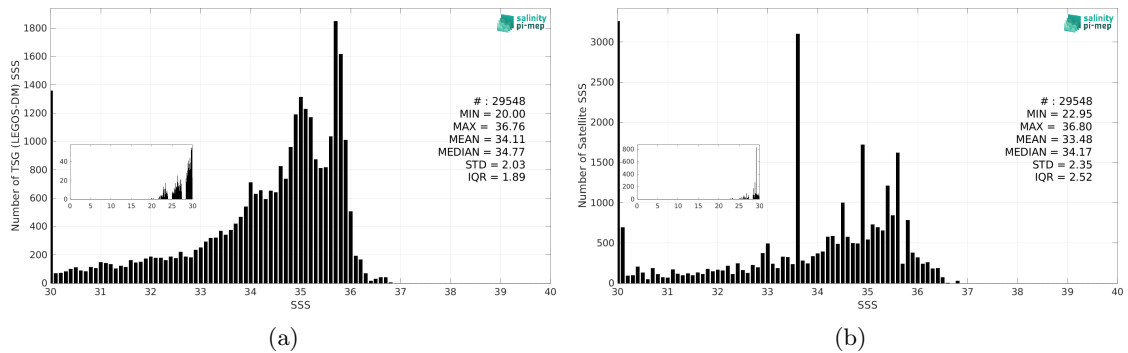
Figure 3: Histograms of SSS from TSG (LEGOS-DM) (a) and SMAP SSS L3 v5.0 - Monthly (JPL) (b) considering all match-up pairs per bins of 0.1 over the Congo river plume Pi-MEP region and for the full satellite product period.
