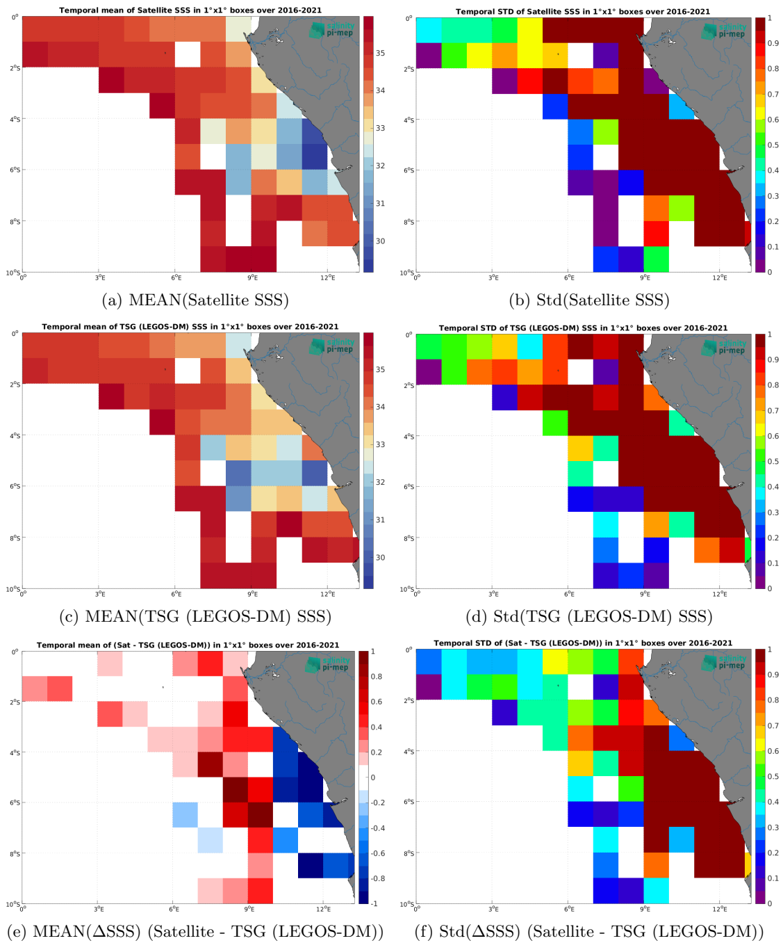
Figure 7: Temporal mean (left) and Std (right) of SSS from SMAP SSS L3 v5.0 - Monthly (JPL) (top), TSG (LEGOS-DM) (middle), and of \Delta SSS (Satellite - TSG (LEGOS-DM)). Only match-up pairs are used to generate these maps.
