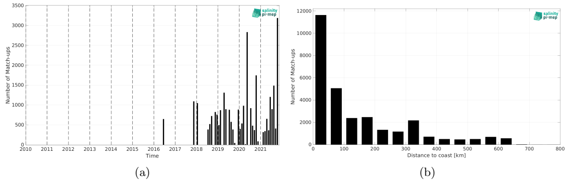
Figure 2: Number of match-ups between TSG (LEGOS-DM) and SMAP SSS L3 v5.0 - Monthly (JPL) SSS as a function of time (a) and as function of the distance to coast (b) over the Congo river plume Pi-MEP region and for the full satellite product period.
