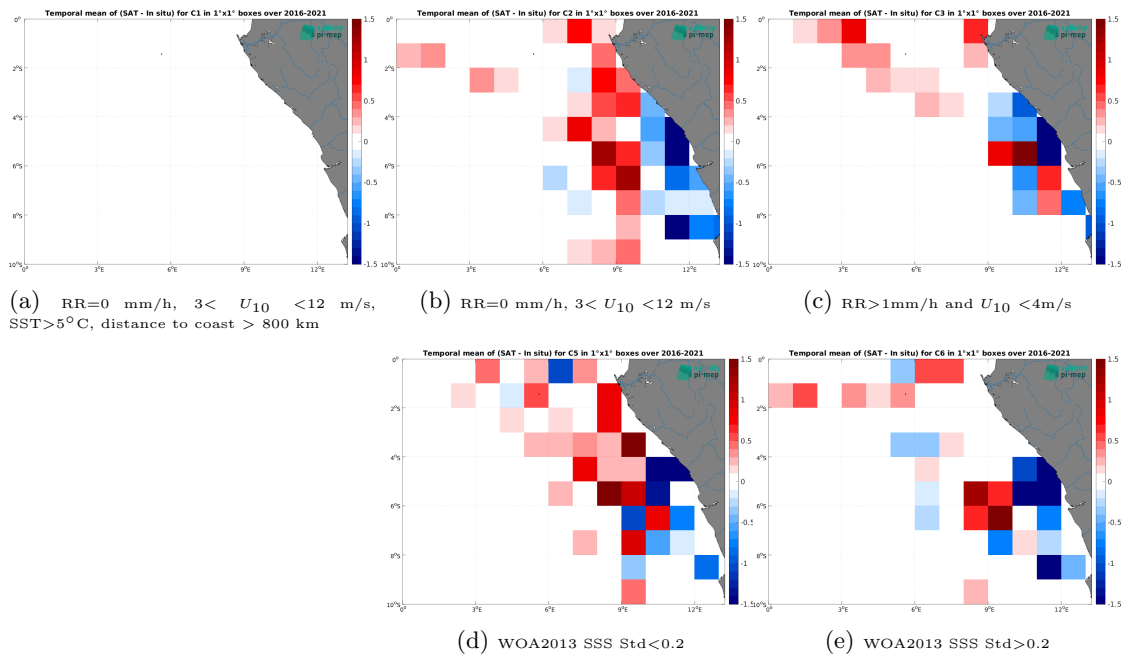
Figure 14: Temporal mean gridded over spatial boxes of size 1^\circ \times 1^\circ of \Delta SSS (SMAP SSS L3 v5.0 - Monthly (JPL) - TSG (LEGOS-DM)) for 5 different subdatasets corresponding to: RR=0 mm/h, 3 < U_{10} < 12 m/s, SST > 5°C, distance to coast > 800 km (a), RR=0 mm/h, 3 < U_{10} < 12 m/s (b), RR > 1mm/h and U_{10} < 4 m/s (c), WOA2013 SSS Std < 0.2 (d), WOA2013 SSS Std > 0.2 (e).
