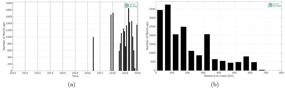
Figure 1: Number of match-ups between TSG (LEGOS-DM) and SMAP SSS L3 v5.0 - Monthly (JPL) SSS as a function of time (a) and as function of the distance to coast (b) over the Congo river plume Pi-MEP region and for the full satellite product period.
