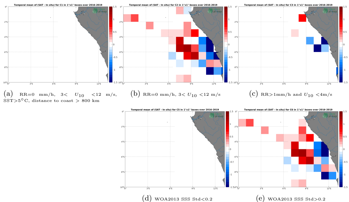
Figure 12: Temporal mean gridded over spatial boxes of size 1^\circ \times 1^\circ of \Delta\text{SSS} (SMAP SSS L3 v5.0 - Monthly (JPL) - TSG (LEGOS-DM)) for 5 different subdatasets corresponding to:RR=0 mm/h, 3 < U_{10} < 12 m/s, SST >5^\circ\text{C} , distance to coast > 800 km (a), RR=0 mm/h, 3 < U_{10} < 12 m/s (b), RR >1 mm/h and U_{10} < 4 m/s (c), WOA2013 SSS Std <0.2 (d), WOA2013 SSS Std >0.2 (e).
