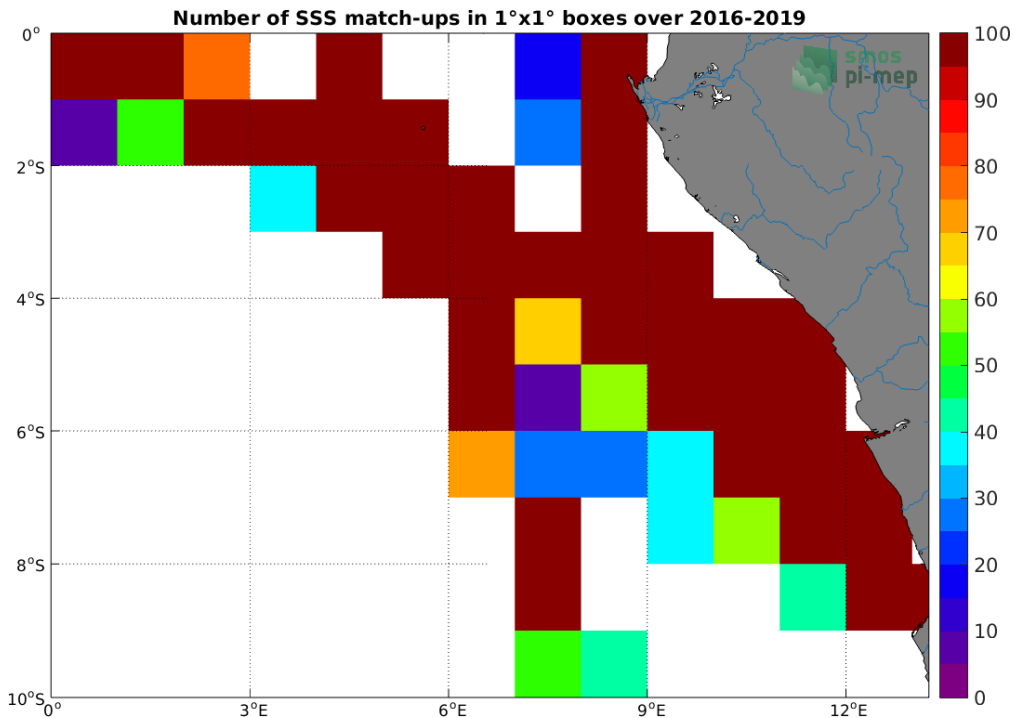
Figure 4: Number of SSS match-ups between TSG (LEGOS-DM) SSS and the SMAP SSS L3 v5.0 - Monthly (JPL) SSS product for the Congo river plume Pi-MEP region over 1^\circ \times 1^\circ boxes and for the full satellite product period.
