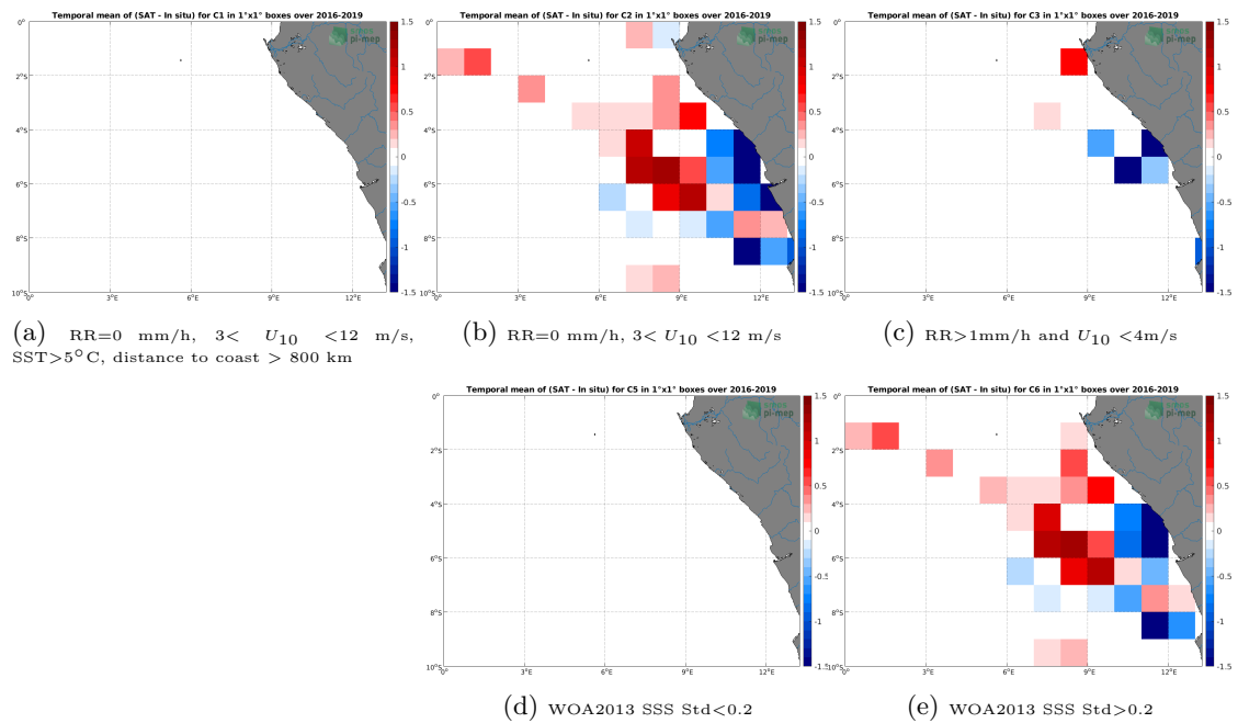
Figure 12: Temporal mean gridded over spatial boxes of size 1°x1° of \Delta SSS (SMAP SSS L3 v5.0 - Monthly (JPL) - TSG (LEGOS-DM)) for 5 different subdatasets corresponding to:RR=0 mm/h, 3 < U_{10} < 12 m/s, SST>5°C, distance to coast > 800 km (a), RR=0 mm/h, 3 < U_{10} < 12 m/s (b), RR>1mm/h and U_{10} < 4 m/s (c), WOA2013 SSS Std<0.2 (d), WOA2013 SSS Std>0.2 (e).
