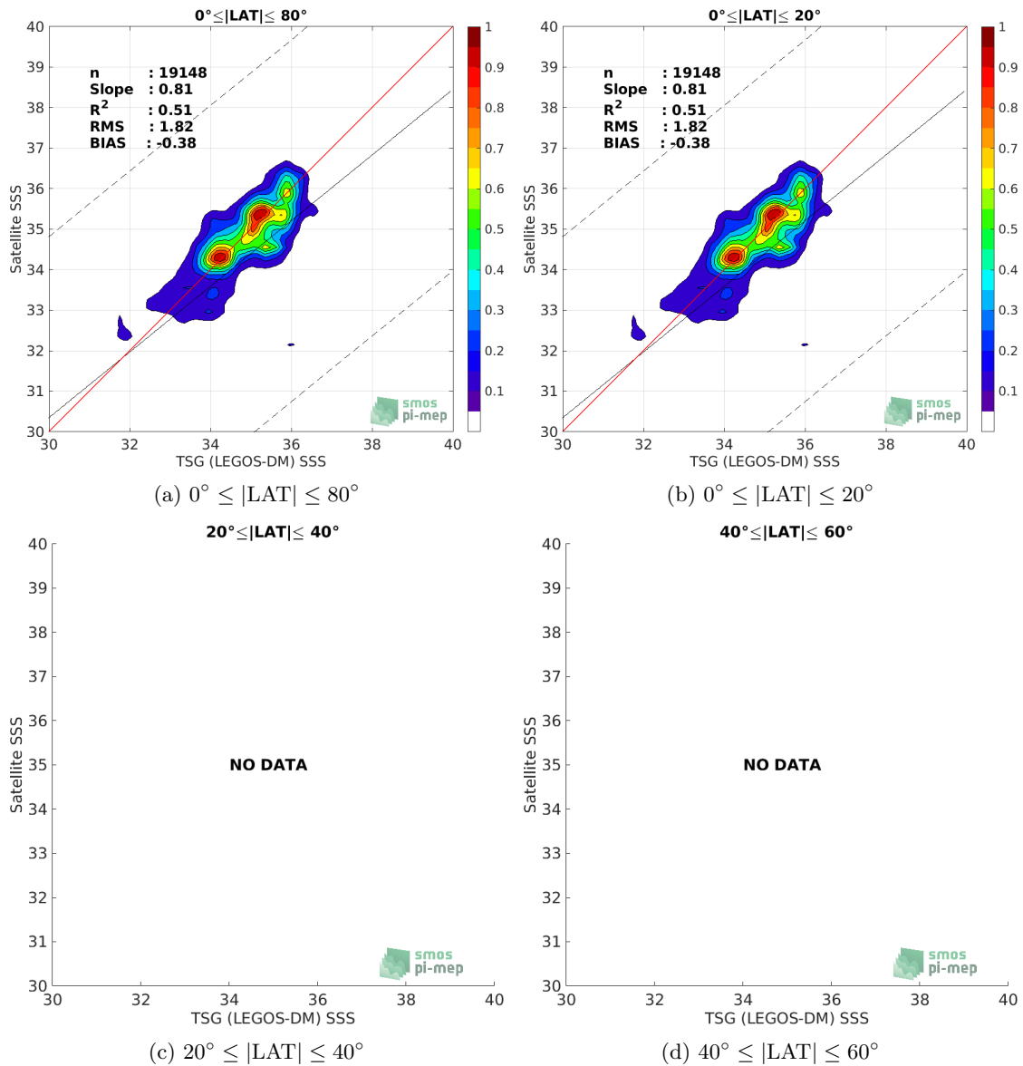
Figure 9: Contour maps of the concentration of SMAP SSS L3 v5.0 - Monthly (JPL) SSS ( y -axis) versus TSG (LEGOS-DM) SSS ( x -axis) at match-up pairs for different latitude bands. For each plot, the red line shows x=y . The black thin and dashed lines indicate a linear fit through the data cloud and the \pm 95\% confidence levels, respectively. The number match-up pairs n , the slope and R^2 coefficient of the linear fit, the root mean square (RMS) and the mean bias between satellite and in situ data are indicated for each latitude band in each plots.
