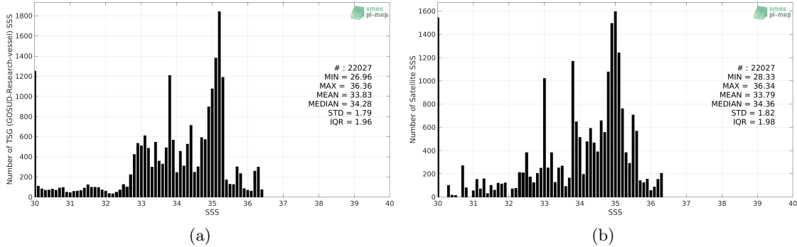
Figure 2: Histograms of SSS from TSG (GOSUD-Research-vessel) (a) and SMAP SSS L3 v5.0 - Monthly (JPL) (b) considering all match-up pairs per bins of 0.1 over the Congo river plume Pi-MEP region and for the full satellite product period.
