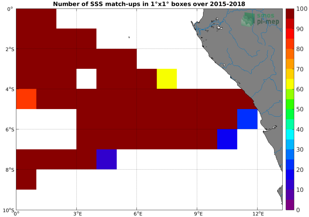
Figure 4: Number of SSS match-ups between TSG (GOSUD-Research-vessel) SSS and the SMAP SSS L3 v5.0 - Monthly (JPL) SSS product for the Congo river plume Pi-MEP region over 1°x1° boxes and for the full satellite product period.
