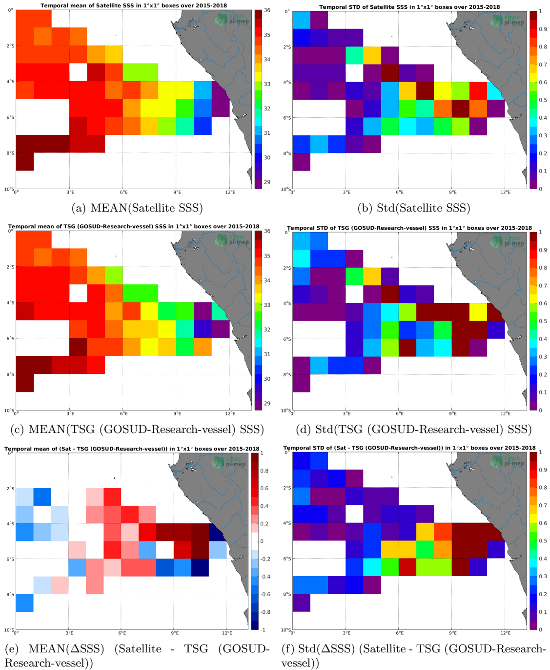
Figure 6: Temporal mean (left) and Std (right) of SSS from SMAP SSS L3 v5.0 - Monthly (JPL) (top), TSG (GOSUD-Research-vessel) (middle), and of \Delta SSS (Satellite - TSG (GOSUD-Research-vessel)). Only match-up pairs are used to generate these maps.
