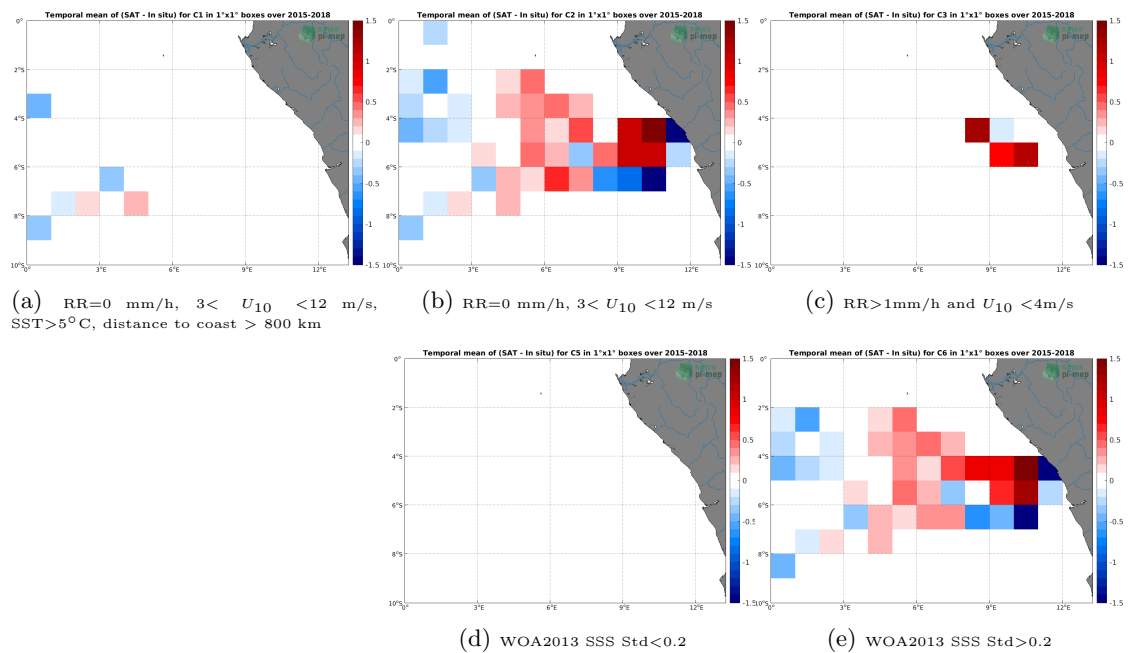
Figure 12: Temporal mean gridded over spatial boxes of size 1^\circ \times 1^\circ of \Delta SSS (SMAP SSS L3 v5.0 - Monthly (JPL) - TSG (GOSUD-Research-vessel)) for 5 different subdatasets corresponding to:RR=0 mm/h, 3 < U_{10} < 12 m/s, SST>5°C, distance to coast > 800 km (a), RR=0 mm/h, 3 < U_{10} < 12 m/s (b), RR>1mm/h and U_{10} < 4 m/s (c), WOA2013 SSS Std<0.2 (d), WOA2013 SSS Std>0.2 (e).
