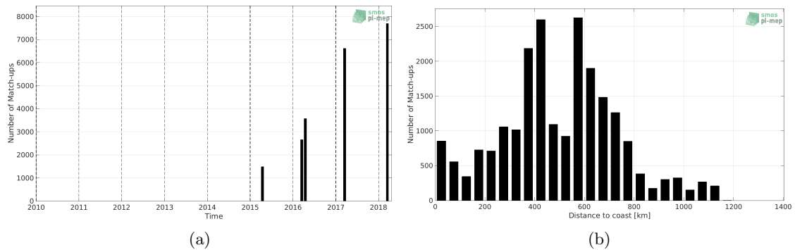
Figure 1: Number of match-ups between TSG (GOSUD-Research-vessel) and SMAP SSS L3 v5.0 - Monthly (JPL) SSS as a function of time (a) and as function of the distance to coast (b) over the Congo river plume Pi-MEP region and for the full satellite product period.
