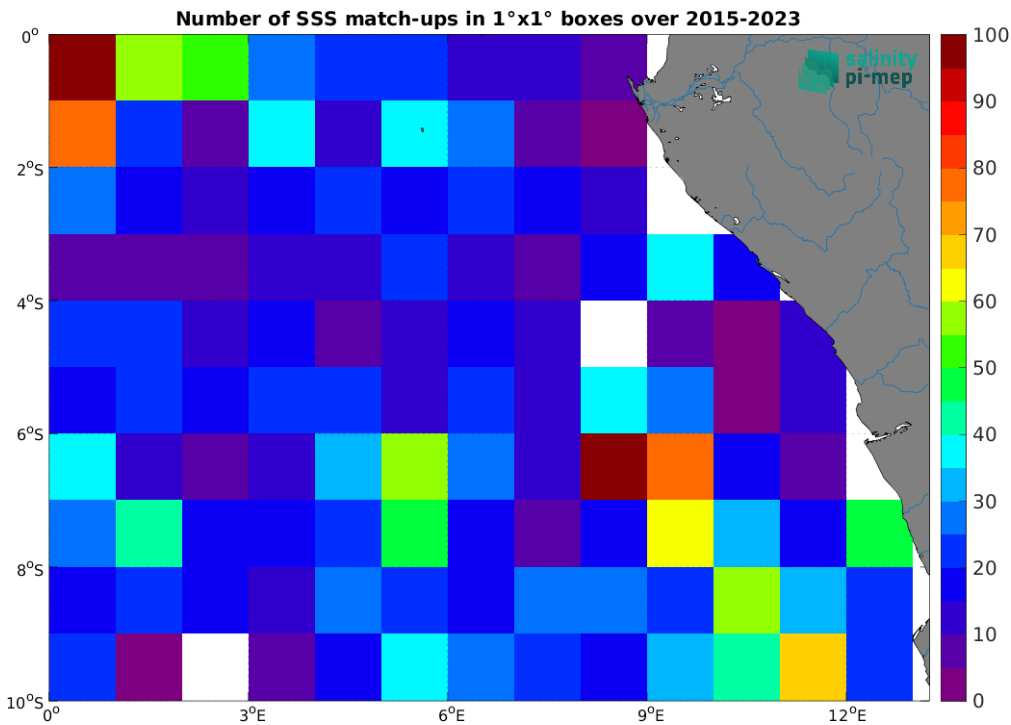
Figure 5: Number of SSS match-ups between Argo SSS and the SMAP SSS L3 v5.0 - Monthly (JPL) SSS product for the Congo river plume Pi-MEP region over 1^\circ \times 1^\circ boxes and for the full satellite product period.
