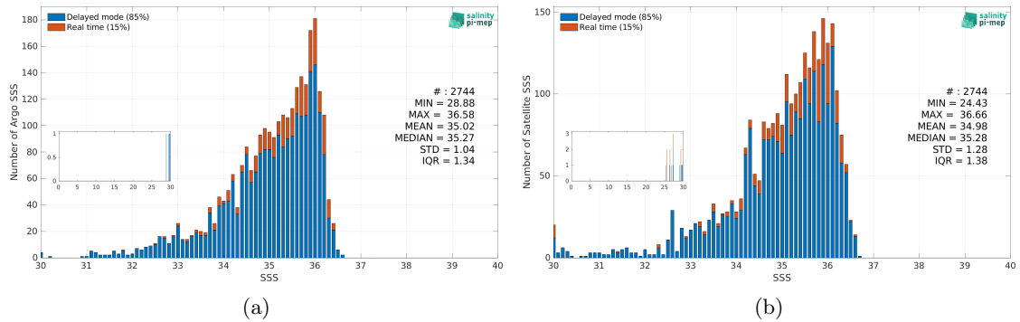
Figure 3: Histograms of SSS from Argo (a) and SMAP SSS L3 v5.0 - Monthly (JPL) (b) considering all match-up pairs per bins of 0.1 over the Congo river plume Pi-MEP region and for the full satellite product period.
