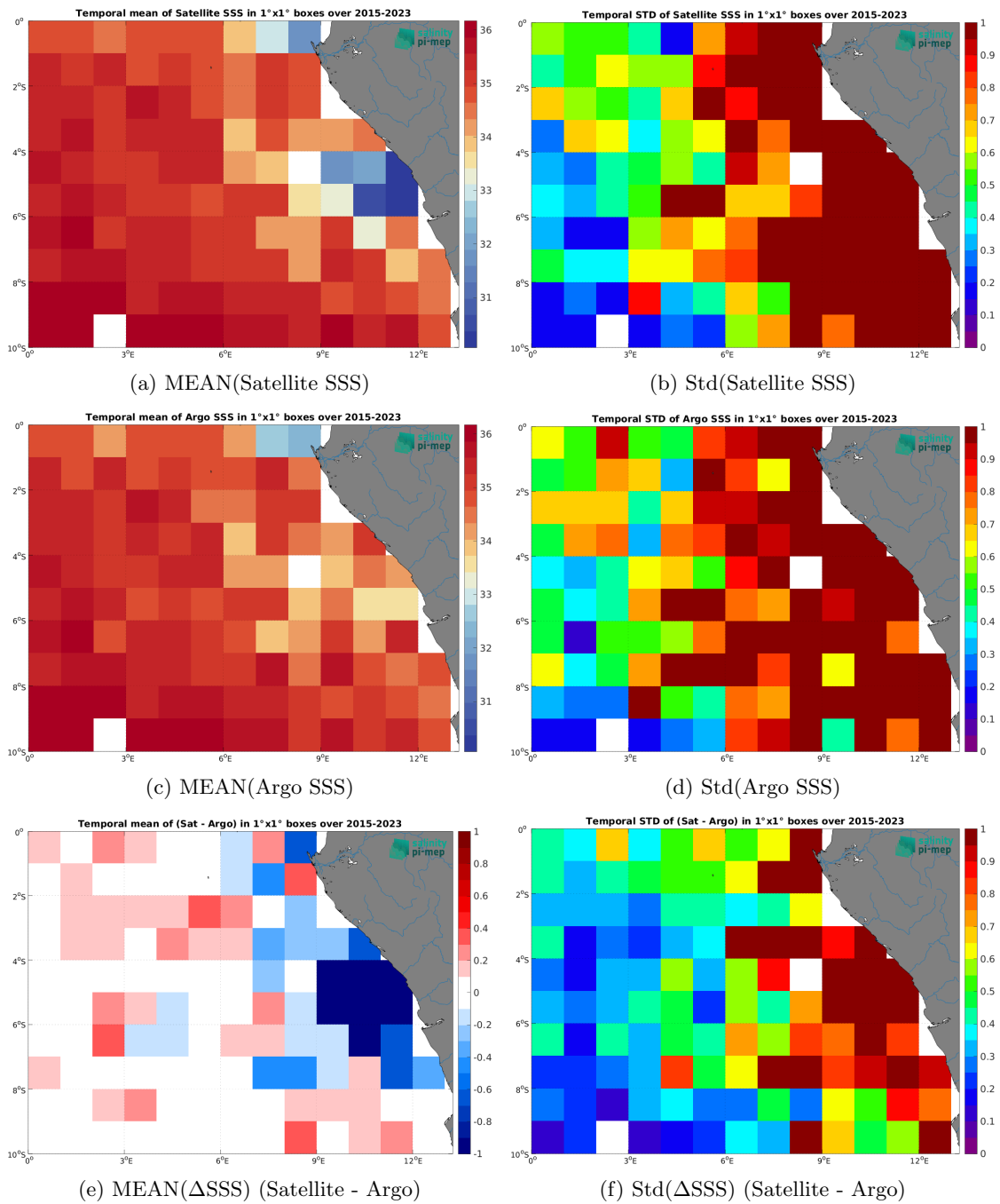
Figure 7: Temporal mean (left) and Std (right) of SSS from SMAP SSS L3 v5.0 - Monthly (JPL) (top), Argo (middle), and of \Delta SSS (Satellite - Argo). Only match-up pairs are used to generate these maps.
