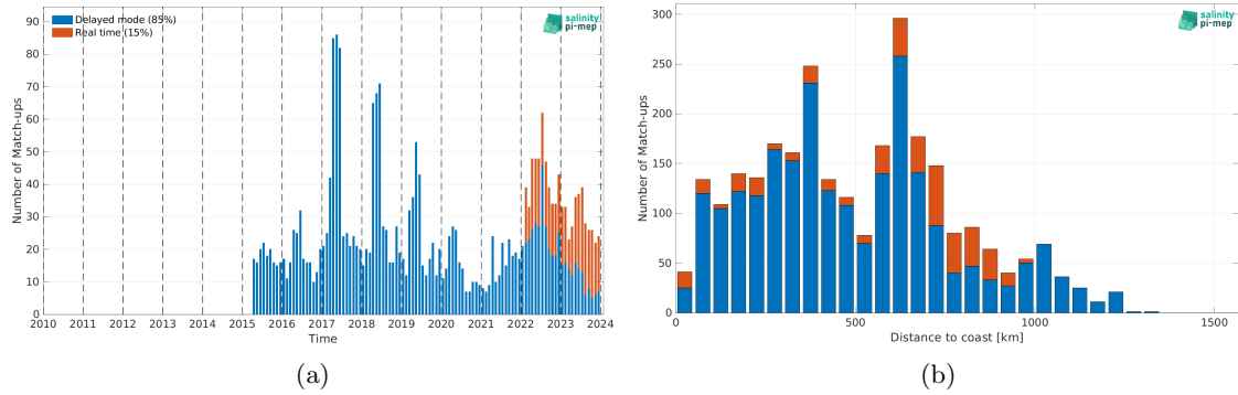
Figure 2: Number of match-ups between Argo and SMAP SSS L3 v5.0 - Monthly (JPL) SSS as a function of time (a) and as function of the distance to coast (b) over the Congo river plume Pi-MEP region and for the full satellite product period.
