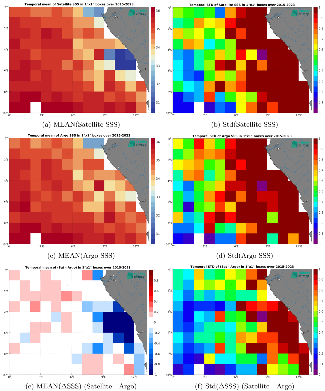
Figure 6: Temporal mean (left) and Std (right) of SSS from SMAP SSS L3 v5.0 - Monthly (JPL) (top), Argo (middle), and of \Delta SSS (Satellite - Argo). Only match-up pairs are used to generate these maps.
