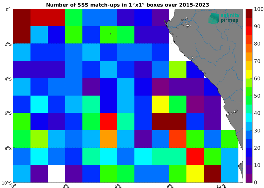
Figure 4: Number of SSS match-ups between Argo SSS and the SMAP SSS L3 v5.0 - Monthly (JPL) SSS product for the Congo river plume Pi-MEP region over 1^\circ \times 1^\circ boxes and for the full satellite product period.
