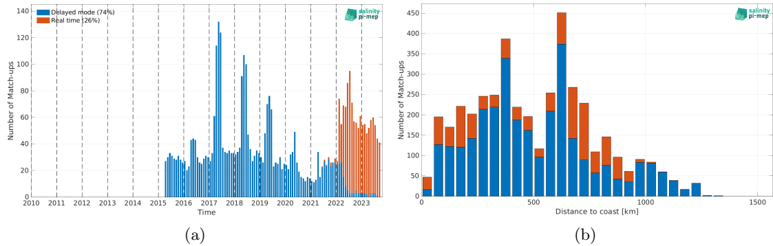
Figure 1: Number of match-ups between Argo and SMAP SSS L3 v5.0 - Monthly (JPL) SSS as a function of time (a) and as function of the distance to coast (b) over the Congo river plume Pi-MEP region and for the full satellite product period.
