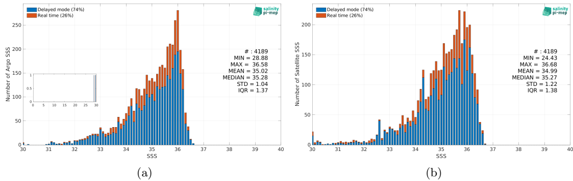
Figure 2: Histograms of SSS from Argo (a) and SMAP SSS L3 v5.0 - Monthly (JPL) (b) considering all match-up pairs per bins of 0.1 over the Congo river plume Pi-MEP region and for the full satellite product period.
