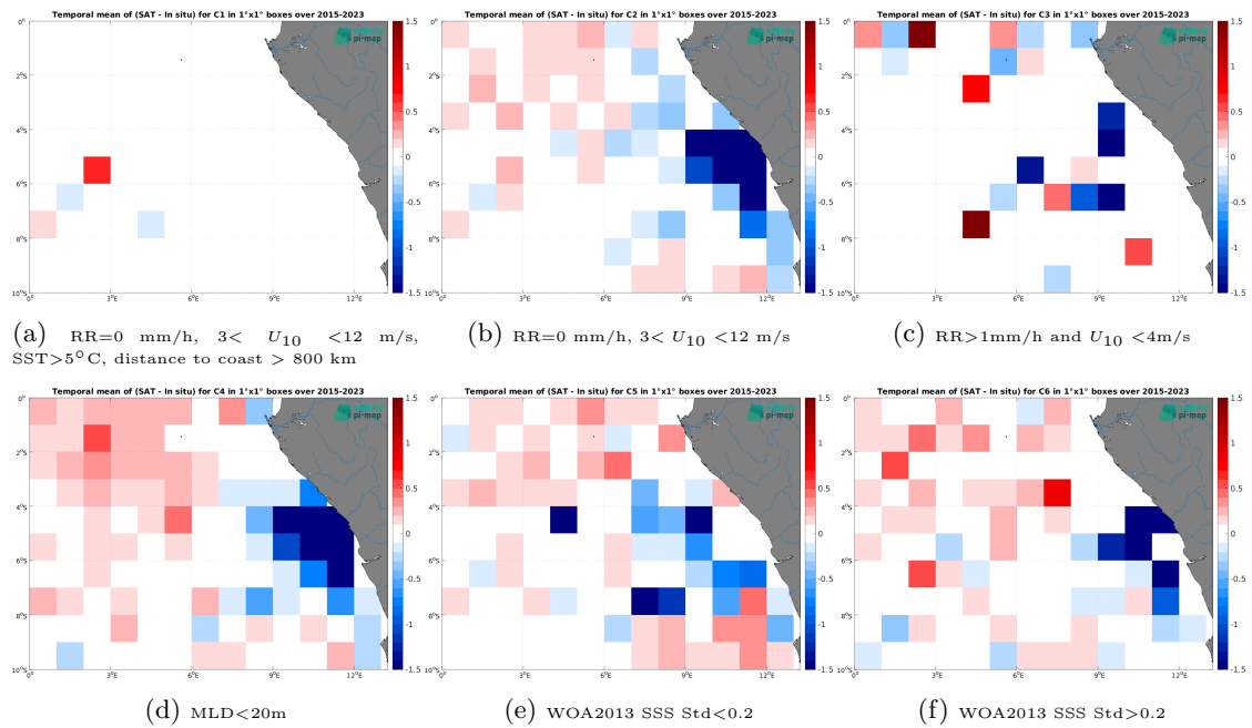
Figure 12: Temporal mean gridded over spatial boxes of size 1^\circ \times 1^\circ of \Delta SSS (SMAP SSS L3 v5.0 - Monthly (JPL) - Argo) for 6 different subdatasets corresponding to: RR=0 mm/h, 3 < U_{10} < 12 m/s, SST > 5°C, distance to coast > 800 km (a), RR=0 mm/h, 3 < U_{10} < 12 m/s (b), RR > 1 mm/h and U_{10} < 4 m/s (c), MLD < 20m (d), WOA2013 SSS Std < 0.2 (e), WOA2013 SSS Std > 0.2 (f).
