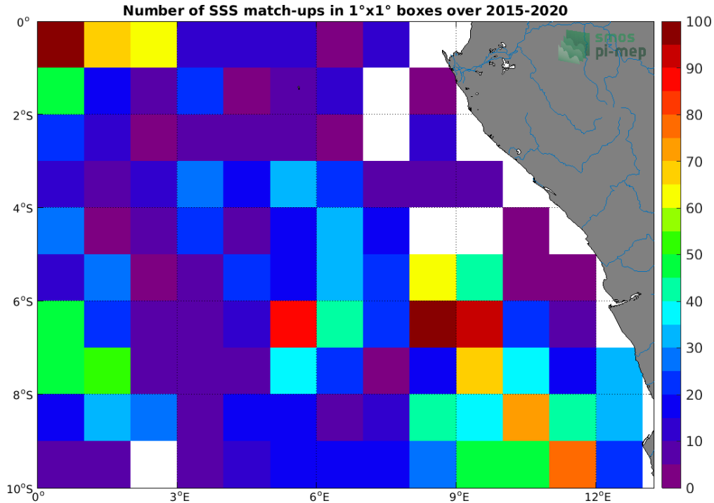
Figure 4: Number of SSS match-ups between Argo SSS and the SMAP SSS L3 v5.0 - Monthly (JPL) SSS product for the Congo river plume Pi-MEP region over 1°x1° boxes and for the full satellite product period.
