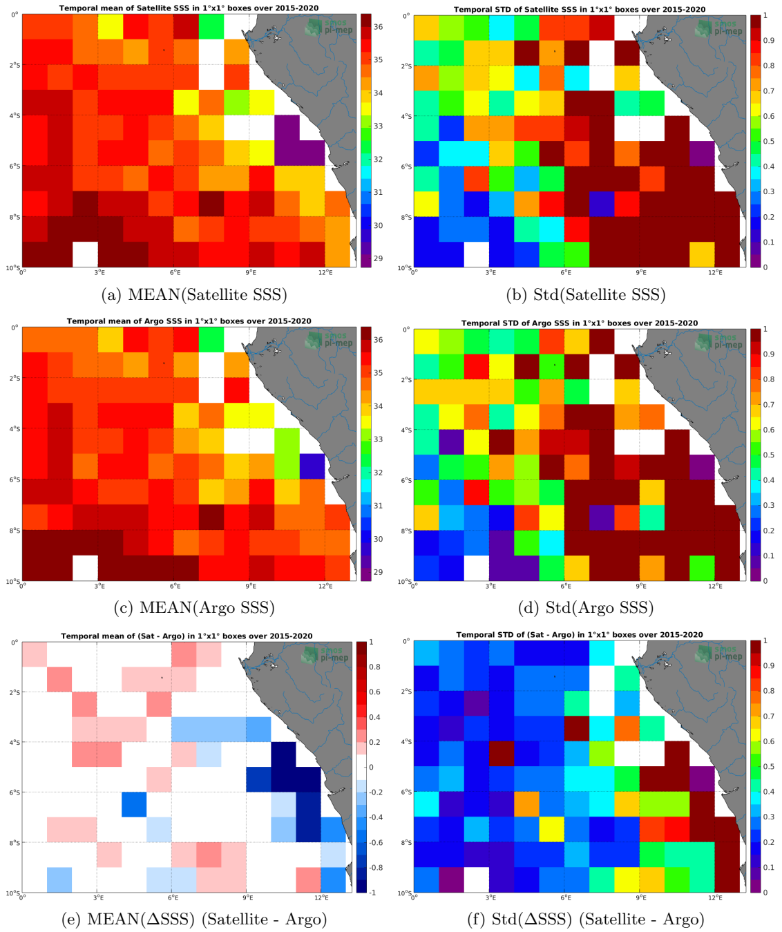
Figure 6: Temporal mean (left) and Std (right) of SSS from SMAP-L3-JPL-V4.3-8DAY-RUNNING-60KM (top), Argo (middle), and of \Delta SSS (Satellite - Argo). Only match-up pairs are used to generate these maps.
