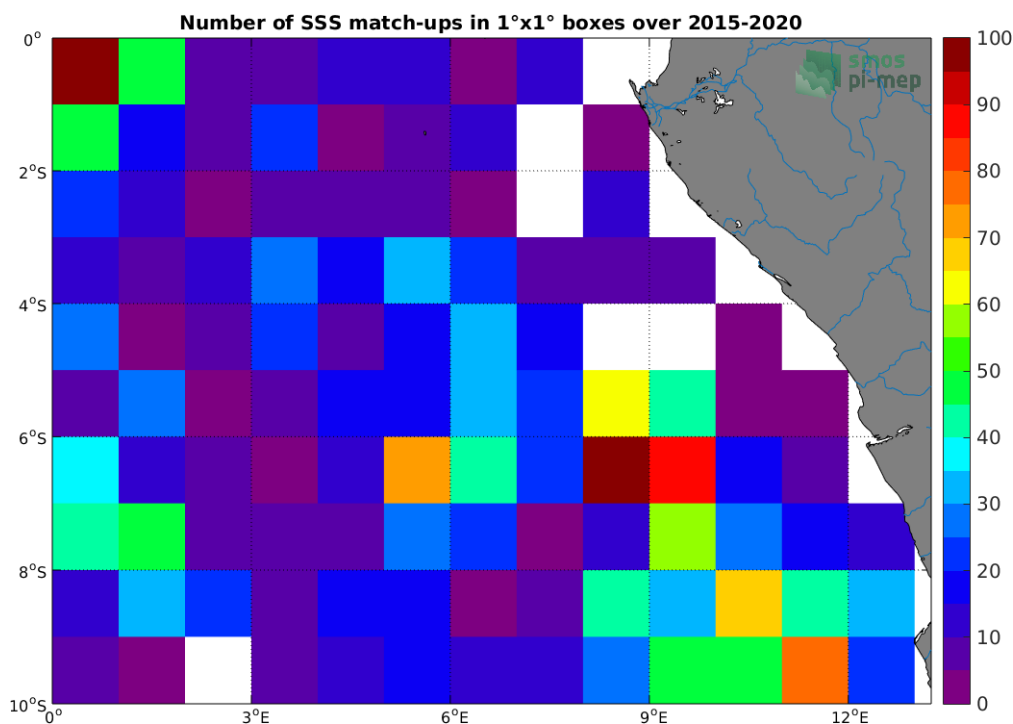
Figure 4: Number of SSS match-ups between Argo SSS and the SMAP-L3-JPL-V4.3-8DAY-RUNNING-60KM SSS product for the Congo river plume Pi-MEP region over 1^\circ \times 1^\circ boxes and for the full satellite product period.
