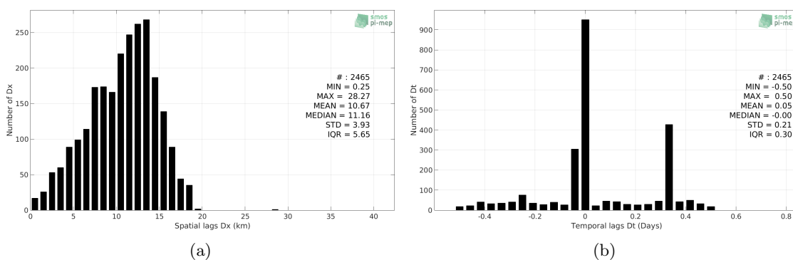
Figure 5: Histograms of the spatial (a) and temporal (b) lags between the time of the Argo measurements and the date of the corresponding SMAP-L3-JPL-V4.3-8DAY-RUNNING-60KM SSS product.
