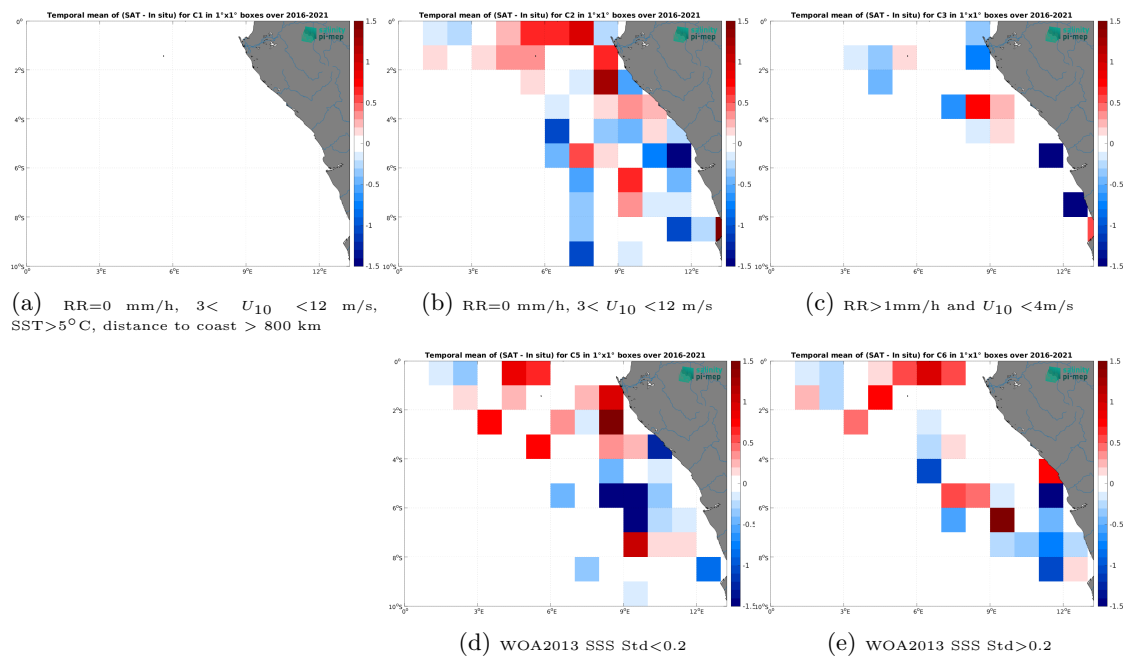
Figure 14: Temporal mean gridded over spatial boxes of size 1^\circ \times 1^\circ of \Delta SSS (SMAP SSS L2 v5.3 - 40 km (RSS) - TSG (LEGOS-DM)) for 5 different subdatasets corresponding to:RR=0 mm/h, 3 < U_{10} < 12 m/s, SST>5°C, distance to coast > 800 km (a), RR=0 mm/h, 3 < U_{10} < 12 m/s (b), RR>1mm/h and U_{10} < 4 m/s (c), WOA2013 SSS Std<0.2 (d), WOA2013 SSS Std>0.2 (e).
