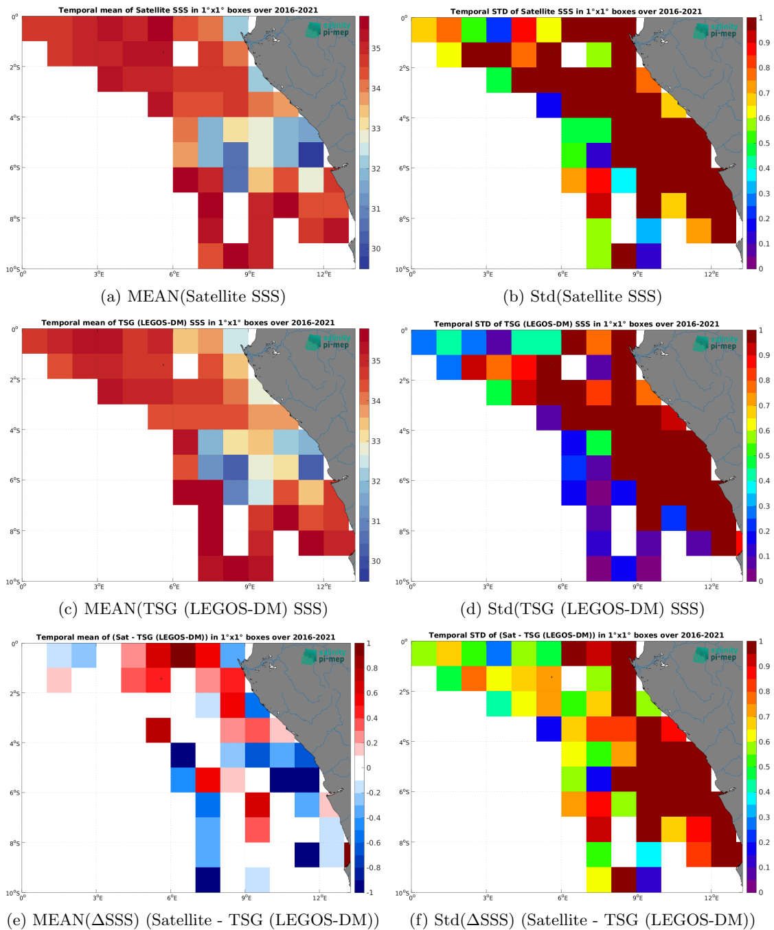
Figure 7: Temporal mean (left) and Std (right) of SSS from SMAP SSS L2 v5.3 - 40 km (RSS) (top), TSG (LEGOS-DM) (middle), and of \Delta SSS (Satellite - TSG (LEGOS-DM)). Only match-up pairs are used to generate these maps.
