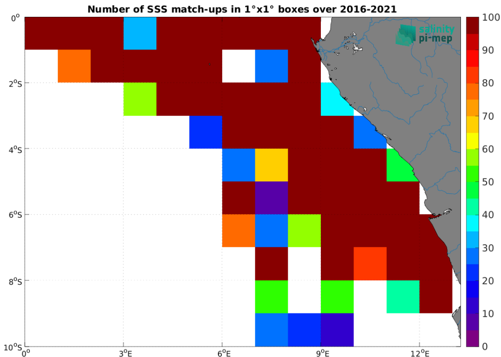
Figure 5: Number of SSS match-ups between TSG (LEGOS-DM) SSS and the SMAP SSS L2 v5.3 - 40 km (RSS) SSS product for the Congo river plume Pi-MEP region over 1^\circ \times 1^\circ boxes and for the full satellite product period.
