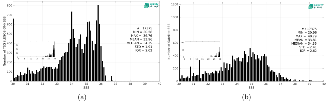
Figure 3: Histograms of SSS from TSG (LEGOS-DM) (a) and SMAP SSS L2 v5.3 - 40 km (RSS) (b) considering all match-up pairs per bins of 0.1 over the Congo river plume Pi-MEP region and for the full satellite product period.
