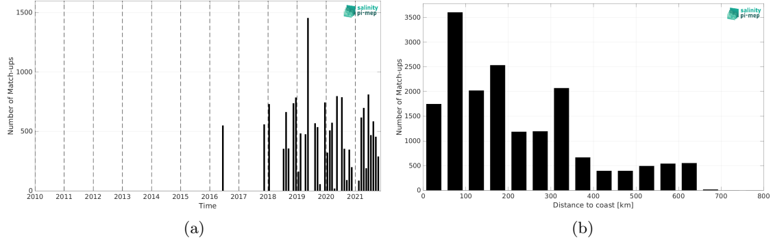
Figure 2: Number of match-ups between TSG (LEGOS-DM) and SMAP SSS L2 v5.3 - 40 km (RSS) SSS as a function of time (a) and as function of the distance to coast (b) over the Congo river plume Pi-MEP region and for the full satellite product period.
