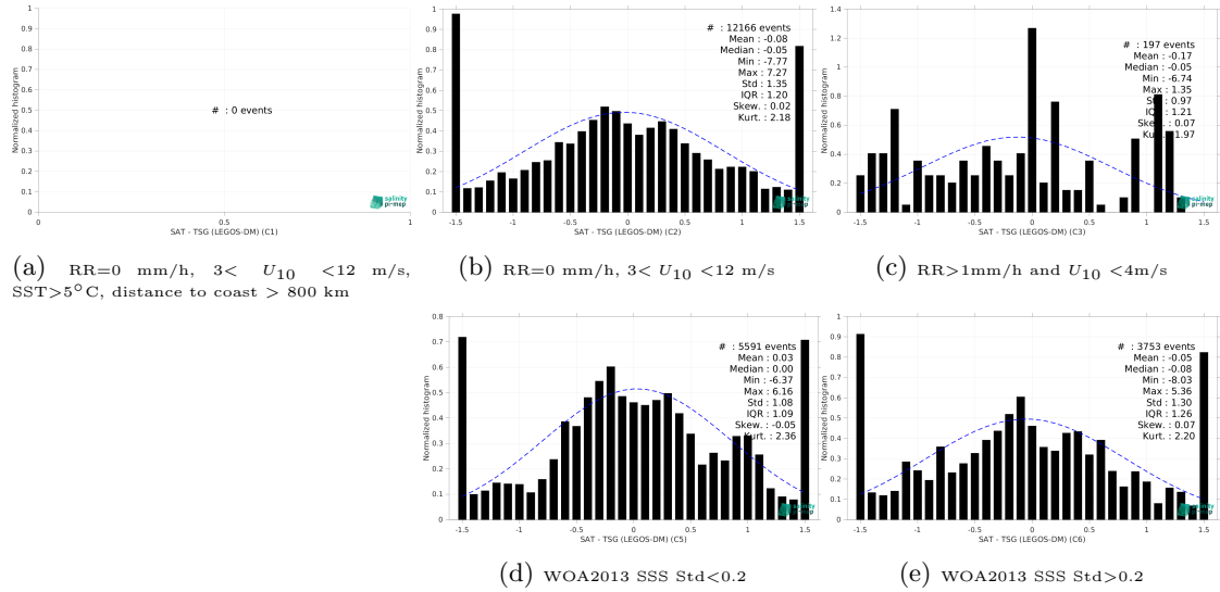
Figure 15: Normalized histogram of \Delta SSS (SMAP SSS L2 v5.3 - 40 km (RSS) - TSG (LEGOS-DM)) for 5 different subdatasets corresponding to: RR=0 mm/h, 3 < U_{10} < 12 m/s, SST > 5°C, distance to coast > 800 km (a), RR=0 mm/h, 3 < U_{10} < 12 m/s (b), RR > 1mm/h and U_{10} < 4 m/s (c), WOA2013 SSS Std < 0.2 (d), WOA2013 SSS Std > 0.2 (e).
