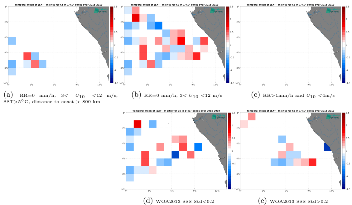
Figure 14: Temporal mean gridded over spatial boxes of size 1^\circ \times 1^\circ of \Delta SSS (SMAP SSS L2 v5.3 - 40 km (RSS) - TSG (GOSUD-Research-vessel)) for 5 different subdatasets corresponding to:RR=0 mm/h, 3 < U_{10} < 12 m/s, SST>5°C, distance to coast > 800 km (a), RR=0 mm/h, 3 < U_{10} < 12 m/s (b), RR>1mm/h and U_{10} < 4 m/s (c), WOA2013 SSS Std<0.2 (d), WOA2013 SSS Std>0.2 (e).
