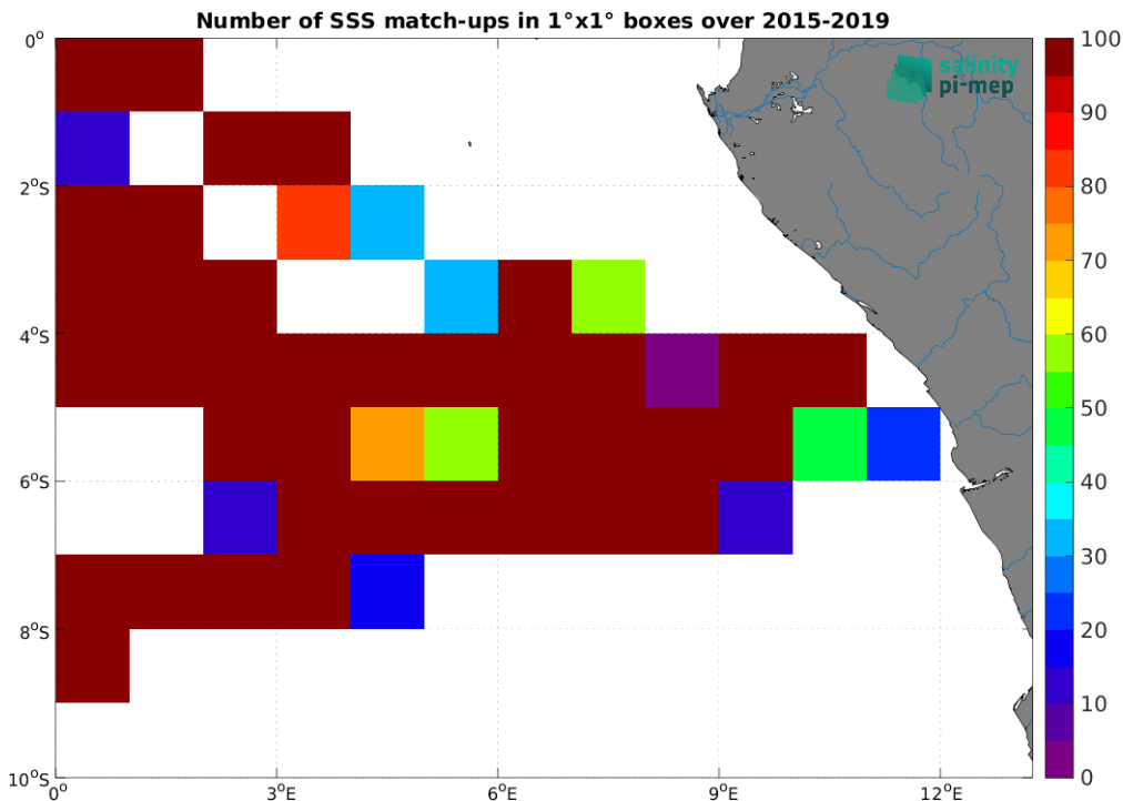
Figure 5: Number of SSS match-ups between TSG (GOSUD-Research-vessel) SSS and the SMAP SSS L2 v5.3 - 40 km (RSS) SSS product for the Congo river plume Pi-MEP region over 1^\circ \times 1^\circ boxes and for the full satellite product period.
