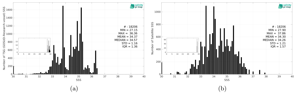
Figure 3: Histograms of SSS from TSG (GOSUD-Research-vessel) (a) and SMAP SSS L2 v5.3 - 40 km (RSS) (b) considering all match-up pairs per bins of 0.1 over the Congo river plume Pi-MEP region and for the full satellite product period.
