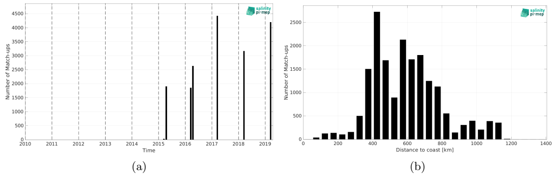
Figure 2: Number of match-ups between TSG (GOSUD-Research-vessel) and SMAP SSS L2 v5.3 - 40 km (RSS) SSS as a function of time (a) and as function of the distance to coast (b) over the Congo river plume Pi-MEP region and for the full satellite product period.
