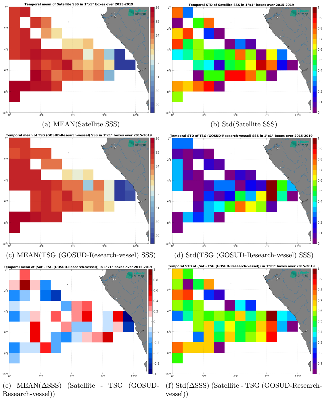
Figure 7: Temporal mean (left) and Std (right) of SSS from SMAP SSS L2 v5.3 - 40 km (RSS) (top), TSG (GOSUD-Research-vessel) (middle), and of \Delta SSS (Satellite - TSG (GOSUD-Research-vessel)). Only match-up pairs are used to generate these maps.
