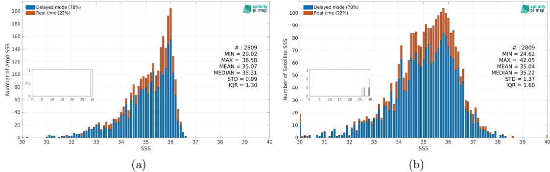
Figure 3: Histograms of SSS from Argo (a) and SMAP SSS L2 v5.3 - 40 km (RSS) (b) considering all match-up pairs per bins of 0.1 over the Congo river plume Pi-MEP region and for the full satellite product period.
