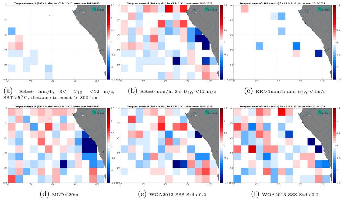
Figure 14: Temporal mean gridded over spatial boxes of size 1^\circ \times 1^\circ of \Delta SSS (SMAP SSS L2 v5.3 - 40 km (RSS) - Argo) for 6 different subdatasets corresponding to:RR=0 mm/h, 3 < U_{10} < 12 m/s, SST>5°C, distance to coast > 800 km (a), RR=0 mm/h, 3 < U_{10} < 12 m/s (b), RR>1mm/h and U_{10} < 4 m/s (c),MLD<20m (d),WOA2013 SSS Std<0.2 (e),WOA2013 SSS Std>0.2 (f).
