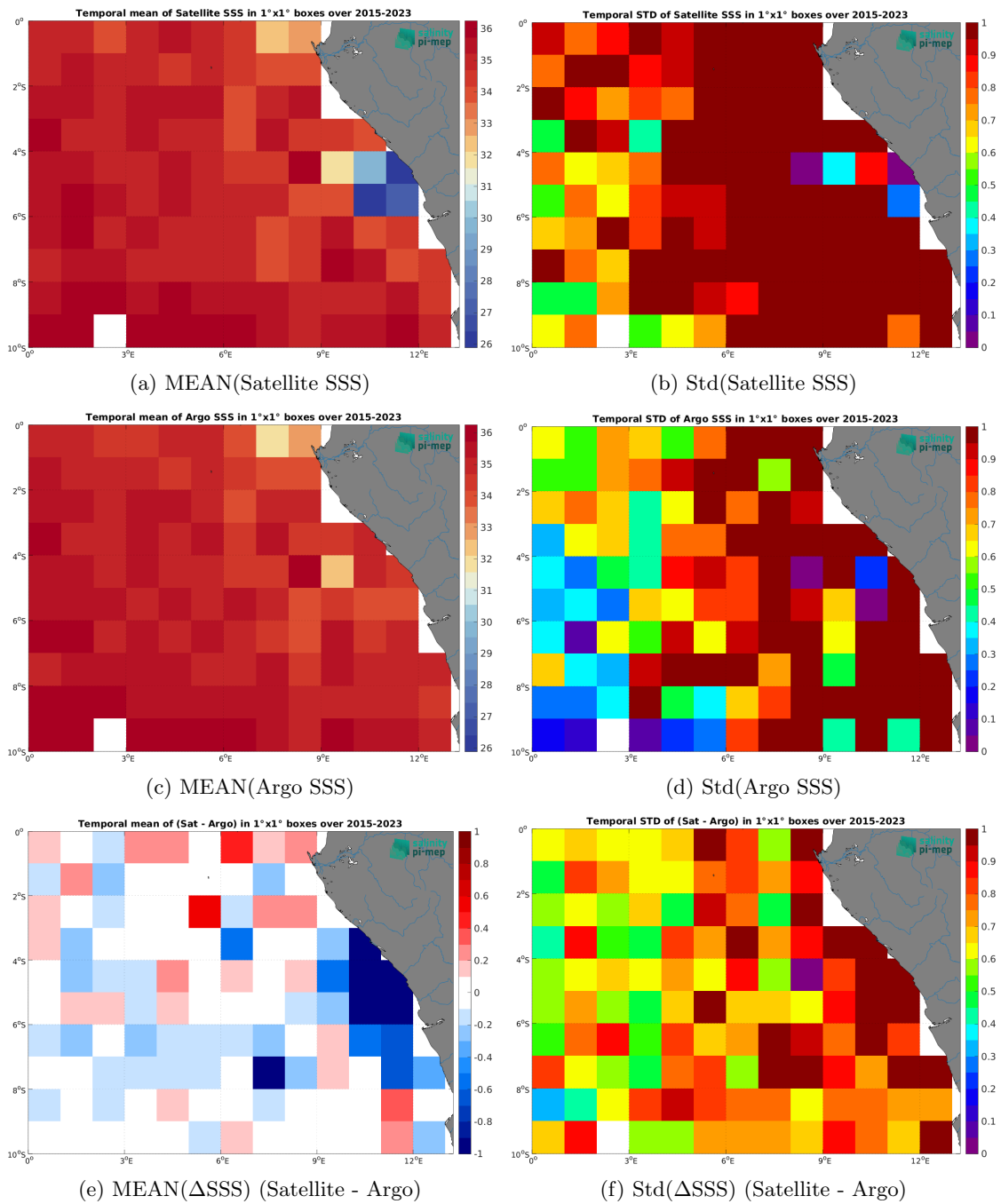
Figure 7: Temporal mean (left) and Std (right) of SSS from SMAP SSS L2 v5.3 - 40 km (RSS) (top), Argo (middle), and of \Delta SSS (Satellite - Argo). Only match-up pairs are used to generate these maps.
