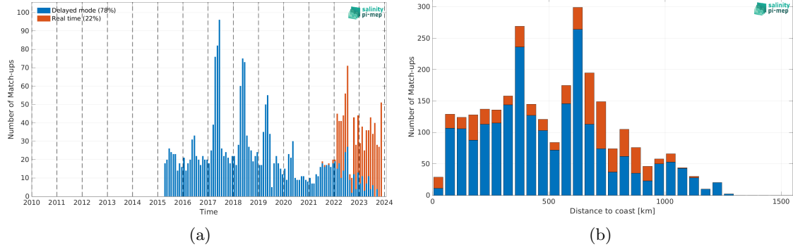
Figure 2: Number of match-ups between Argo and SMAP SSS L2 v5.3 - 40 km (RSS) SSS as a function of time (a) and as function of the distance to coast (b) over the Congo river plume Pi-MEP region and for the full satellite product period.
