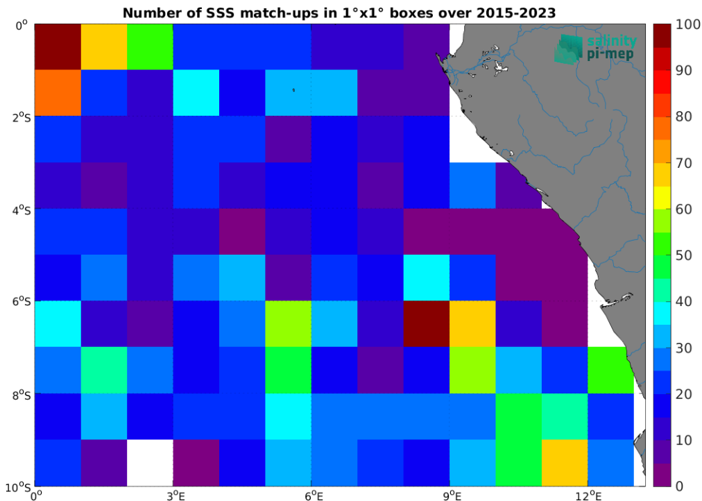
Figure 5: Number of SSS match-ups between Argo SSS and the SMAP SSS L2 v5.3 - 40 km (RSS) SSS product for the Congo river plume Pi-MEP region over 1^\circ \times 1^\circ boxes and for the full satellite product period.
