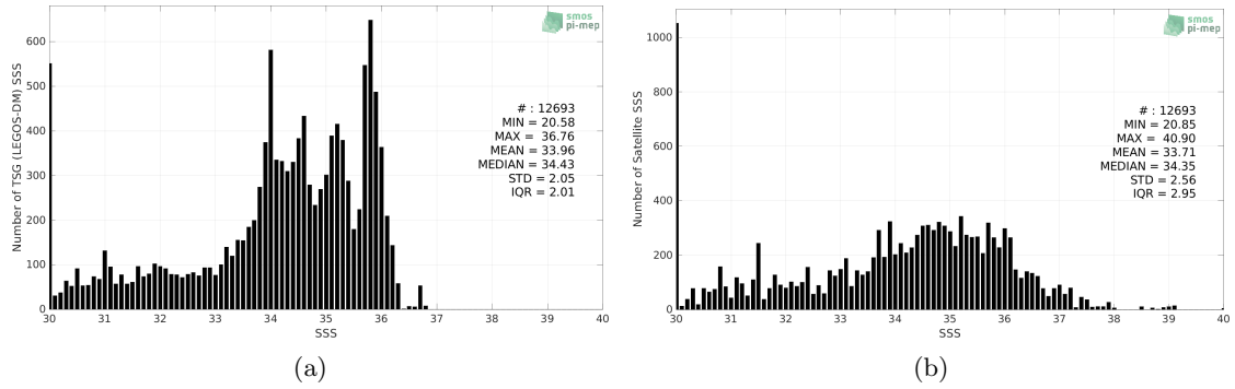
Figure 2: Histograms of SSS from TSG (LEGOS-DM) (a) and SMAP SSS L2 v5 - 40 km (RSS) (b) considering all match-up pairs per bins of 0.1 over the Congo river plume Pi-MEP region and for the full satellite product period.
