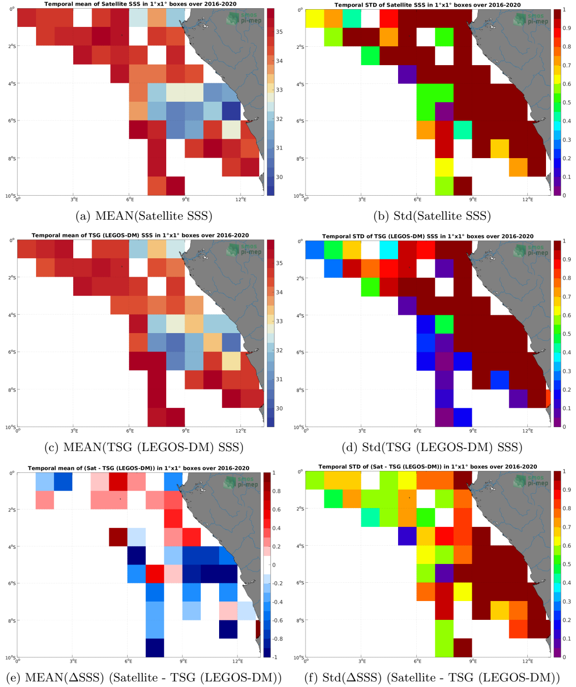
Figure 6: Temporal mean (left) and Std (right) of SSS from SMAP SSS L2 v5 - 40 km (RSS) (top), TSG (LEGOS-DM) (middle), and of \Delta SSS (Satellite - TSG (LEGOS-DM)). Only match-up pairs are used to generate these maps.
