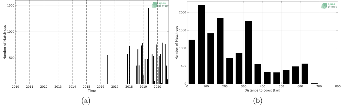
Figure 1: Number of match-ups between TSG (LEGOS-DM) and SMAP SSS L2 v5 - 40 km (RSS) SSS as a function of time (a) and as function of the distance to coast (b) over the Congo river plume Pi-MEP region and for the full satellite product period.
