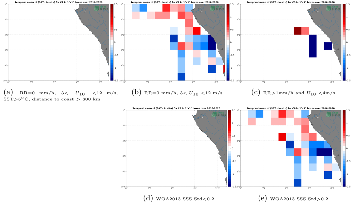
Figure 12: Temporal mean gridded over spatial boxes of size 1^\circ \times 1^\circ of \Delta SSS (SMAP SSS L2 v5 - 40 km (RSS) - TSG (LEGOS-DM)) for 5 different subdatasets corresponding to:RR=0 mm/h, 3 < U_{10} < 12 m/s, SST >5^\circ\text{C} , distance to coast > 800 km (a), RR=0 mm/h, 3 < U_{10} < 12 m/s (b), RR >1 mm/h and U_{10} < 4 m/s (c), WOA2013 SSS Std <0.2 (d), WOA2013 SSS Std >0.2 (e).
