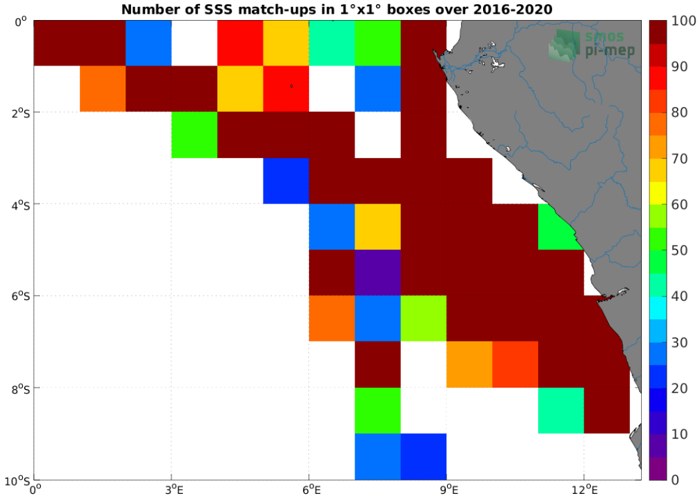
Figure 4: Number of SSS match-ups between TSG (LEGOS-DM) SSS and the SMAP SSS L2 v5 - 40 km (RSS) SSS product for the Congo river plume Pi-MEP region over 1^\circ \times 1^\circ boxes and for the full satellite product period.
