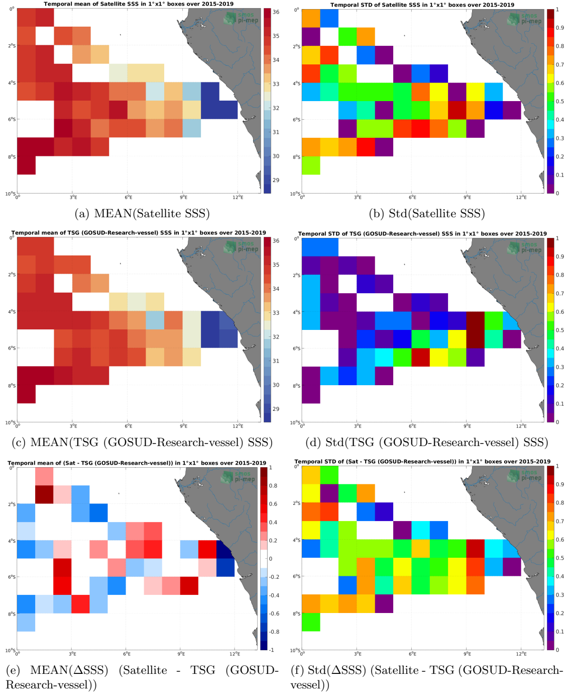
Figure 6: Temporal mean (left) and Std (right) of SSS from SMAP SSS L2 v5 - 40 km (RSS) (top), TSG (GOSUD-Research-vessel) (middle), and of \Delta SSS (Satellite - TSG (GOSUD-Research-vessel)). Only match-up pairs are used to generate these maps.
