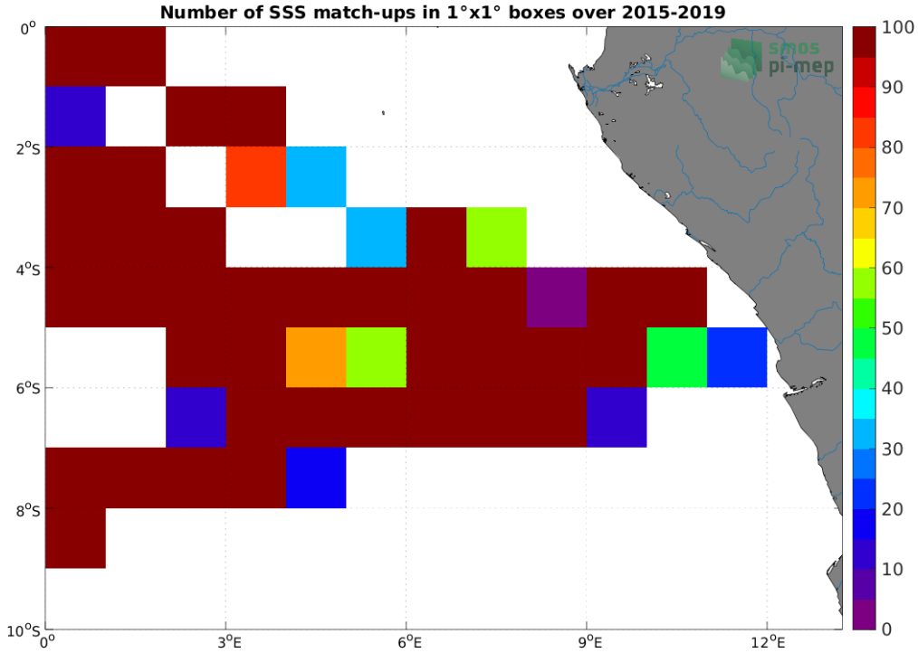
Figure 4: Number of SSS match-ups between TSG (GOSUD-Research-vessel) SSS and the SMAP SSS L2 v5 - 40 km (RSS) SSS product for the Congo river plume Pi-MEP region over 1^\circ \times 1^\circ boxes and for the full satellite product period.
