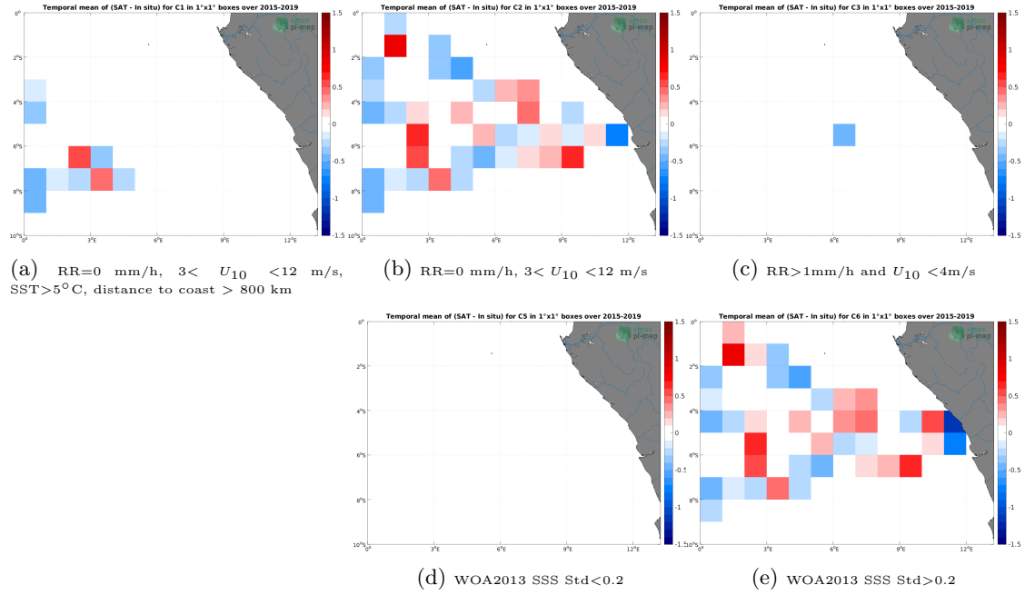
Figure 12: Temporal mean gridded over spatial boxes of size 1^\circ \times 1^\circ of \Delta SSS (SMAP SSS L2 v5 - 40 km (RSS) - TSG (GOSUD-Research-vessel)) for 5 different subdatasets corresponding to: RR=0 mm/h, 3 < U_{10} < 12 m/s, SST > 5^\circ C , distance to coast > 800 km (a), RR=0 mm/h, 3 < U_{10} < 12 m/s (b), RR > 1 mm/h and U_{10} < 4 m/s (c), WOA2013 SSS Std < 0.2 (d), WOA2013 SSS Std > 0.2 (e).
