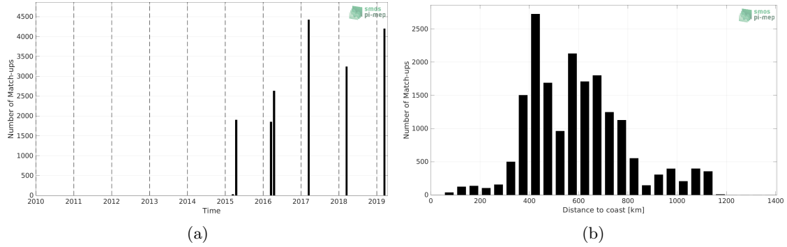
Figure 1: Number of match-ups between TSG (GOSUD-Research-vessel) and SMAP SSS L2 v5 - 40 km (RSS) SSS as a function of time (a) and as function of the distance to coast (b) over the Congo river plume Pi-MEP region and for the full satellite product period.
