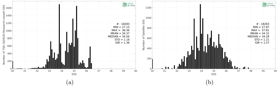
Figure 2: Histograms of SSS from TSG (GOSUD-Research-vessel) (a) and SMAP SSS L2 v5 - 40 km (RSS) (b) considering all match-up pairs per bins of 0.1 over the Congo river plume Pi-MEP region and for the full satellite product period.
