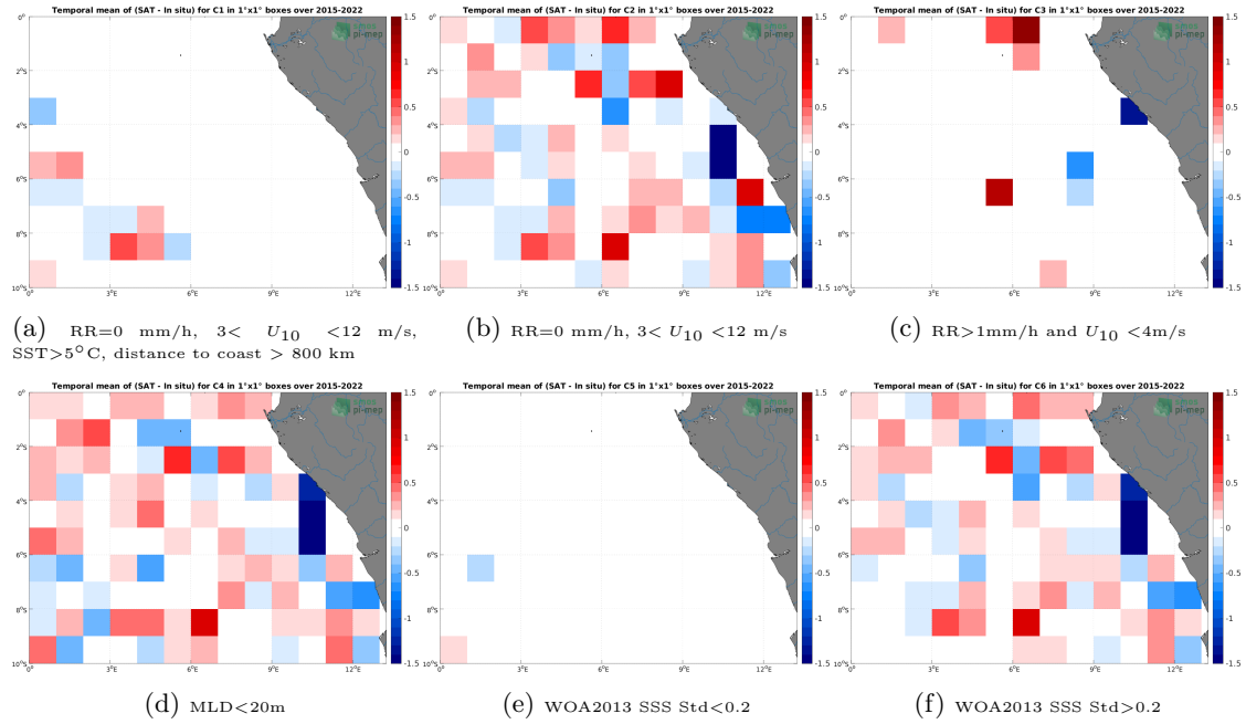
Figure 12: Temporal mean gridded over spatial boxes of size 1^\circ \times 1^\circ of \Delta SSS (SMAP SSS L2 v5 - 40 km (RSS) - Argo) for 6 different subdatasets corresponding to: RR=0 mm/h, 3 < U_{10} < 12 m/s, SST >5^\circ\text{C} , distance to coast > 800 km (a), RR=0 mm/h, 3 < U_{10} < 12 m/s (b), RR >1 mm/h and U_{10} < 4 m/s (c),MLD <20 m (d),WOA2013 SSS Std <0.2 (e),WOA2013 SSS Std >0.2 (f).
