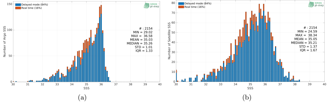
Figure 2: Histograms of SSS from Argo (a) and SMAP SSS L2 v5 - 40 km (RSS) (b) considering all match-up pairs per bins of 0.1 over the Congo river plume Pi-MEP region and for the full satellite product period.
