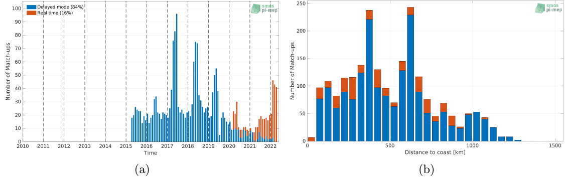
Figure 1: Number of match-ups between Argo and SMAP SSS L2 v5 - 40 km (RSS) SSS as a function of time (a) and as function of the distance to coast (b) over the Congo river plume Pi-MEP region and for the full satellite product period.
