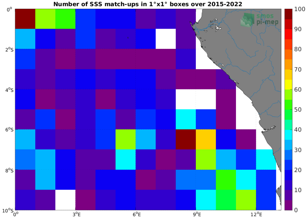
Figure 4: Number of SSS match-ups between Argo SSS and the SMAP SSS L2 v5 - 40 km (RSS) SSS product for the Congo river plume Pi-MEP region over 1^\circ \times 1^\circ boxes and for the full satellite product period.
