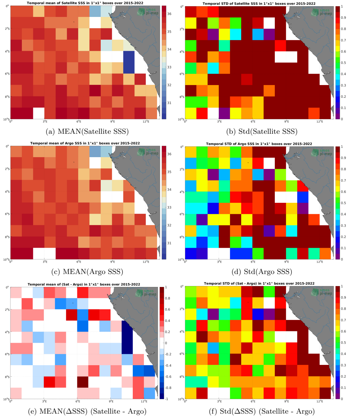
Figure 6: Temporal mean (left) and Std (right) of SSS from SMAP SSS L2 v5 - 40 km (RSS) (top), Argo (middle), and of \Delta SSS (Satellite - Argo). Only match-up pairs are used to generate these maps.
