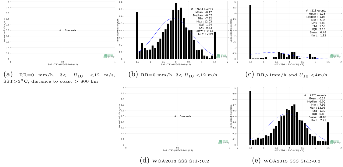
Figure 13: Normalized histogram of \Delta\text{SSS} (SMAP SSS L2 v4 (RSS) - TSG (LEGOS-DM)) for 5 different subdatasets corresponding to: RR=0 mm/h, 3 < U_{10} < 12 m/s, SST > 5^\circ\text{C} , distance to coast > 800 km (a), RR=0 mm/h, 3 < U_{10} < 12 m/s (b), RR > 1\text{mm/h} and U_{10} < 4\text{m/s} (c), WOA2013 SSS Std < 0.2 (d), WOA2013 SSS Std > 0.2 (e).
