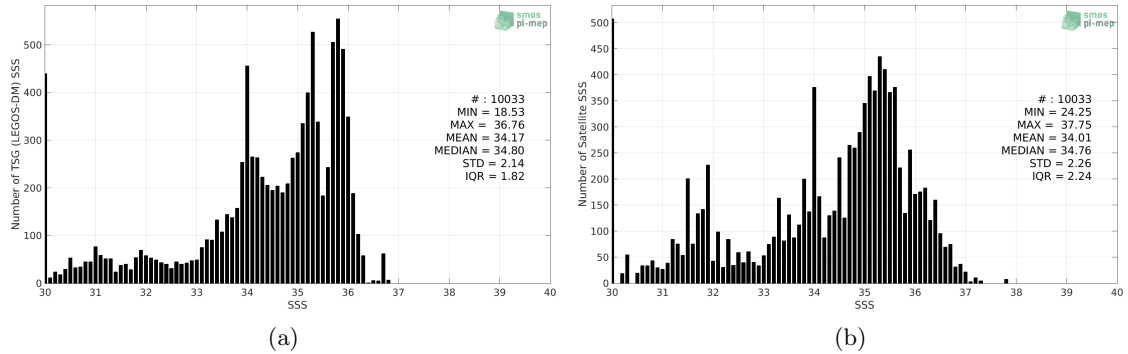
Figure 2: Histograms of SSS from TSG (LEGOS-DM) (a) and SMAP SSS L2 v4 (RSS) (b) considering all match-up pairs per bins of 0.1 over the Congo river plume Pi-MEP region and for the full satellite product period.
