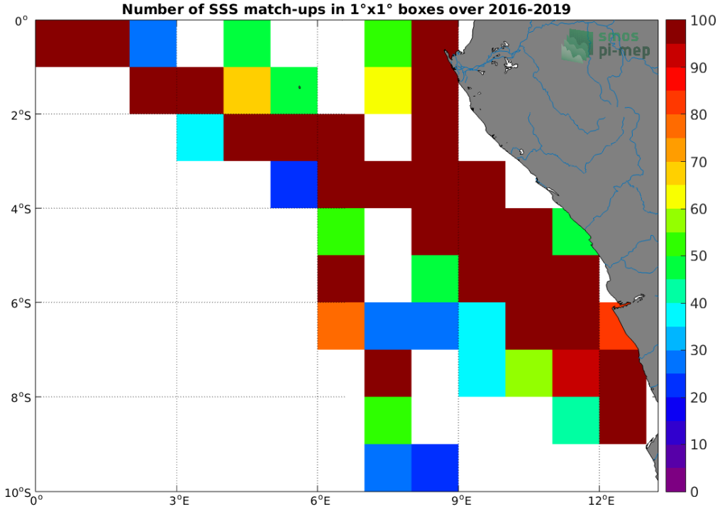
Figure 4: Number of SSS match-ups between TSG (LEGOS-DM) SSS and the SMAP SSS L2 v4 (RSS) SSS product for the Congo river plume Pi-MEP region over 1^\circ \times 1^\circ boxes and for the full satellite product period.
