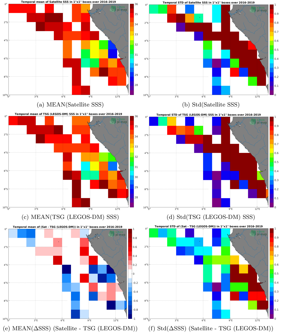
Figure 6: Temporal mean (left) and Std (right) of SSS from SMAP SSS L2 v4 (RSS) (top), TSG (LEGOS-DM) (middle), and of \Delta SSS (Satellite - TSG (LEGOS-DM)). Only match-up pairs are used to generate these maps.
