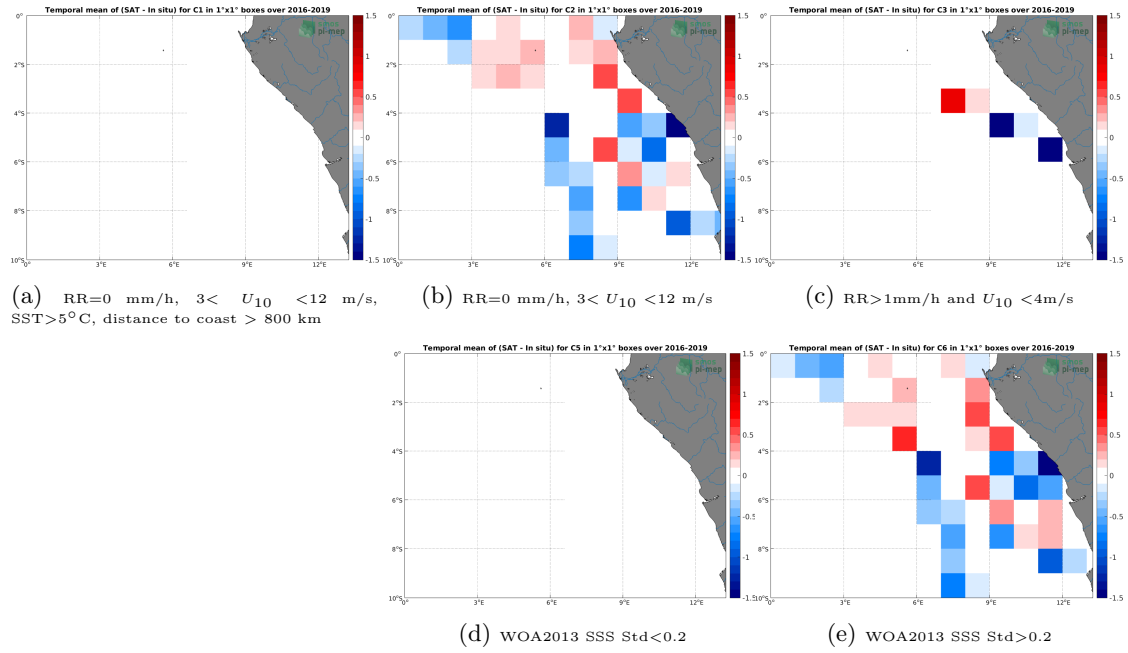
Figure 12: Temporal mean gridded over spatial boxes of size 1^\circ \times 1^\circ of \Delta SSS (SMAP SSS L2 v4 (RSS) - TSG (LEGOS-DM)) for 5 different subdatasets corresponding to: RR=0 mm/h, 3 < U_{10} < 12 m/s, SST > 5^\circ C , distance to coast > 800 km (a), RR=0 mm/h, 3 < U_{10} < 12 m/s (b), RR > 1 mm/h and U_{10} < 4 m/s (c), WOA2013 SSS Std < 0.2 (d), WOA2013 SSS Std > 0.2 (e).
