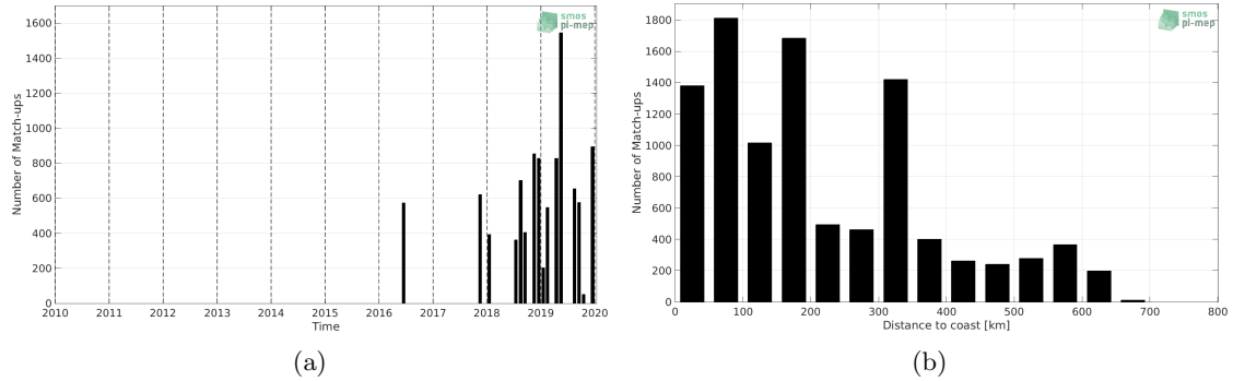
Figure 1: Number of match-ups between TSG (LEGOS-DM) and SMAP SSS L2 v4 (RSS) SSS as a function of time (a) and as function of the distance to coast (b) over the Congo river plume Pi-MEP region and for the full satellite product period.
