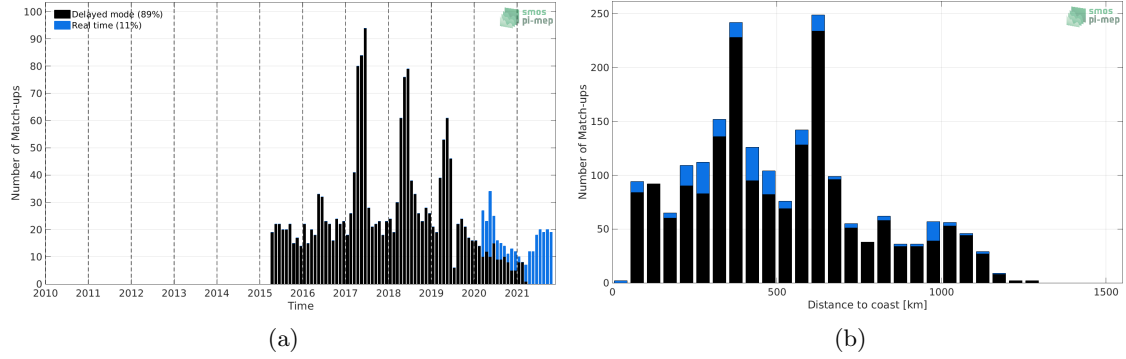
Figure 1: Number of match-ups between Argo and SMAP SSS L2 v4 (RSS) SSS as a function of time (a) and as function of the distance to coast (b) over the Congo river plume Pi-MEP region and for the full satellite product period.
