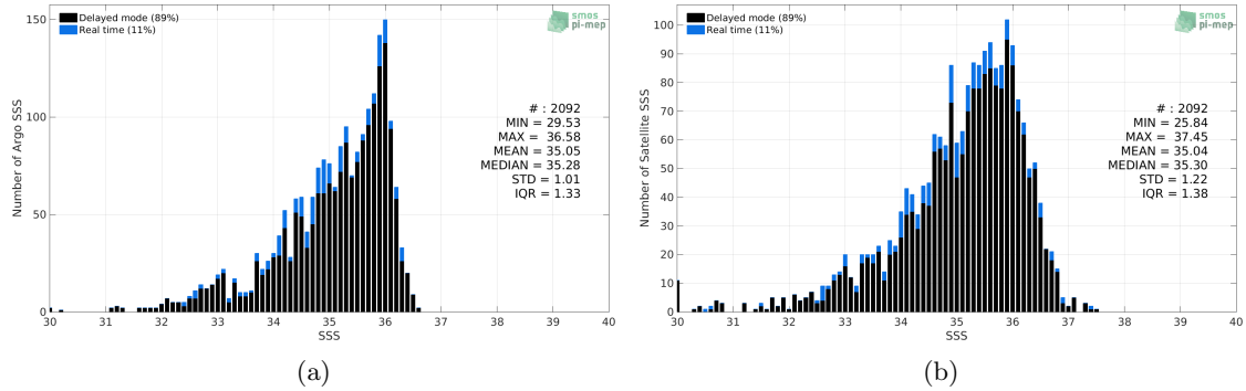
Figure 2: Histograms of SSS from Argo (a) and SMAP SSS L2 v4 (RSS) (b) considering all match-up pairs per bins of 0.1 over the Congo river plume Pi-MEP region and for the full satellite product period.
