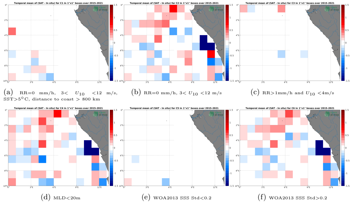
Figure 12: Temporal mean gridded over spatial boxes of size 1^\circ \times 1^\circ of \Delta SSS (SMAP SSS L2 v4 (RSS) - Argo) for 6 different subdatasets corresponding to: RR=0 mm/h, 3 < U_{10} < 12 m/s, SST > 5^\circ C , distance to coast > 800 km (a), RR=0 mm/h, 3 < U_{10} < 12 m/s (b), RR > 1 mm/h and U_{10} < 4 m/s (c), MLD < 20 m (d), WOA2013 SSS Std < 0.2 (e), WOA2013 SSS Std > 0.2 (f).
