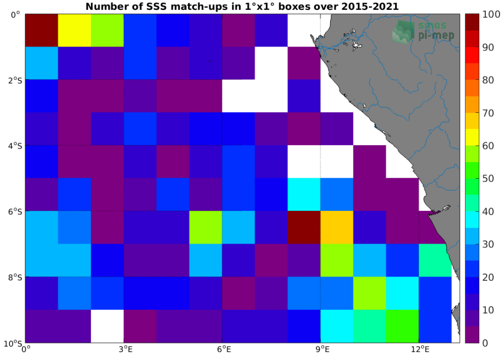
Figure 4: Number of SSS match-ups between Argo SSS and the SMAP SSS L2 v4 (RSS) SSS product for the Congo river plume Pi-MEP region over 1^\circ \times 1^\circ boxes and for the full satellite product period.
