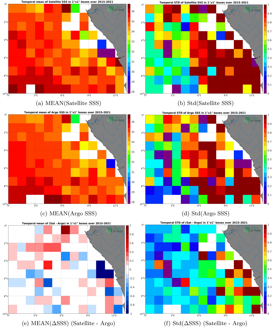
Figure 6: Temporal mean (left) and Std (right) of SSS from SMAP SSS L2 v4 (RSS) (top), Argo (middle), and of \Delta SSS (Satellite - Argo). Only match-up pairs are used to generate these maps.
