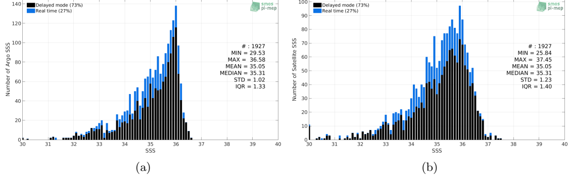
Figure 2: Histograms of SSS from Argos (a) and SMAP SSS L2 v4 (RSS) (b) considering all match-up pairs per bins of 0.1 over the Congo river plume Pi-MEP region and for the full satellite product period.
