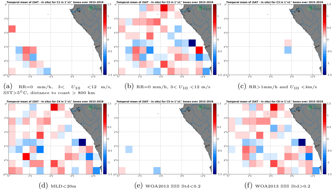
Figure 12: Temporal mean gridded over spatial boxes of size 1^\circ \times 1^\circ of \Delta SSS (SMAP-L2-RSS-V4 - Argo) for 6 different subdatasets corresponding to: RR=0 mm/h, 3 < U_{10} < 12 m/s, SST >5^\circ C, distance to coast > 800 km (a), RR=0 mm/h, 3 < U_{10} < 12 m/s (b), RR >1 mm/h and U_{10} < 4 m/s (c), MLD <20 m (d), WOA2013 SSS Std <0.2 (e), WOA2013 SSS Std >0.2 (f).
