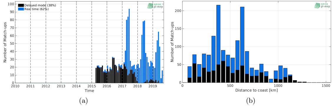
Figure 1: Number of match-ups between Argo and SMAP-L2-RSS-V4 SSS as a function of time (a) and as function of the distance to coast (b) over the Congo river plume Pi-MEP region and for the full satellite product period.
