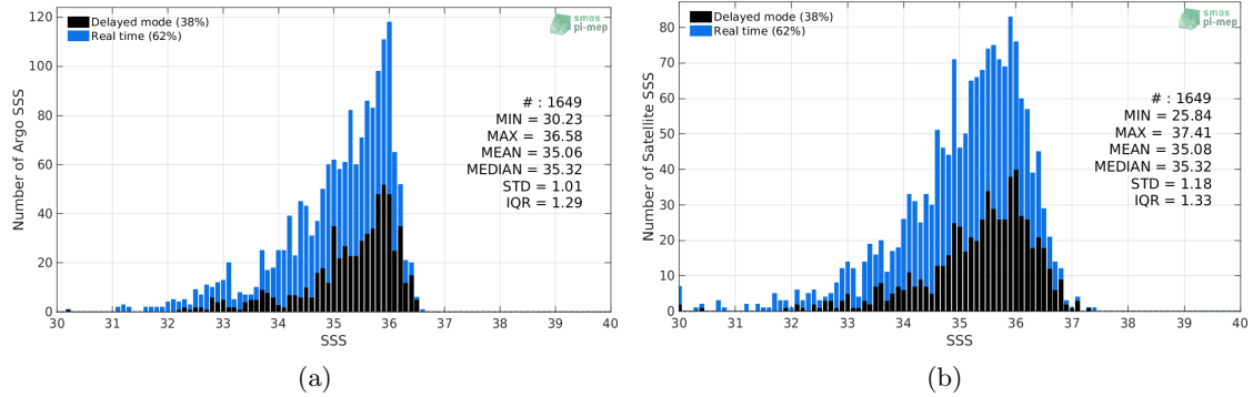
Figure 2: Histograms of SSS from Argo (a) and SMAP-L2-RSS-V4 (b) considering all match-up pairs per bins of 0.1 over the Congo river plume Pi-MEP region and for the full satellite product period.
