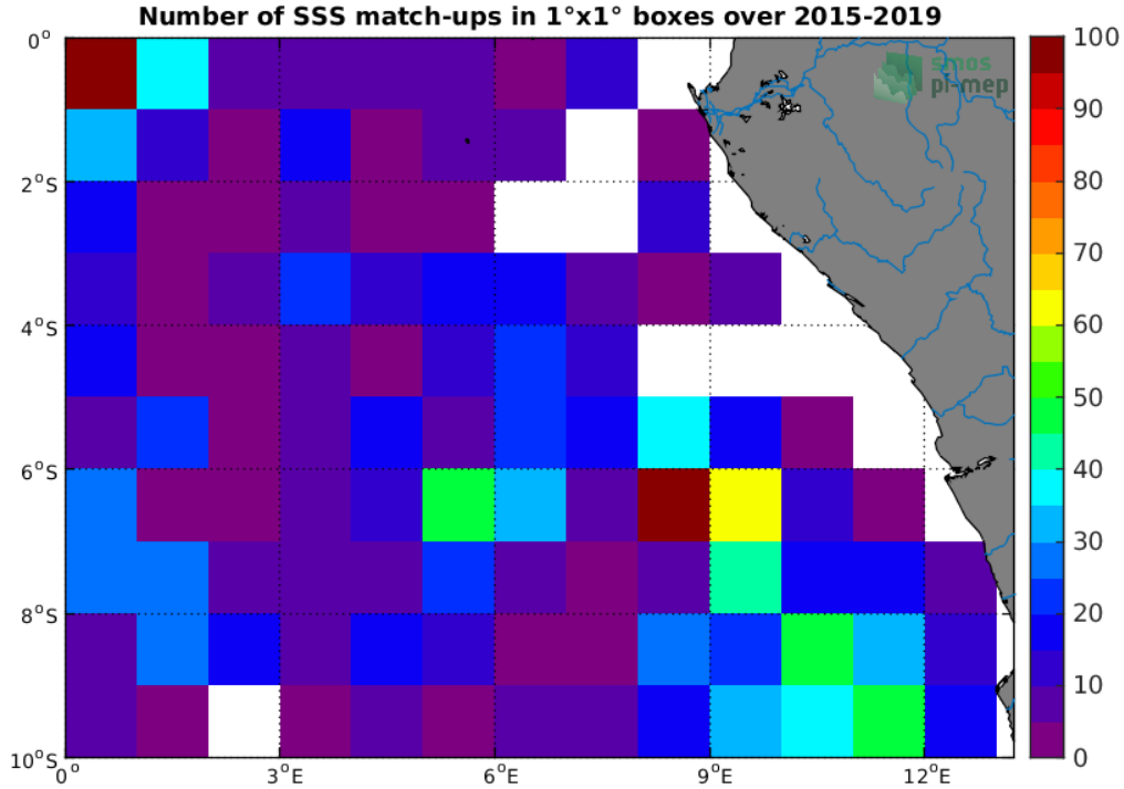
Figure 4: Number of SSS match-ups between Argo SSS and the SMAP-L2-RSS-V4 SSS product for the Congo river plume Pi-MEP region over 1^\circ \times 1^\circ boxes and for the full satellite product period.
