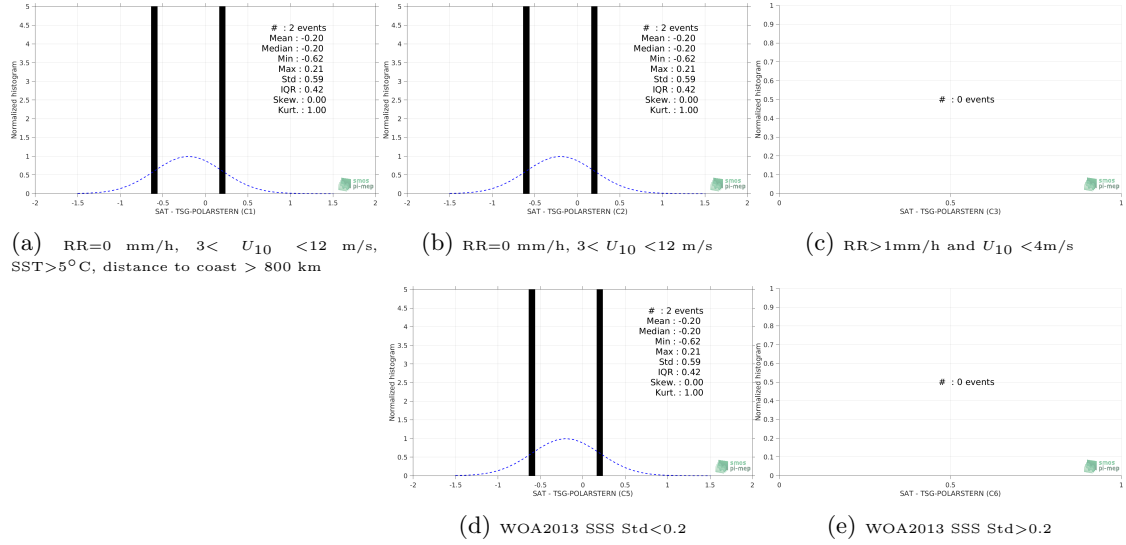
Figure 13: Normalized histogram of \Delta\text{SSS} (SMAP-L2-JPL-V4.3 - TSG-POLARSTERN) for 5 different subdatasets corresponding to: RR=0 mm/h, 3 < U_{10} < 12 m/s, SST >5^{\circ}\text{C} , distance to coast > 800 km (a), RR=0 mm/h, 3 < U_{10} < 12 m/s (b), RR >1 mm/h and U_{10} < 4 m/s (c), WOA2013 SSS Std <0.2 (d), WOA2013 SSS Std >0.2 (e).
