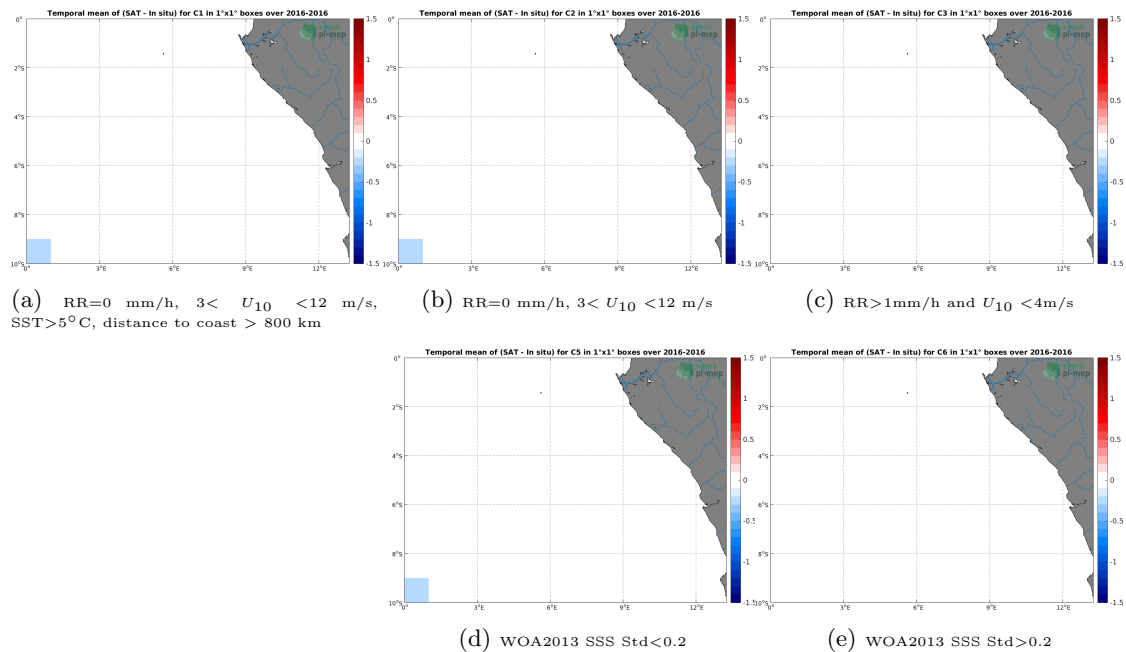
Figure 12: Temporal mean gridded over spatial boxes of size 1^{\circ}\times 1^{\circ} of \Delta\text{SSS} (SMAP-L2-JPL-V4.3 - TSG-POLARSTERN) for 5 different subdatasets corresponding to:RR=0 mm/h, 3 < U_{10} < 12 m/s, SST >5^{\circ}\text{C} , distance to coast > 800 km (a), RR=0 mm/h, 3 < U_{10} < 12 m/s (b), RR >1 mm/h and U_{10} < 4 m/s (c), WOA2013 SSS Std <0.2 (d), WOA2013 SSS Std >0.2 (e).
