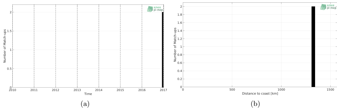
Figure 1: Number of match-ups between TSG-POLARSTERN and SMAP-L2-JPL-V4.3 SSS as a function of time (a) and as function of the distance to coast (b) over the Congo river plume Pi-MEP region and for the full satellite product period.
