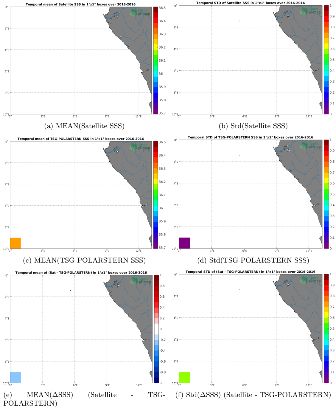
Figure 6: Temporal mean (left) and Std (right) of SSS from SMAP-L2-JPL-V4.3 (top), TSG-POLARSTERN (middle), and of \Delta SSS (Satellite - TSG-POLARSTERN). Only match-up pairs are used to generate these maps.
