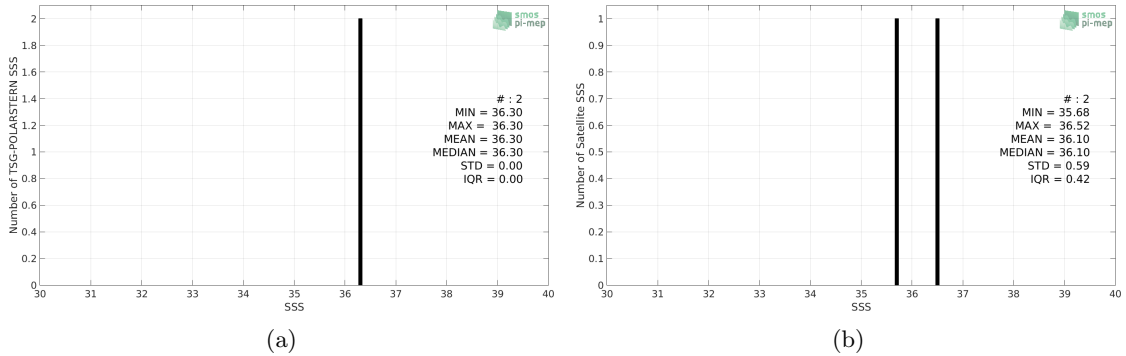
Figure 2: Histograms of SSS from TSG-POLARSTERN (a) and SMAP-L2-JPL-V4.3 (b) considering all match-up pairs per bins of 0.1 over the Congo river plume Pi-MEP region and for the full satellite product period.
