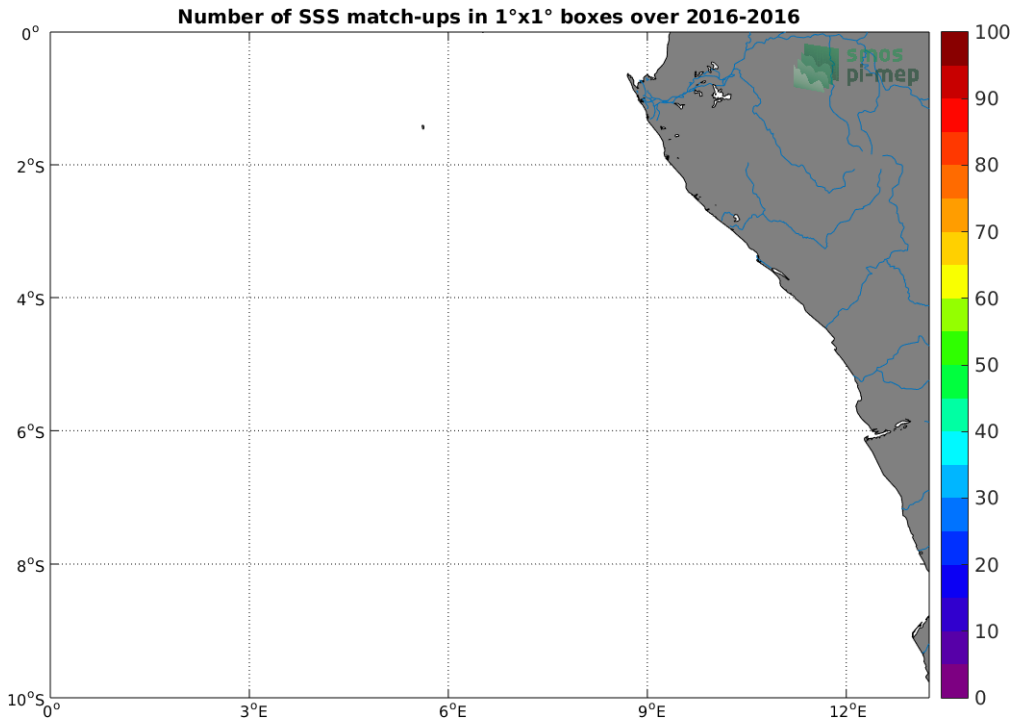
Figure 4: Number of SSS match-ups between TSG-POLARSTERN SSS and the SMAP-L2-JPL-V4.3 SSS product for the Congo river plume Pi-MEP region over 1°x1° boxes and for the full satellite product period.
