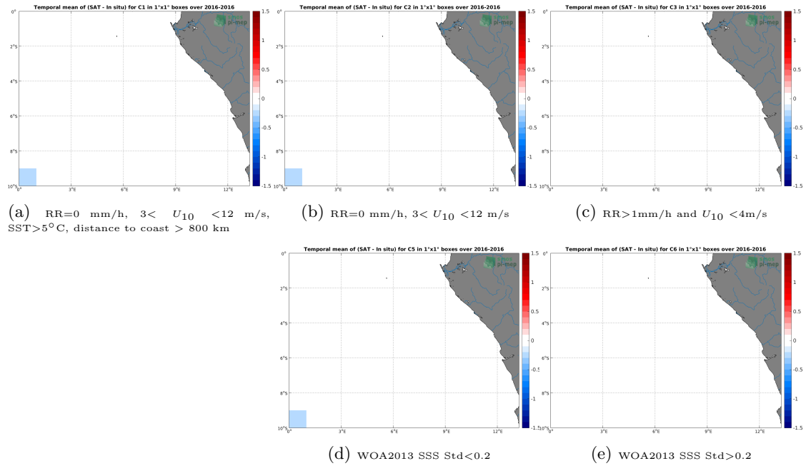
Figure 12: Temporal mean gridded over spatial boxes of size 1^\circ \times 1^\circ of \Delta SSS (SMAP-L2-JPL-V4.3 - TSG-POLARSTERN) for 5 different subdatasets corresponding to:RR=0 mm/h, 3 < U_{10} < 12 m/s, SST >5^\circ\text{C} , distance to coast > 800 km (a), RR=0 mm/h, 3 < U_{10} < 12 m/s (b), RR >1 mm/h and U_{10} < 4 m/s (c), WOA2013 SSS Std <0.2 (d), WOA2013 SSS Std >0.2 (e).
