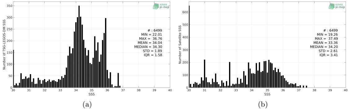
Figure 2: Histograms of SSS from TSG-LEGOS-DM (a) and SMAP-L2-JPL-V4.3 (b) considering all match-up pairs per bins of 0.1 over the Congo river plume Pi-MEP region and for the full satellite product period.
