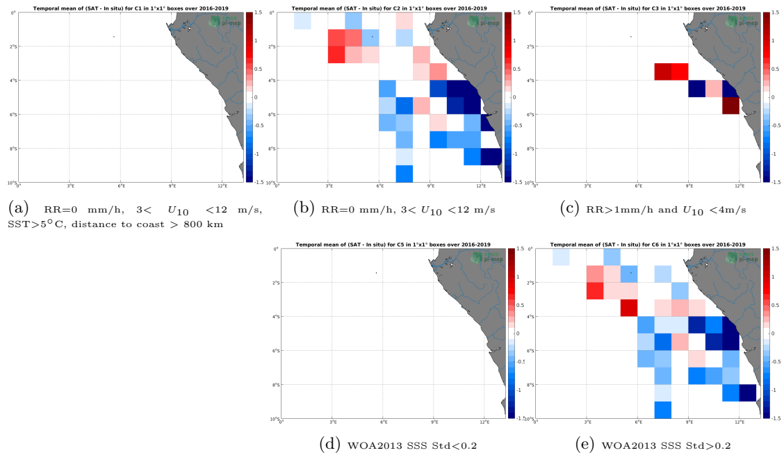
Figure 12: Temporal mean gridded over spatial boxes of size 1^\circ \times 1^\circ of \Delta SSS (SMAP-L2-JPL-V4.3 - TSG-LEGOS-DM) for 5 different subdatasets corresponding to:RR=0 mm/h, 3 < U_{10} < 12 m/s, SST > 5^\circ\text{C} , distance to coast > 800 km (a), RR=0 mm/h, 3 < U_{10} < 12 m/s (b), RR > 1 mm/h and U_{10} < 4 m/s (c), WOA2013 SSS Std < 0.2 (d), WOA2013 SSS Std > 0.2 (e).
