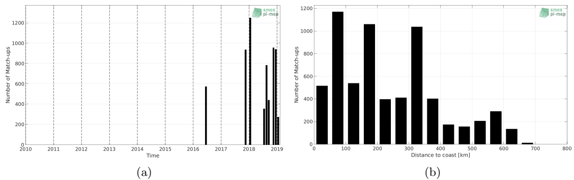
Figure 1: Number of match-ups between TSG-LEGOS-DM and SMAP-L2-JPL-V4.3 SSS as a function of time (a) and as function of the distance to coast (b) over the Congo river plume Pi-MEP region and for the full satellite product period.
