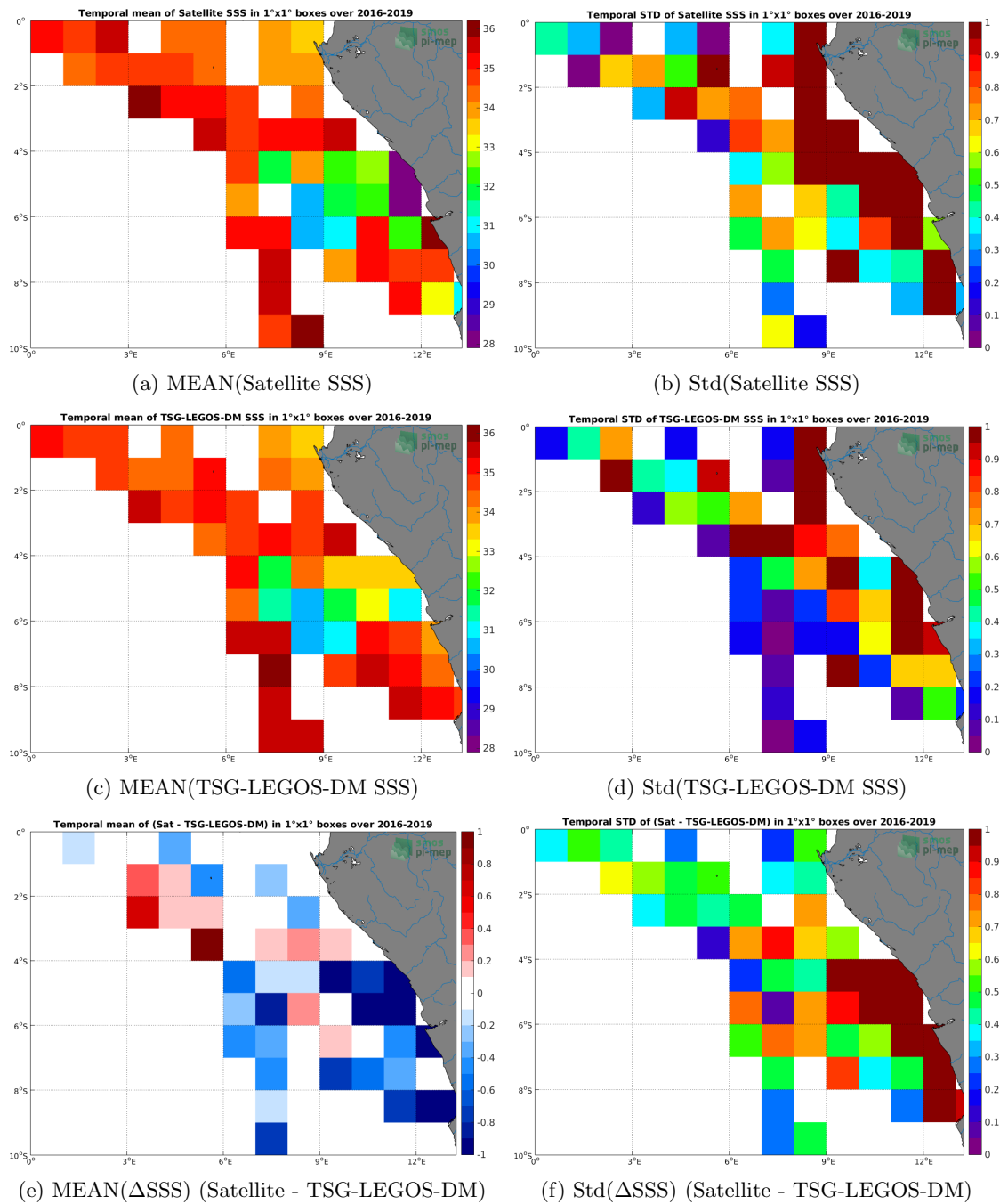
Figure 6: Temporal mean (left) and Std (right) of SSS from SMAP-L2-JPL-V4.3 (top), TSG-LEGOS-DM (middle), and of \Delta SSS (Satellite - TSG-LEGOS-DM). Only match-up pairs are used to generate these maps.
