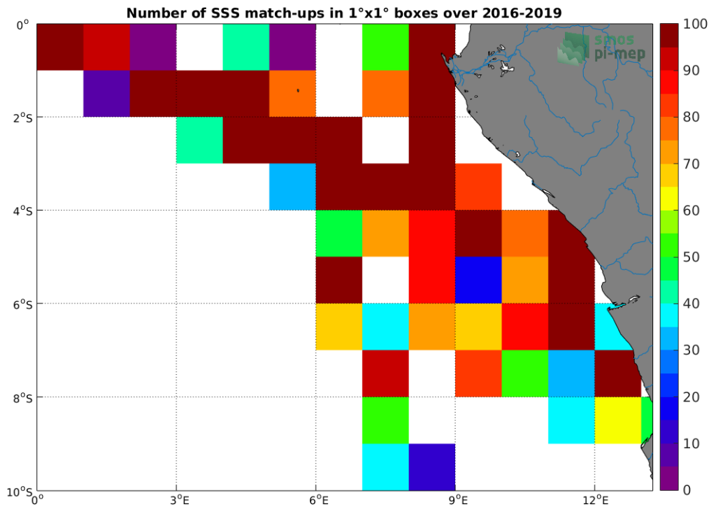
Figure 4: Number of SSS match-ups between TSG-LEGOS-DM SSS and the SMAP-L2-JPL-V4.3 SSS product for the Congo river plume Pi-MEP region over 1°x1° boxes and for the full satellite product period.
