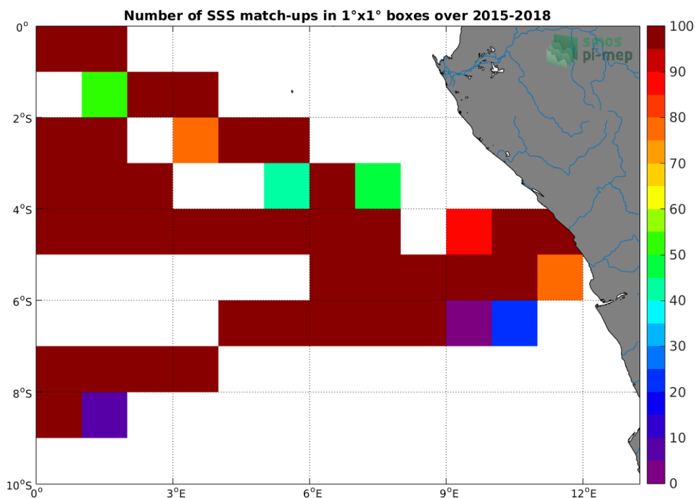
Figure 4: Number of SSS match-ups between TSG-GOSUD-Research-vessel SSS and the SMAP-L2-JPL-V4.3 SSS product for the Congo river plume Pi-MEP region over 1^\circ \times 1^\circ boxes and for the full satellite product period.
