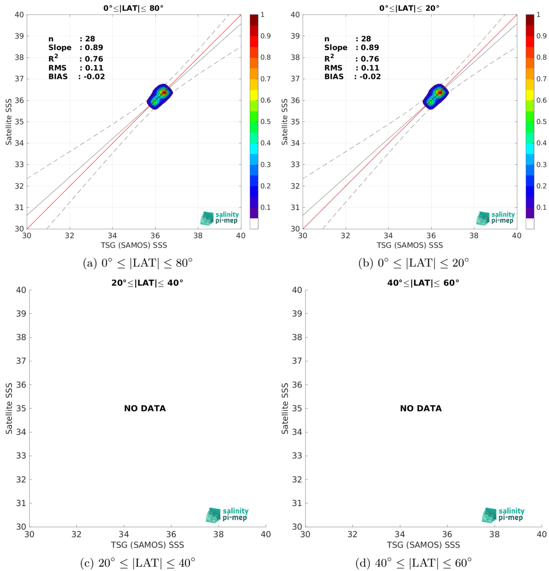
Figure 10: Contour maps of the concentration of CCI SSS L4 Merged-OI v5.5 - 7-day running (ESA) SSS (y-axis) versus TSG (SAMOS) SSS (x-axis) at match-up pairs for different latitude bands. For each plot, the red line shows x=y . The black thin and dashed lines indicate a linear fit through the data cloud and the \pm 95\% confidence levels, respectively. The number match-up pairs n , the slope and R^2 coefficient of the linear fit, the root mean square (RMS) and the mean bias between satellite and in situ data are indicated for each latitude band in each plots.
