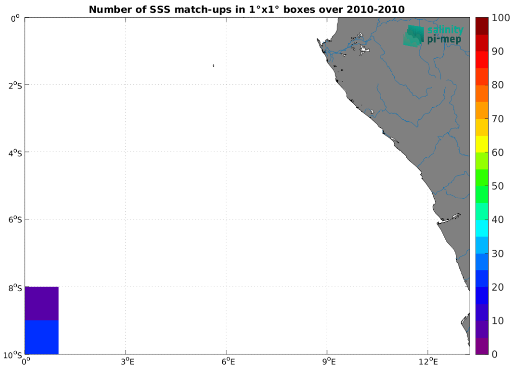
Figure 5: Number of SSS match-ups between TSG (SAMOS) SSS and the CCI SSS L4 Merged-OI v5.5 - 7-day running (ESA) SSS product for the Congo river plume Pi-MEP region over 1^\circ \times 1^\circ boxes and for the full satellite product period.
