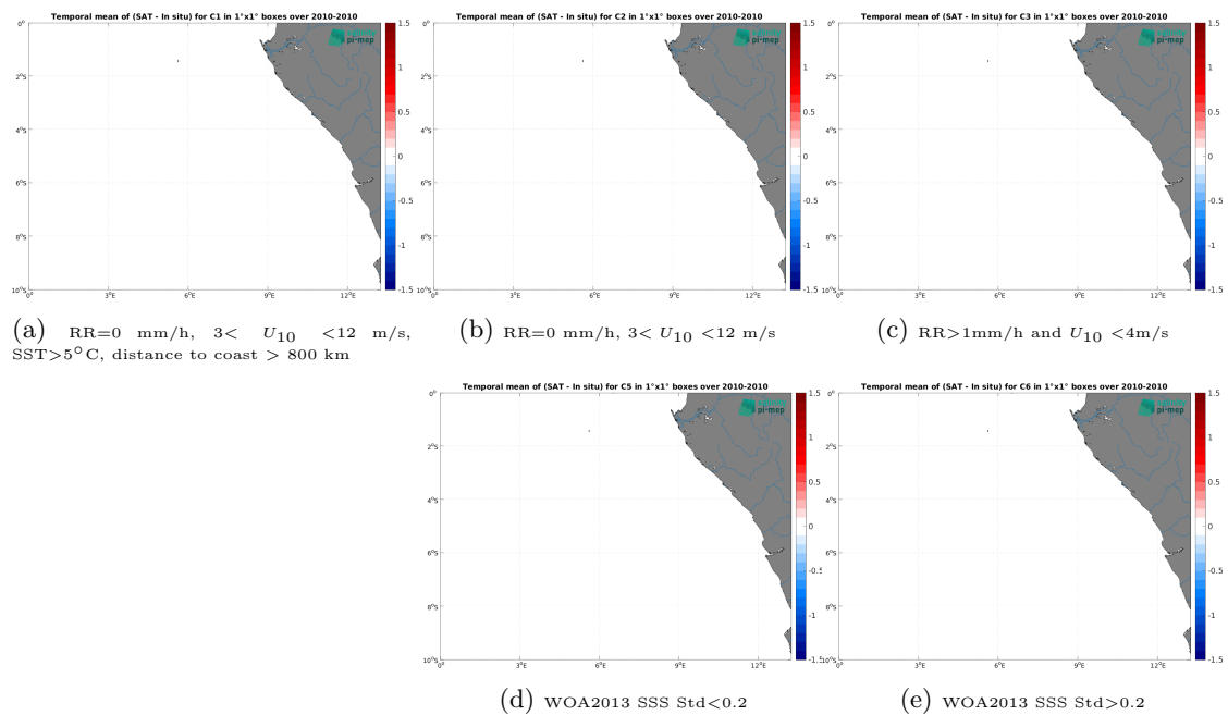
Figure 14: Temporal mean gridded over spatial boxes of size 1^\circ \times 1^\circ of \Delta SSS (CCI SSS L4 Merged-OI v5.5 - 7-day running (ESA) - TSG (SAMOS)) for 5 different subdatasets corresponding to:RR=0 mm/h, 3 < U_{10} < 12 m/s, SST > 5^\circ\text{C} , distance to coast > 800 km (a), RR=0 mm/h, 3 < U_{10} < 12 m/s (b), RR > 1 mm/h and U_{10} < 4 m/s (c), WOA2013 SSS Std < 0.2 (d), WOA2013 SSS Std > 0.2 (e).
