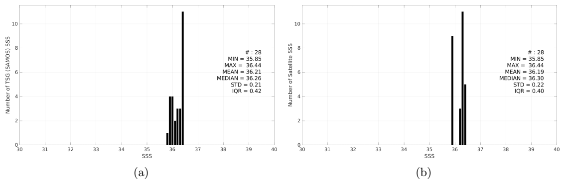
Figure 3: Histograms of SSS from TSG (SAMOS) (a) and CCI SSS L4 Merged-OI v5.5 - 7-day running (ESA) (b) considering all match-up pairs per bins of 0.1 over the Congo river plume Pi-MEP region and for the full satellite product period.
