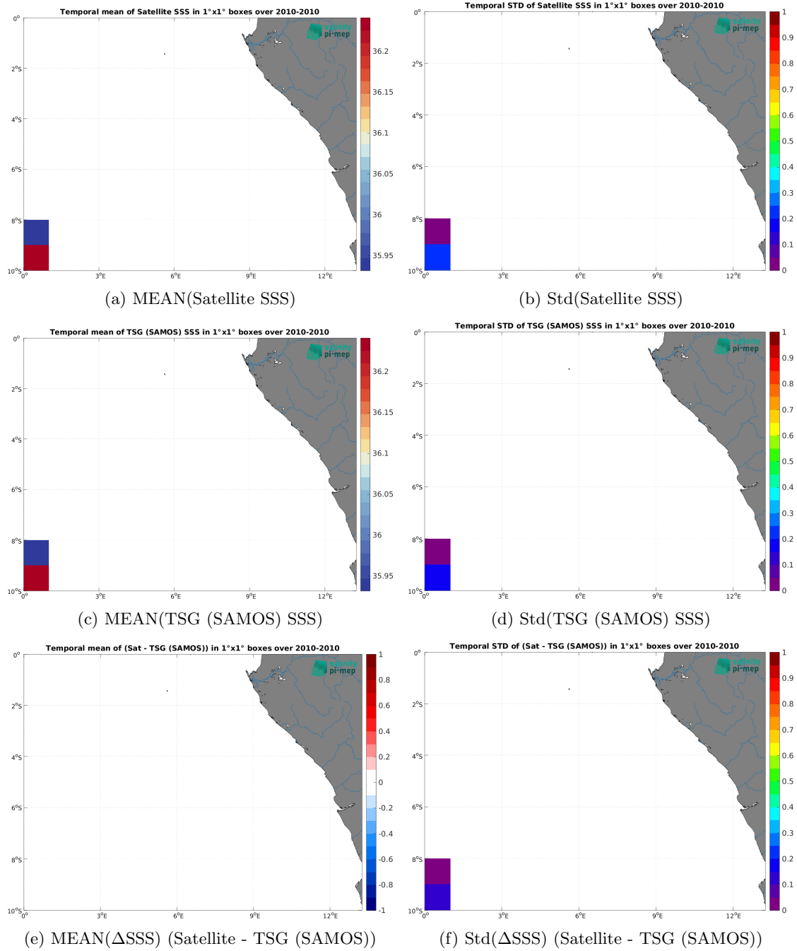
Figure 7: Temporal mean (left) and Std (right) of SSS from CCI SSS L4 Merged-OI v5.5 - 7-day running (ESA) (top), TSG (SAMOS) (middle), and of \Delta SSS (Satellite - TSG (SAMOS)). Only match-up pairs are used to generate these maps.
