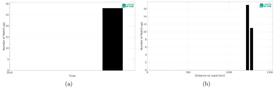
Figure 2: Number of match-ups between TSG (SAMOS) and CCI SSS L4 Merged-OI v5.5 - 7-day running (ESA) SSS as a function of time (a) and as function of the distance to coast (b) over the Congo river plume Pi-MEP region and for the full satellite product period.
