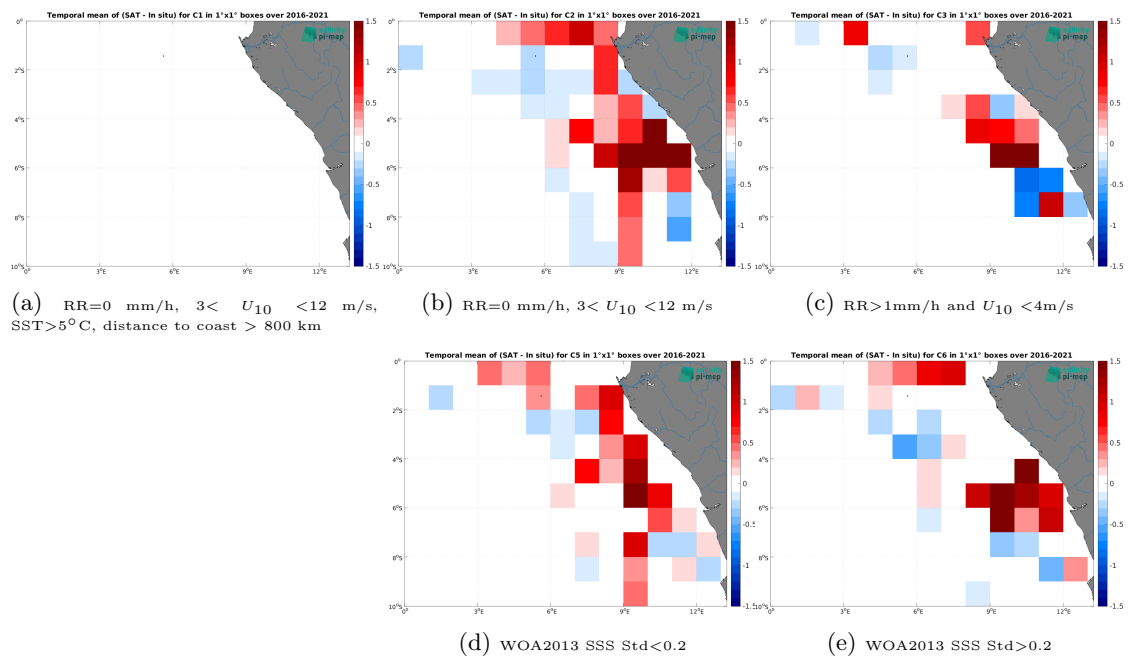
Figure 14: Temporal mean gridded over spatial boxes of size 1^\circ \times 1^\circ of \Delta SSS (CCI SSS L4 Merged-OI v5.5 - 7-day running (ESA) - TSG (LEGOS-DM)) for 5 different subdatasets corresponding to:RR=0 mm/h, 3 < U_{10} < 12 m/s, SST > 5°C, distance to coast > 800 km (a), RR=0 mm/h, 3 < U_{10} < 12 m/s (b), RR > 1mm/h and U_{10} < 4 m/s (c), WOA2013 SSS Std < 0.2 (d), WOA2013 SSS Std > 0.2 (e).
