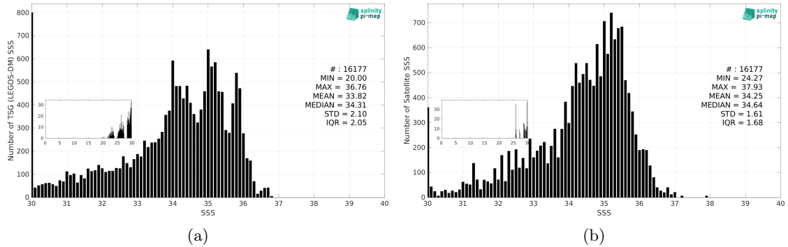
Figure 3: Histograms of SSS from TSG (LEGOS-DM) (a) and CCI SSS L4 Merged-OI v5.5 - 7-day running (ESA) (b) considering all match-up pairs per bins of 0.1 over the Congo river plume Pi-MEP region and for the full satellite product period.
