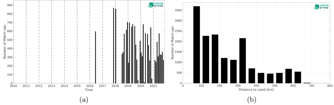
Figure 2: Number of match-ups between TSG (LEGOS-DM) and CCI SSS L4 Merged-OI v5.5 - 7-day running (ESA) SSS as a function of time (a) and as function of the distance to coast (b) over the Congo river plume Pi-MEP region and for the full satellite product period.
