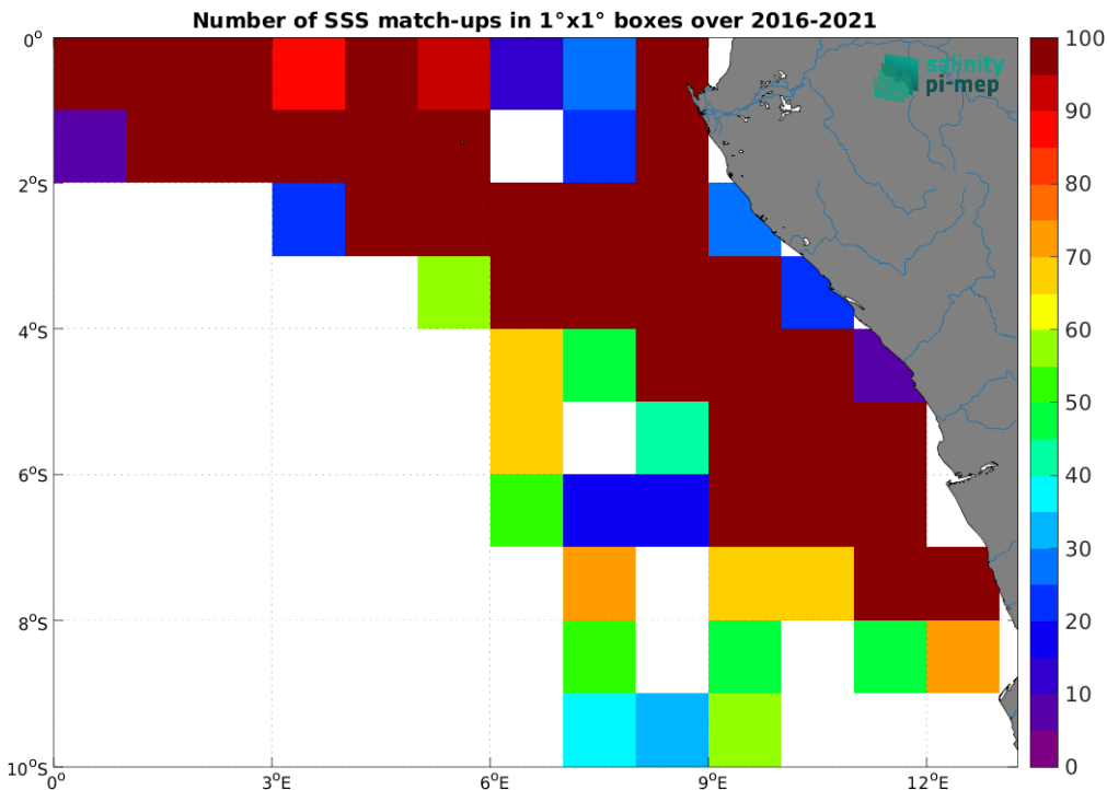
Figure 5: Number of SSS match-ups between TSG (LEGOS-DM) SSS and the CCI SSS L4 Merged-OI v5.5 - 7-day running (ESA) SSS product for the Congo river plume Pi-MEP region over 1^\circ \times 1^\circ boxes and for the full satellite product period.
