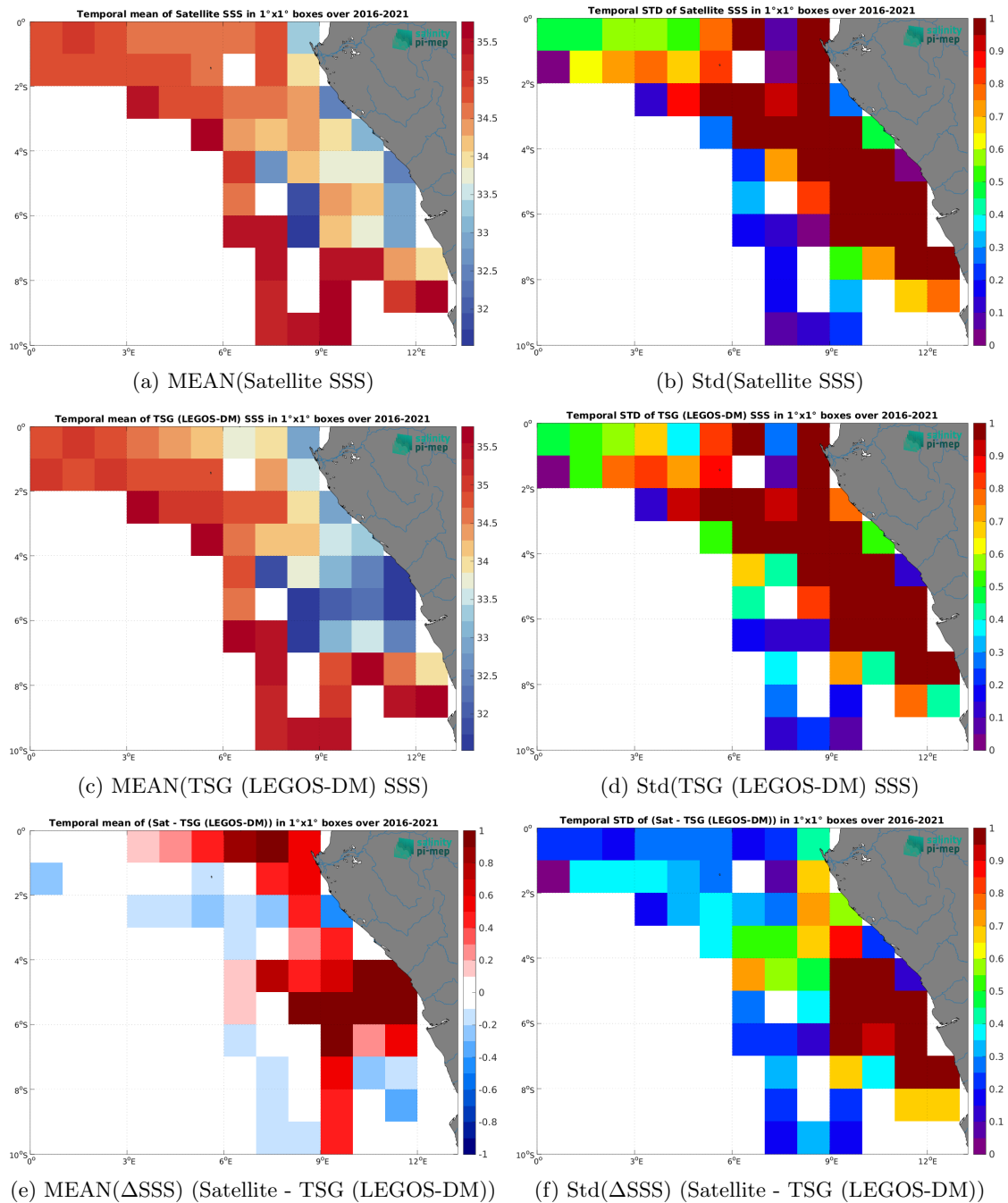
Figure 7: Temporal mean (left) and Std (right) of SSS from CCI SSS L4 Merged-OI v5.5 - 7-day running (ESA) (top), TSG (LEGOS-DM) (middle), and of \Delta SSS (Satellite - TSG (LEGOS-DM)). Only match-up pairs are used to generate these maps.
