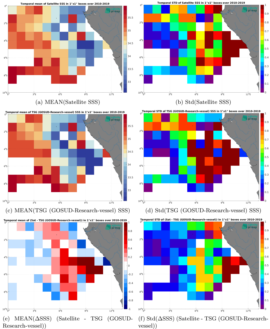
Figure 7: Temporal mean (left) and Std (right) of SSS from CCI SSS L4 Merged-OI v5.5 - 7-day running (ESA) (top), TSG (GOSUD-Research-vessel) (middle), and of \Delta SSS (Satellite - TSG (GOSUD-Research-vessel)). Only match-up pairs are used to generate these maps.
