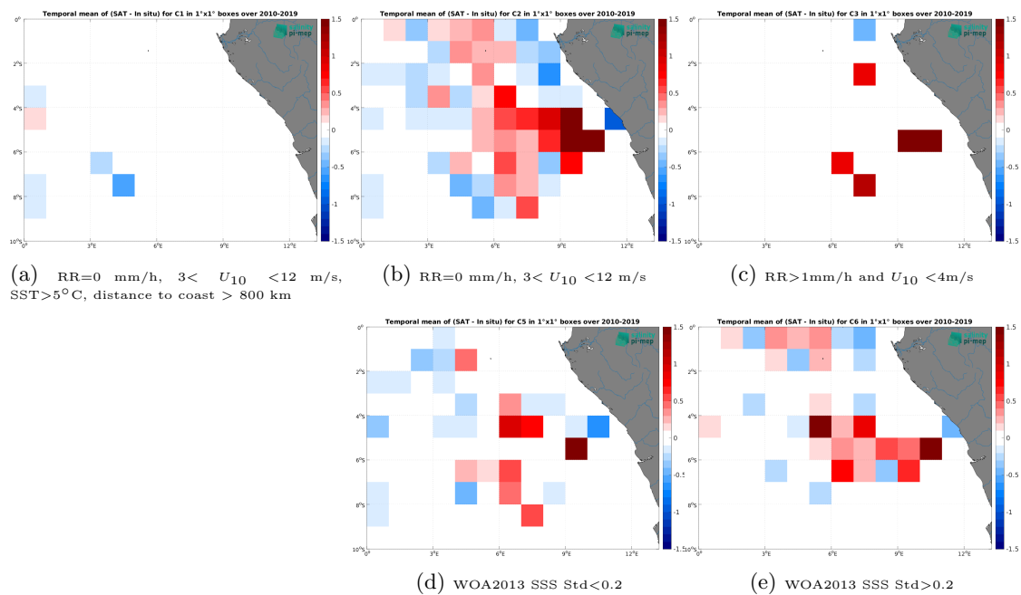
Figure 14: Temporal mean gridded over spatial boxes of size 1^\circ \times 1^\circ of \Delta SSS (CCI SSS L4 Merged-OI v5.5 - 7-day running (ESA) - TSG (GOSUD-Research-vessel)) for 5 different subdatasets corresponding to:RR=0 mm/h, 3 < U_{10} < 12 m/s, SST > 5^\circ\text{C} , distance to coast > 800 km (a), RR=0 mm/h, 3 < U_{10} < 12 m/s (b), RR > 1 mm/h and U_{10} < 4 m/s (c), WOA2013 SSS Std < 0.2 (d), WOA2013 SSS Std > 0.2 (e).
