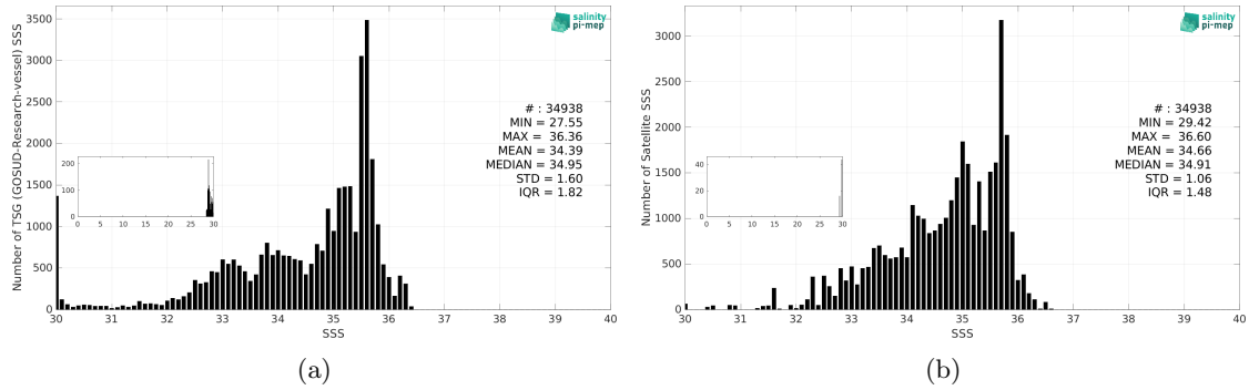
Figure 3: Histograms of SSS from TSG (GOSUD-Research-vessel) (a) and CCI SSS L4 Merged-OI v5.5 - 7-day running (ESA) (b) considering all match-up pairs per bins of 0.1 over the Congo river plume Pi-MEP region and for the full satellite product period.
