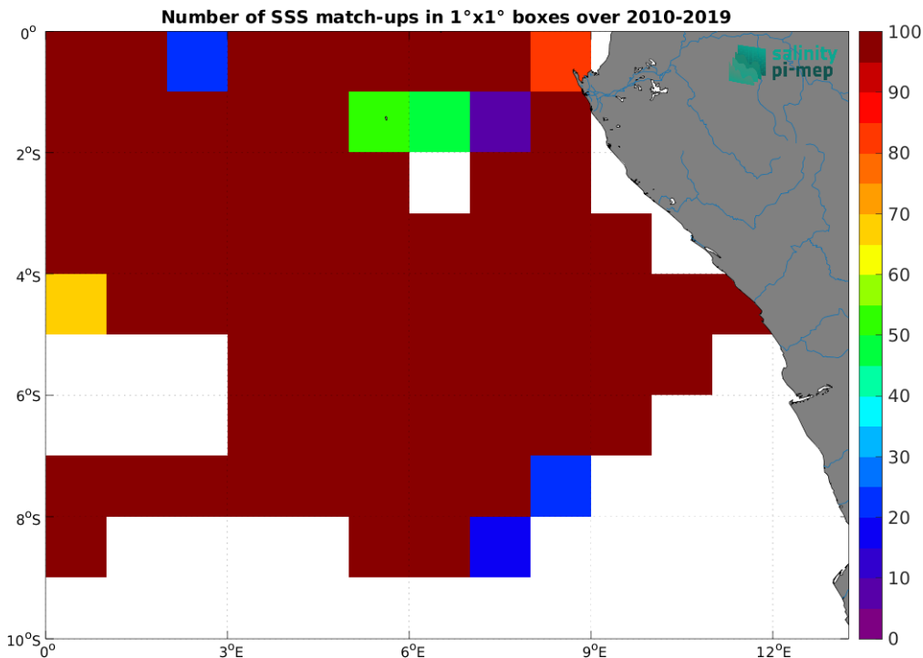
Figure 5: Number of SSS match-ups between TSG (GOSUD-Research-vessel) SSS and the CCI SSS L4 Merged-OI v5.5 - 7-day running (ESA) SSS product for the Congo river plume Pi-MEP region over 1^\circ \times 1^\circ boxes and for the full satellite product period.
