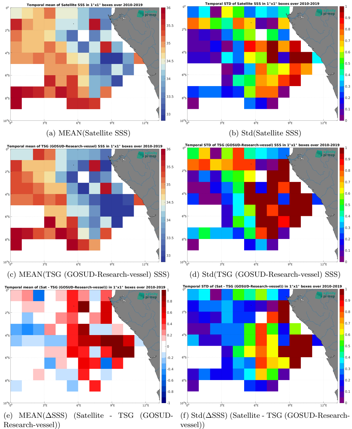
Figure 7: Temporal mean (left) and Std (right) of SSS from CCI SSS L4 Merged-OI v5.5 - 30-day running (ESA) (top), TSG (GOSUD-Research-vessel) (middle), and of \Delta SSS (Satellite - TSG (GOSUD-Research-vessel)). Only match-up pairs are used to generate these maps.
