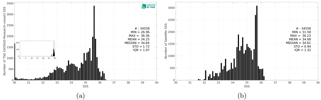
Figure 3: Histograms of SSS from TSG (GOSUD-Research-vessel) (a) and CCI SSS L4 Merged-OI v5.5 - 30-day running (ESA) (b) considering all match-up pairs per bins of 0.1 over the Congo river plume Pi-MEP region and for the full satellite product period.
