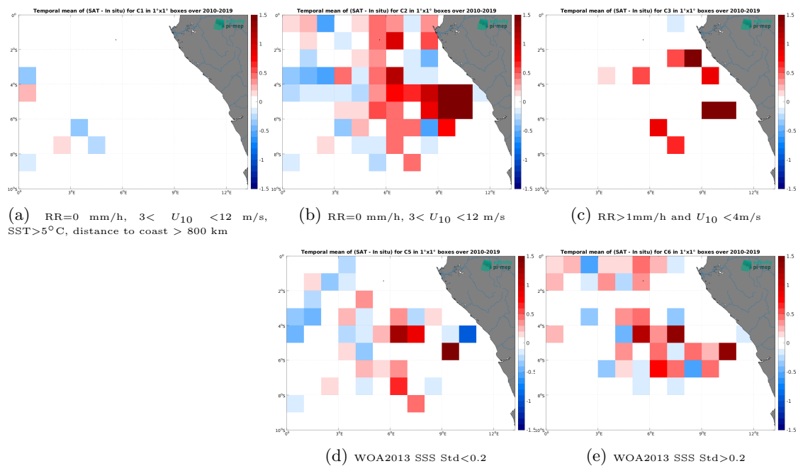
Figure 14: Temporal mean gridded over spatial boxes of size 1^\circ \times 1^\circ of \Delta SSS (CCI SSS L4 Merged-OI v5.5 - 30-day running (ESA) - TSG (GOSUD-Research-vessel)) for 5 different subdatasets corresponding to: RR=0 mm/h, 3 < U_{10} < 12 m/s, SST > 5^\circ\text{C} , distance to coast > 800 km (a), RR=0 mm/h, 3 < U_{10} < 12 m/s (b), RR > 1 mm/h and U_{10} < 4 m/s (c), WOA2013 SSS Std < 0.2 (d), WOA2013 SSS Std > 0.2 (e).
