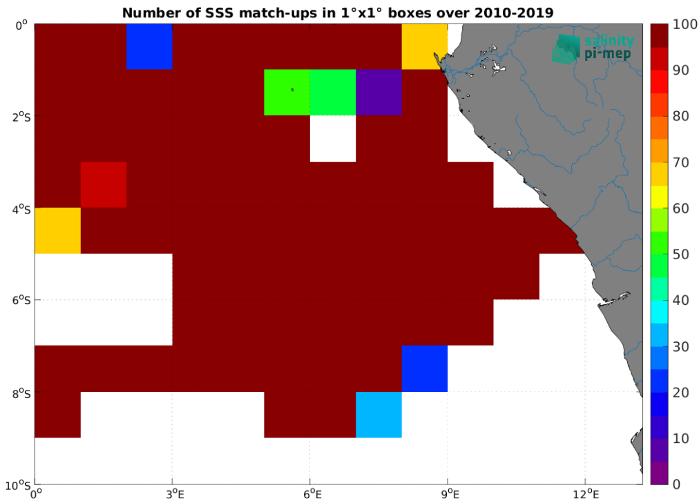
Figure 5: Number of SSS match-ups between TSG (GOSUD-Research-vessel) SSS and the CCI SSS L4 Merged-OI v5.5 - 30-day running (ESA) SSS product for the Congo river plume Pi-MEP region over 1^\circ \times 1^\circ boxes and for the full satellite product period.
