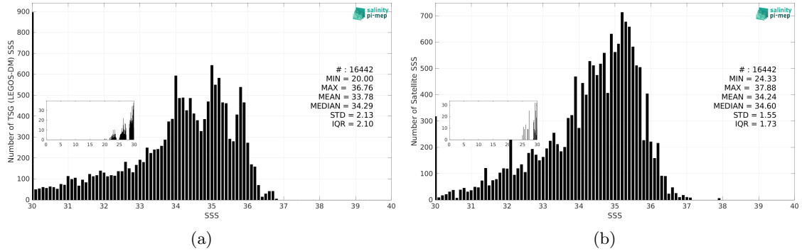
Figure 3: Histograms of SSS from TSG (LEGOS-DM) (a) and CCI SSS L4 Merged-OI v4.41 - 7-day running (ESA) (b) considering all match-up pairs per bins of 0.1 over the Congo river plume Pi-MEP region and for the full satellite product period.
