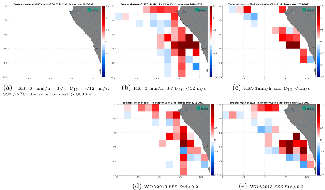
Figure 14: Temporal mean gridded over spatial boxes of size 1^\circ \times 1^\circ of \Delta SSS (CCI SSS L4 Merged-OI v4.41 - 7-day running (ESA) - TSG (LEGOS-DM)) for 5 different subdatasets corresponding to:RR=0 mm/h, 3 < U_{10} < 12 m/s, SST > 5^\circ\text{C} , distance to coast > 800 km (a), RR=0 mm/h, 3 < U_{10} < 12 m/s (b), RR > 1 mm/h and U_{10} < 4 m/s (c), WOA2013 SSS Std < 0.2 (d), WOA2013 SSS Std > 0.2 (e).
