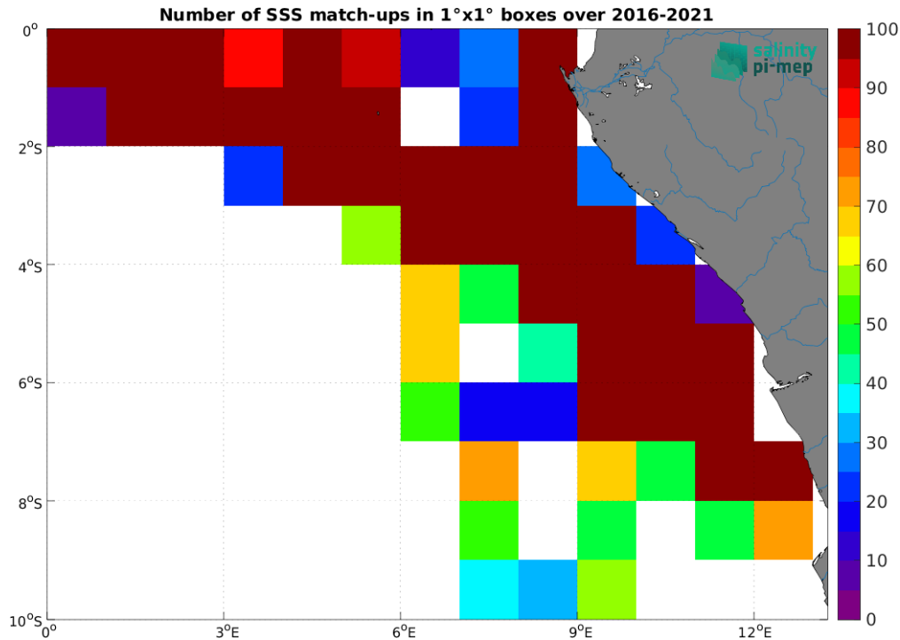
Figure 5: Number of SSS match-ups between TSG (LEGOS-DM) SSS and the CCI SSS L4 Merged-OI v4.41 - 7-day running (ESA) SSS product for the Congo river plume Pi-MEP region over 1^\circ \times 1^\circ boxes and for the full satellite product period.
