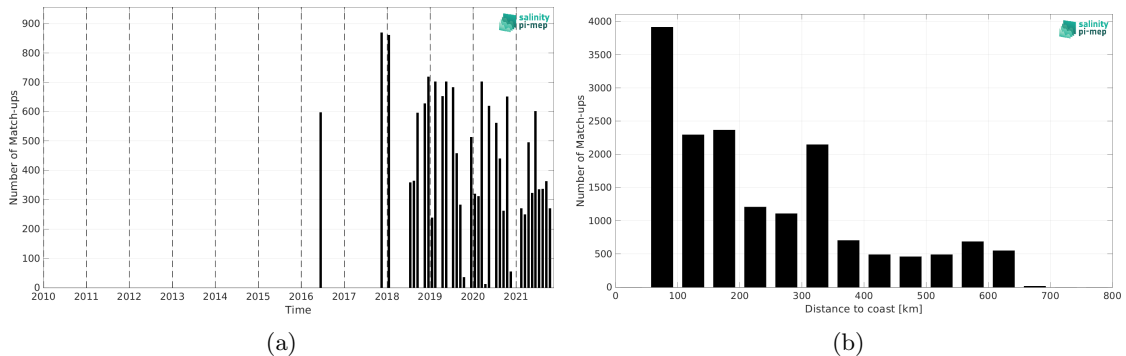
Figure 2: Number of match-ups between TSG (LEGOS-DM) and CCI SSS L4 Merged-OI v4.41 - 7-day running (ESA) SSS as a function of time (a) and as function of the distance to coast (b) over the Congo river plume Pi-MEP region and for the full satellite product period.
