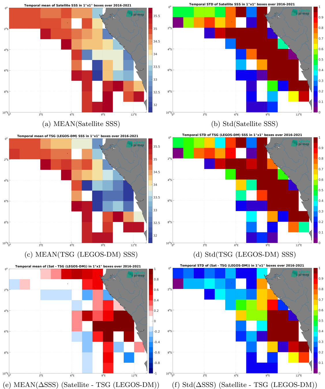
Figure 7: Temporal mean (left) and Std (right) of SSS from CCI SSS L4 Merged-OI v4.41 - 7-day running (ESA) (top), TSG (LEGOS-DM) (middle), and of \Delta SSS (Satellite - TSG (LEGOS-DM)). Only match-up pairs are used to generate these maps.
