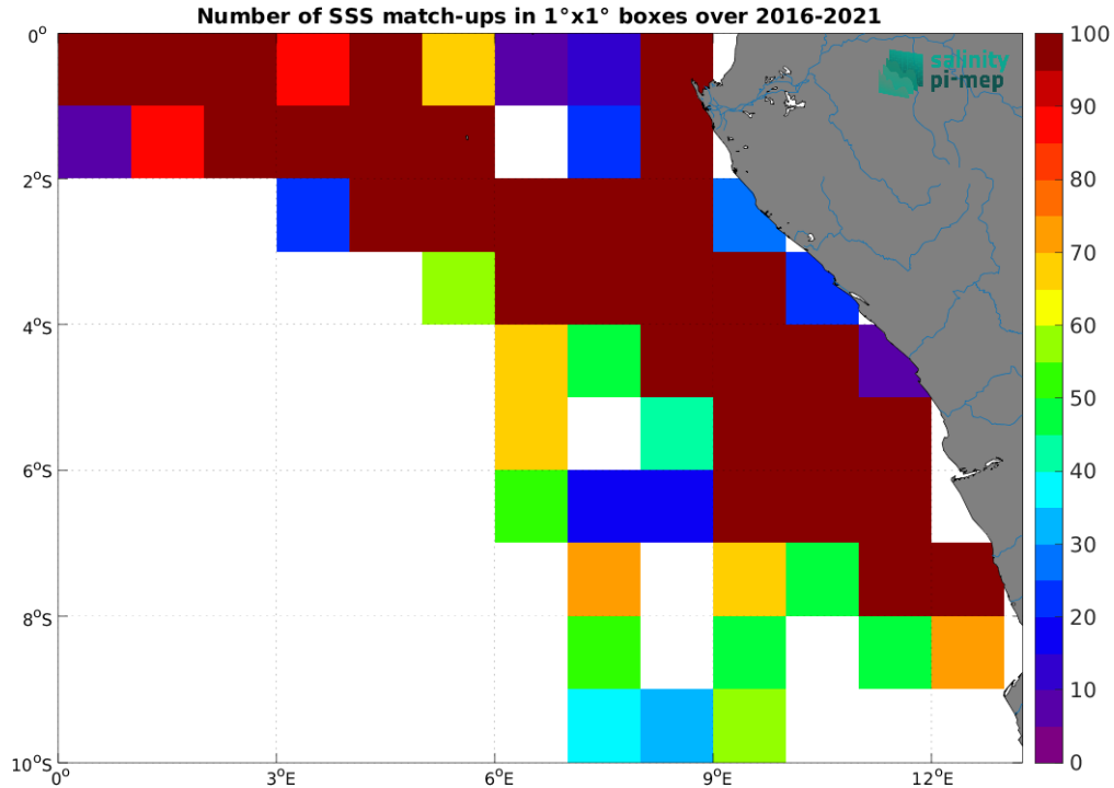
Figure 4: Number of SSS match-ups between TSG (LEGOS-DM) SSS and the CCI SSS L4 Merged-OI v4.4 - 7-day running (ESA) SSS product for the Congo river plume Pi-MEP region over 1^\circ \times 1^\circ boxes and for the full satellite product period.
