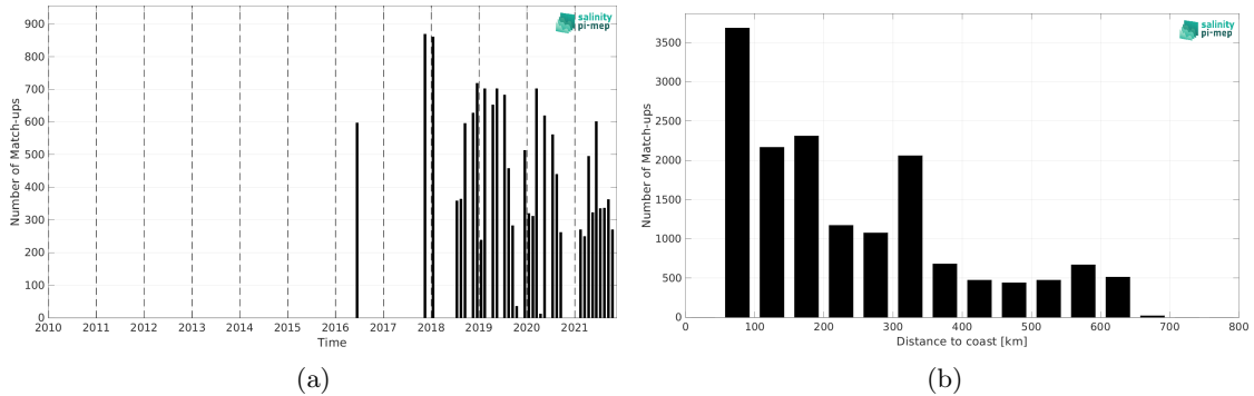
Figure 1: Number of match-ups between TSG (LEGOS-DM) and CCI SSS L4 Merged-OI v4.4 - 7-day running (ESA) SSS as a function of time (a) and as function of the distance to coast (b) over the Congo river plume Pi-MEP region and for the full satellite product period.
