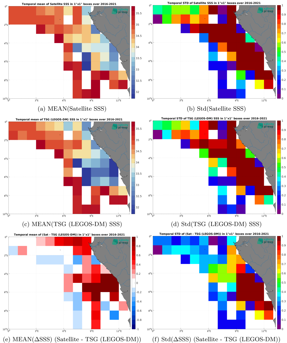
Figure 6: Temporal mean (left) and Std (right) of SSS from CCI SSS L4 Merged-OI v4.4 - 7-day running (ESA) (top), TSG (LEGOS-DM) (middle), and of \Delta SSS (Satellite - TSG (LEGOS-DM)). Only match-up pairs are used to generate these maps.
