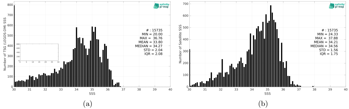
Figure 2: Histograms of SSS from TSG (LEGOS-DM) (a) and CCI SSS L4 Merged-OI v4.4 - 7-day running (ESA) (b) considering all match-up pairs per bins of 0.1 over the Congo river plume Pi-MEP region and for the full satellite product period.
