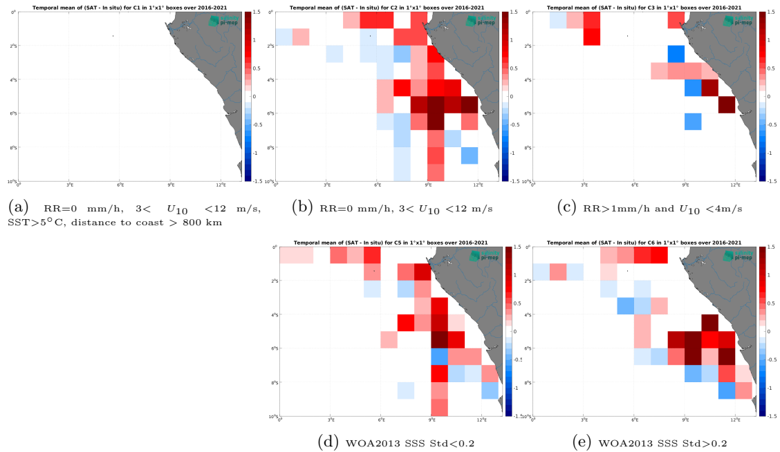
Figure 12: Temporal mean gridded over spatial boxes of size 1^{\circ}\times 1^{\circ} of \Delta\text{SSS} (CCI SSS L4 Merged-OI v4.4 - 7-day running (ESA) - TSG (LEGOS-DM)) for 5 different subdatasets corresponding to:RR=0 mm/h, 3 < U_{10} < 12 m/s, SST >5^{\circ}\text{C} , distance to coast > 800 km (a), RR=0 mm/h, 3 < U_{10} < 12 m/s (b), RR >1 mm/h and U_{10} < 4 m/s (c), WOA2013 SSS Std <0.2 (d), WOA2013 SSS Std >0.2 (e).
