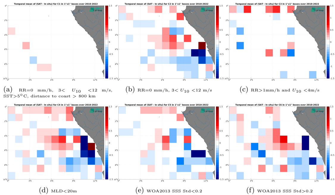
Figure 12: Temporal mean gridded over spatial boxes of size 1^\circ \times 1^\circ of \Delta SSS (CCI SSS L4 Merged-OI v4.4 - 7-day running (ESA) - Argo) for 6 different subdatasets corresponding to:RR=0 mm/h, 3 < U_{10} < 12 m/s, SST >5^\circ C, distance to coast > 800 km (a), RR=0 mm/h, 3 < U_{10} < 12 m/s (b), RR >1 mm/h and U_{10} < 4 m/s (c),MLD <20 m (d),WOA2013 SSS Std <0.2 (e),WOA2013 SSS Std >0.2 (f).
