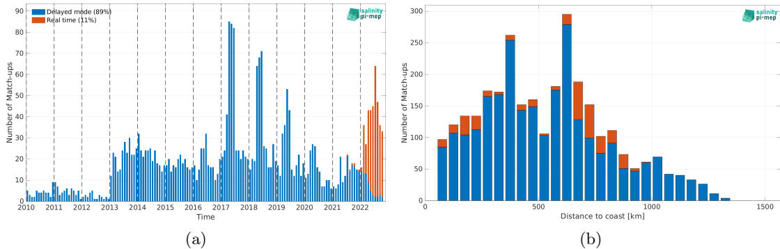
Figure 1: Number of match-ups between Argo and CCI SSS L4 Merged-OI v4.4 - 7-day running (ESA) SSS as a function of time (a) and as function of the distance to coast (b) over the Congo river plume Pi-MEP region and for the full satellite product period.
