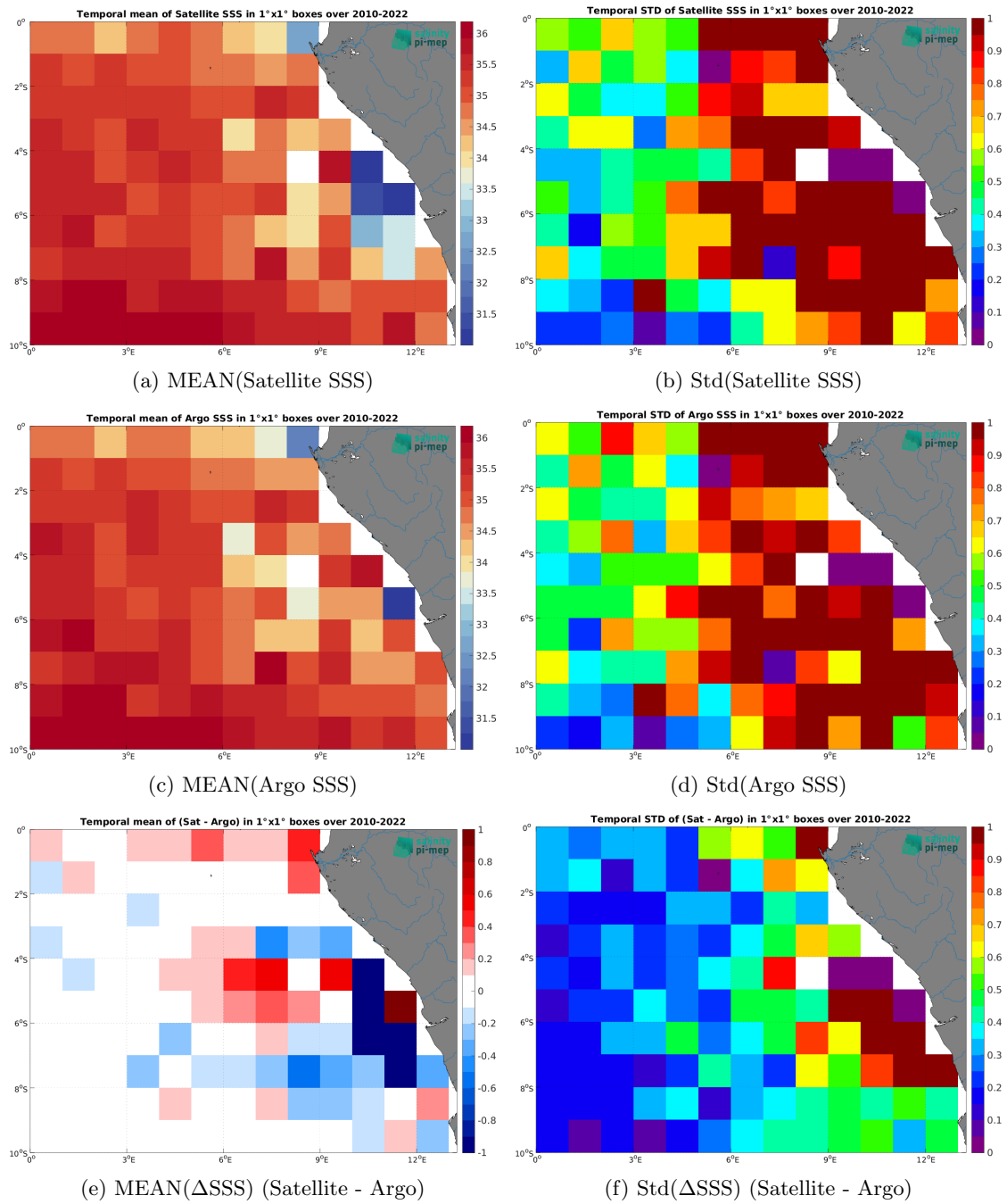
Figure 6: Temporal mean (left) and Std (right) of SSS from CCI SSS L4 Merged-OI v4.4 - 7-day running (ESA) (top), Argo (middle), and of \Delta SSS (Satellite - Argo). Only match-up pairs are used to generate these maps.
