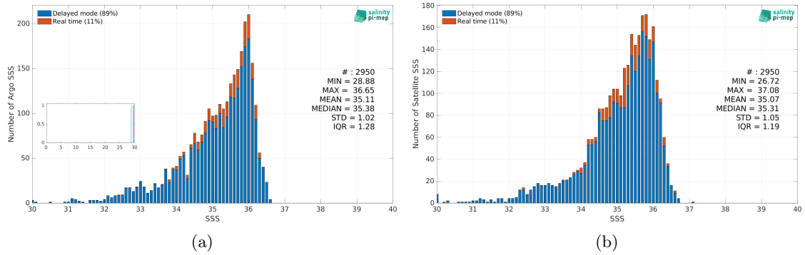
Figure 2: Histograms of SSS from Argo (a) and CCI SSS L4 Merged-OI v4.4 - 7-day running (ESA) (b) considering all match-up pairs per bins of 0.1 over the Congo river plume Pi-MEP region and for the full satellite product period.
