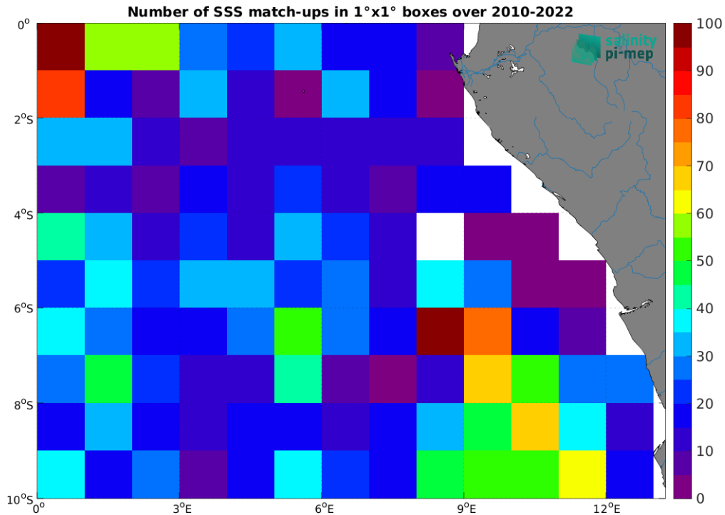
Figure 4: Number of SSS match-ups between Argo SSS and the CCI SSS L4 Merged-OI v4.4 - 7-day running (ESA) SSS product for the Congo river plume Pi-MEP region over 1^\circ \times 1^\circ boxes and for the full satellite product period.
