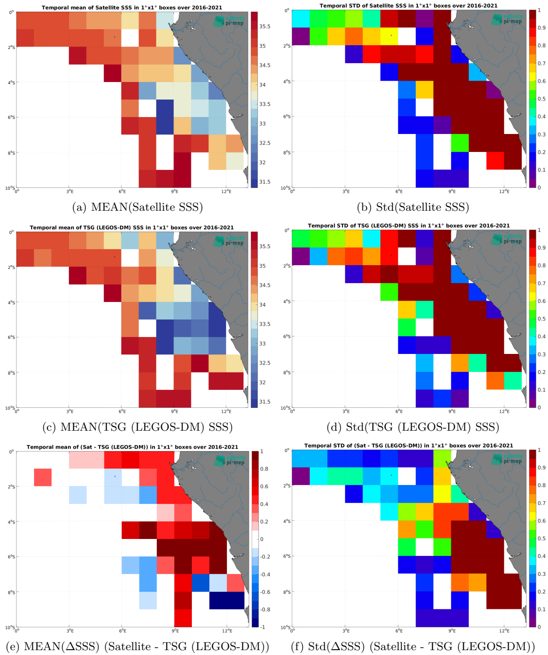
Figure 6: Temporal mean (left) and Std (right) of SSS from CCI SSS L4 Merged-OI v4.4 - 30-day running (ESA) (top), TSG (LEGOS-DM) (middle), and of \Delta SSS (Satellite - TSG (LEGOS-DM)). Only match-up pairs are used to generate these maps.
