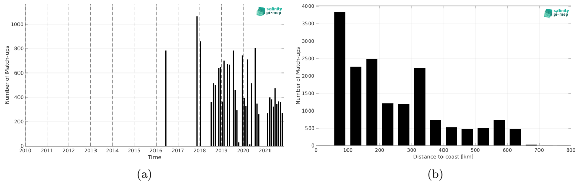
Figure 1: Number of match-ups between TSG (LEGOS-DM) and CCI SSS L4 Merged-OI v4.4 - 30-day running (ESA) SSS as a function of time (a) and as function of the distance to coast (b) over the Congo river plume Pi-MEP region and for the full satellite product period.
