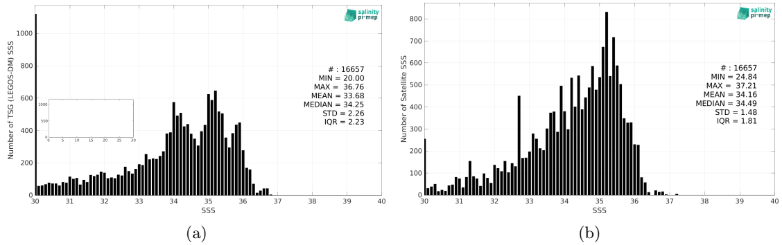
Figure 2: Histograms of SSS from TSG (LEGOS-DM) (a) and CCI SSS L4 Merged-OI v4.4 - 30-day running (ESA) (b) considering all match-up pairs per bins of 0.1 over the Congo river plume Pi-MEP region and for the full satellite product period.
