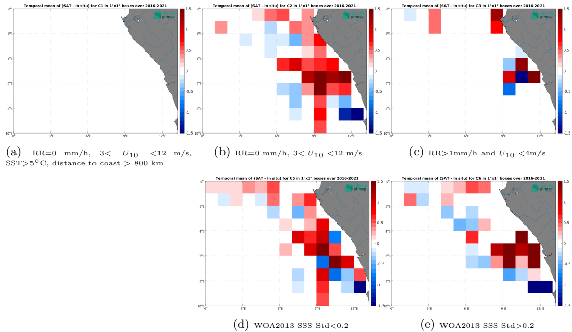
Figure 12: Temporal mean gridded over spatial boxes of size 1^{\circ}\times 1^{\circ} of \Delta\text{SSS} (CCI SSS L4 Merged-OI v4.4 - 30-day running (ESA) - TSG (LEGOS-DM)) for 5 different subdatasets corresponding to:RR=0 mm/h, 3 < U_{10} < 12 m/s, SST >5^{\circ}\text{C} , distance to coast > 800 km (a), RR=0 mm/h, 3 < U_{10} < 12 m/s (b), RR >1 mm/h and U_{10} < 4 m/s (c), WOA2013 SSS Std <0.2 (d), WOA2013 SSS Std >0.2 (e).
