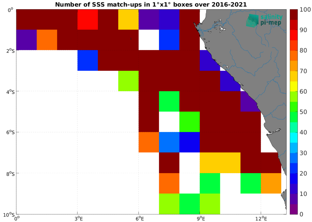
Figure 4: Number of SSS match-ups between TSG (LEGOS-DM) SSS and the CCI SSS L4 Merged-OI v4.4 - 30-day running (ESA) SSS product for the Congo river plume Pi-MEP region over 1^\circ \times 1^\circ boxes and for the full satellite product period.
