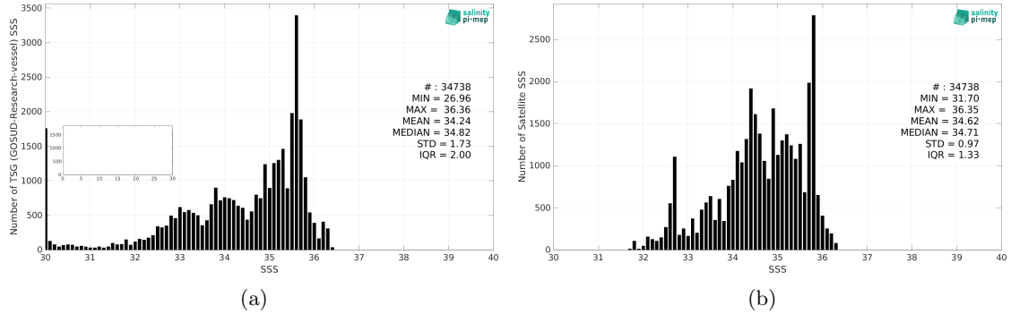
Figure 2: Histograms of SSS from TSG (GOSUD-Research-vessel) (a) and CCI SSS L4 Merged-OI v4.4 - 30-day running (ESA) (b) considering all match-up pairs per bins of 0.1 over the Congo river plume Pi-MEP region and for the full satellite product period.
