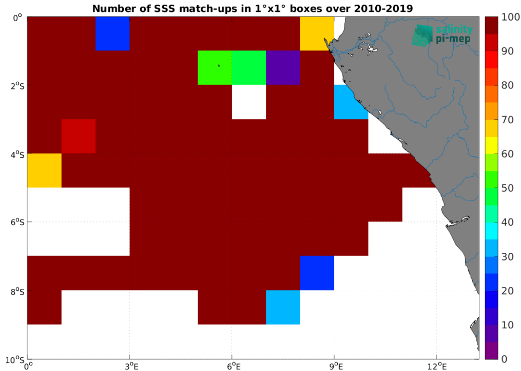
Figure 4: Number of SSS match-ups between TSG (GOSUD-Research-vessel) SSS and the CCI SSS L4 Merged-OI v4.4 - 30-day running (ESA) SSS product for the Congo river plume Pi-MEP region over 1^\circ \times 1^\circ boxes and for the full satellite product period.
