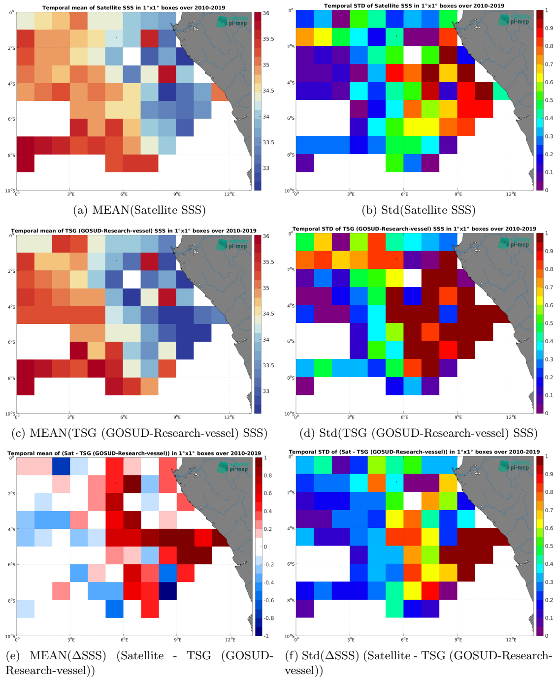
Figure 6: Temporal mean (left) and Std (right) of SSS from CCI SSS L4 Merged-OI v4.4 - 30-day running (ESA) (top), TSG (GOSUD-Research-vessel) (middle), and of \Delta SSS (Satellite - TSG (GOSUD-Research-vessel)). Only match-up pairs are used to generate these maps.
