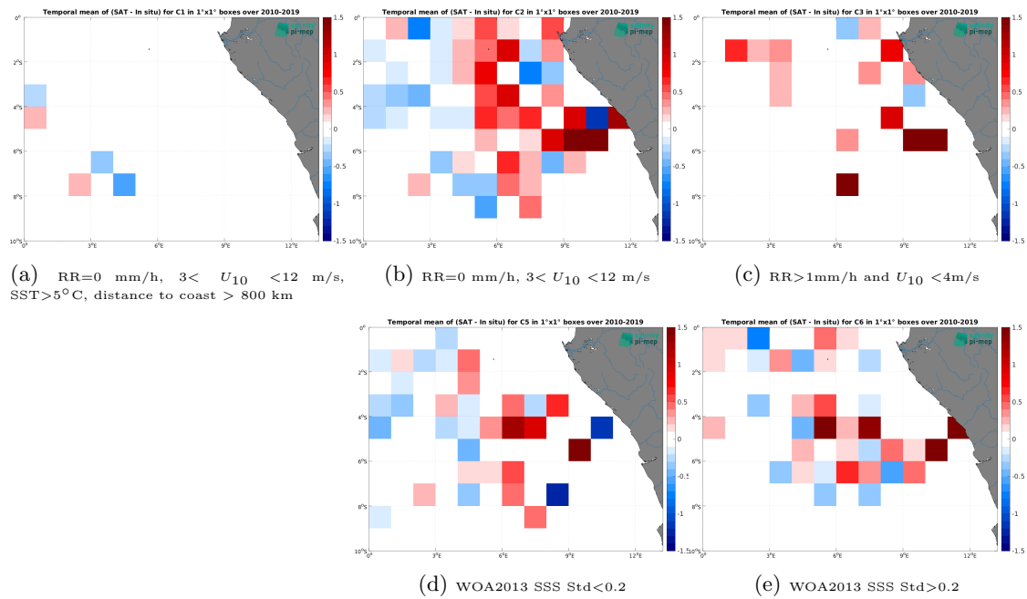
Figure 12: Temporal mean gridded over spatial boxes of size 1^\circ \times 1^\circ of \Delta SSS (CCI SSS L4 Merged-OI v4.4 - 30-day running (ESA) - TSG (GOSUD-Research-vessel)) for 5 different subdatasets corresponding to:RR=0 mm/h, 3 < U_{10} < 12 m/s, SST > 5^\circ\text{C} , distance to coast > 800 km (a), RR=0 mm/h, 3 < U_{10} < 12 m/s (b), RR > 1 mm/h and U_{10} < 4 m/s (c), WOA2013 SSS Std < 0.2 (d), WOA2013 SSS Std > 0.2 (e).
