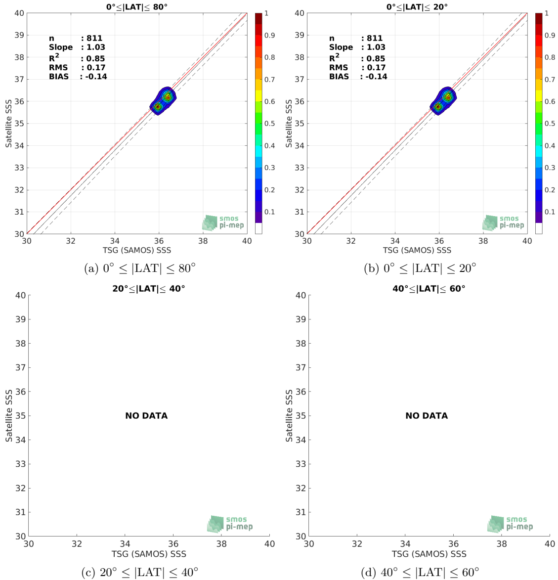
Figure 9: Contour maps of the concentration of CCI SSS L4 Merged-OI v3.2 - 7-day running (ESA) SSS ( y -axis) versus TSG (SAMOS) SSS ( x -axis) at match-up pairs for different latitude bands. For each plot, the red line shows x=y . The black thin and dashed lines indicate a linear fit through the data cloud and the \pm 95\% confidence levels, respectively. The number match-up pairs n , the slope and R^2 coefficient of the linear fit, the root mean square (RMS) and the mean bias between satellite and in situ data are indicated for each latitude band in each plots.
