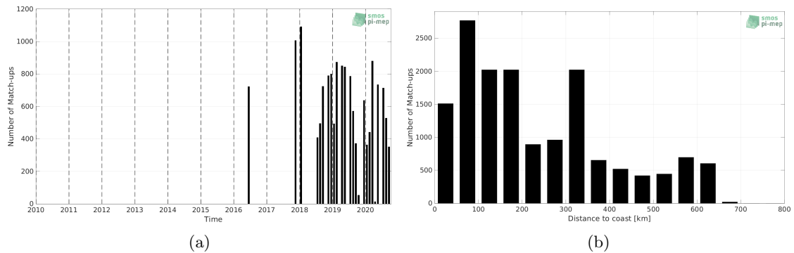
Figure 1: Number of match-ups between TSG (LEGOS-DM) and CCI SSS L4 Merged-OI v3.2 - 7-day running (ESA) SSS as a function of time (a) and as function of the distance to coast (b) over the Congo river plume Pi-MEP region and for the full satellite product period.
