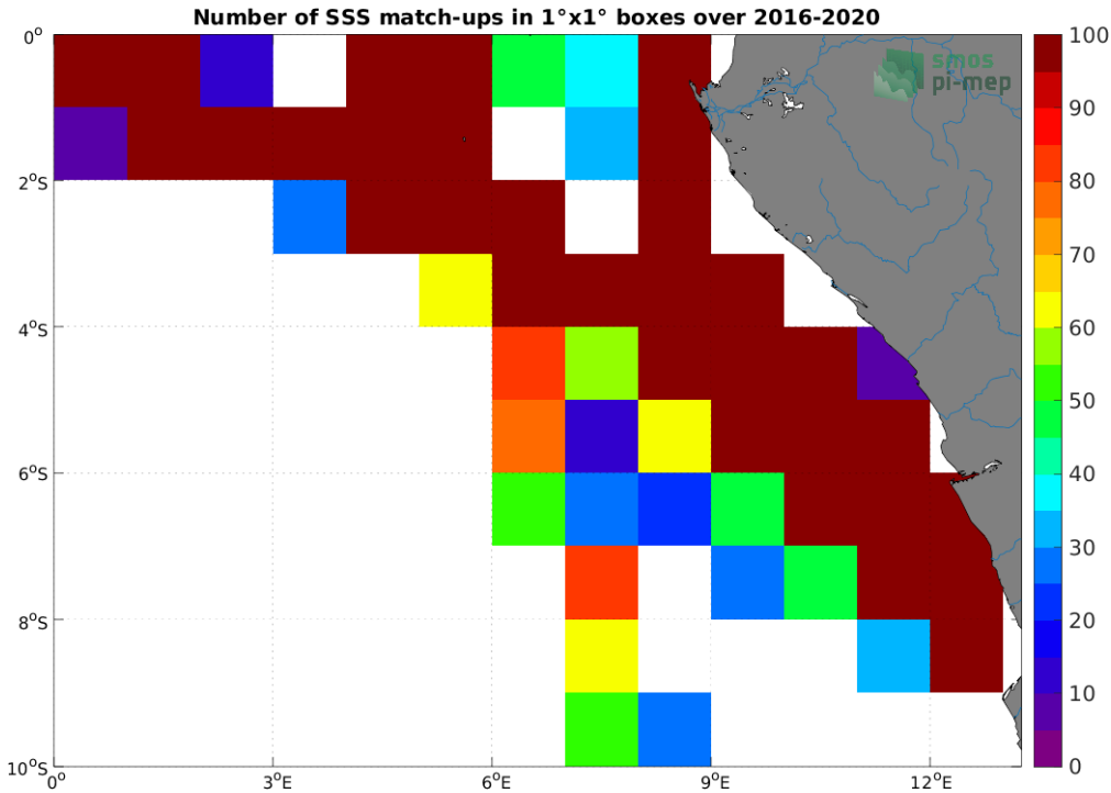
Figure 4: Number of SSS match-ups between TSG (LEGOS-DM) SSS and the CCI SSS L4 Merged-OI v3.2 - 7-day running (ESA) SSS product for the Congo river plume Pi-MEP region over 1^\circ \times 1^\circ boxes and for the full satellite product period.
