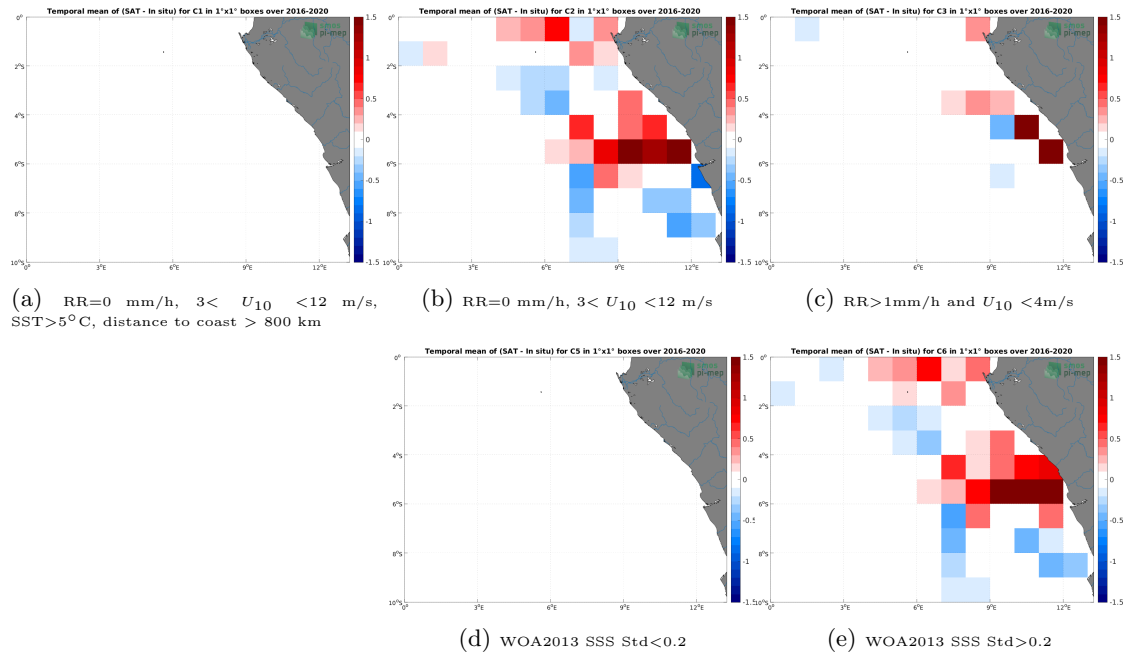
Figure 12: Temporal mean gridded over spatial boxes of size 1^{\circ}\times 1^{\circ} of \Delta\text{SSS} (CCI SSS L4 Merged-OI v3.2 - 7-day running (ESA) - TSG (LEGOS-DM)) for 5 different subdatasets corresponding to:RR=0 mm/h, 3 < U_{10} < 12 m/s, SST >5^{\circ}\text{C} , distance to coast > 800 km (a), RR=0 mm/h, 3 < U_{10} < 12 m/s (b), RR >1 mm/h and U_{10} < 4 m/s (c), WOA2013 SSS Std <0.2 (d), WOA2013 SSS Std >0.2 (e).
