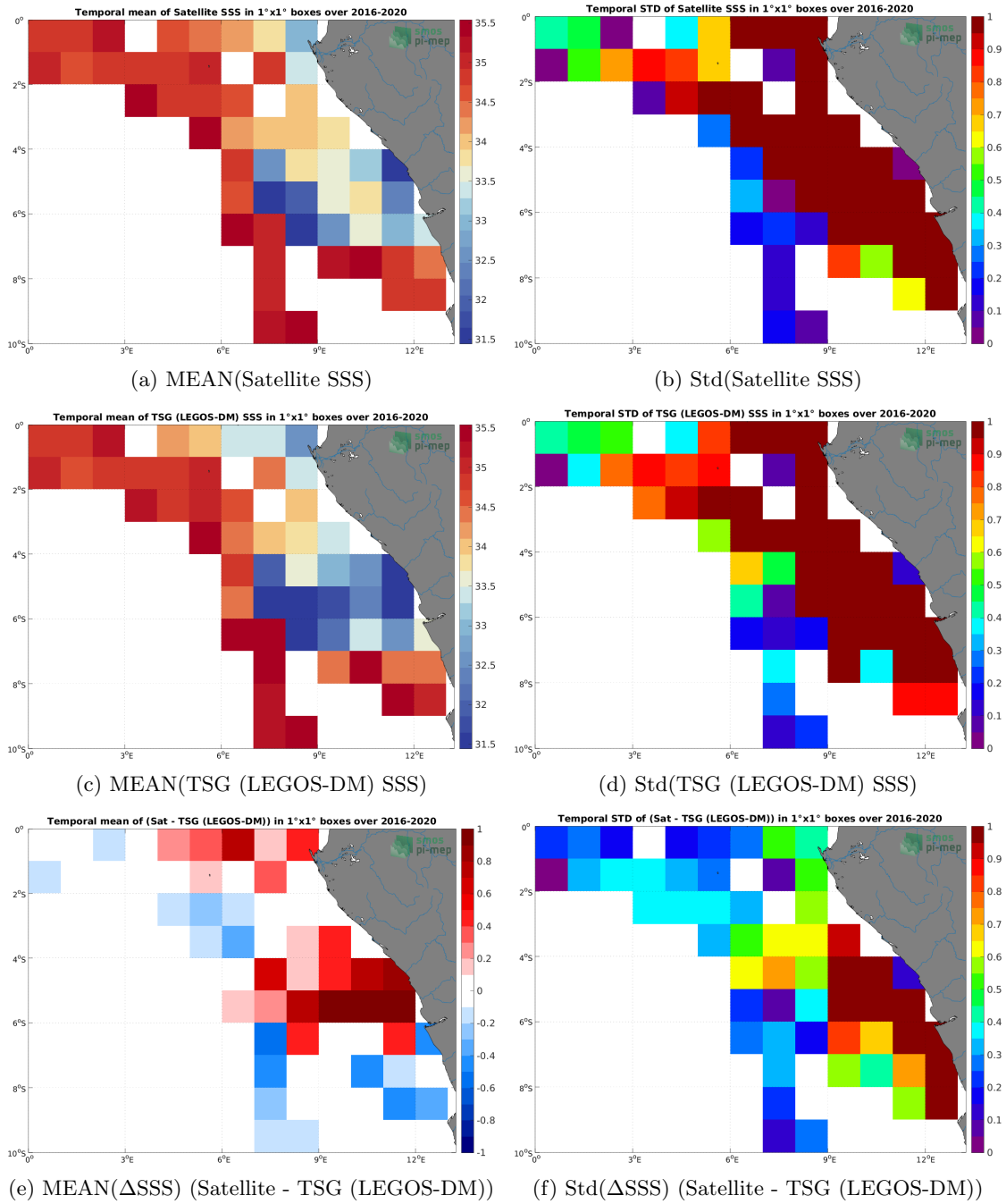
Figure 6: Temporal mean (left) and Std (right) of SSS from CCI SSS L4 Merged-OI v3.2 - 7-day running (ESA) (top), TSG (LEGOS-DM) (middle), and of \Delta SSS (Satellite - TSG (LEGOS-DM)). Only match-up pairs are used to generate these maps.
