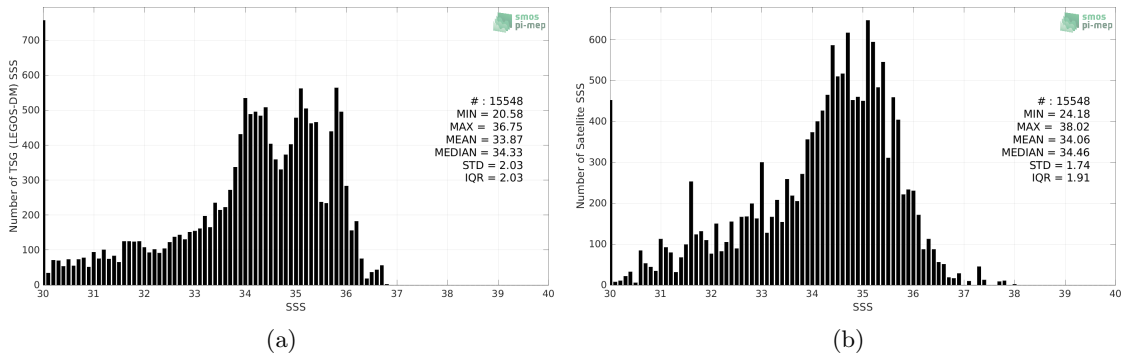
Figure 2: Histograms of SSS from TSG (LEGOS-DM) (a) and CCI SSS L4 Merged-OI v3.2 - 7-day running (ESA) (b) considering all match-up pairs per bins of 0.1 over the Congo river plume Pi-MEP region and for the full satellite product period.
