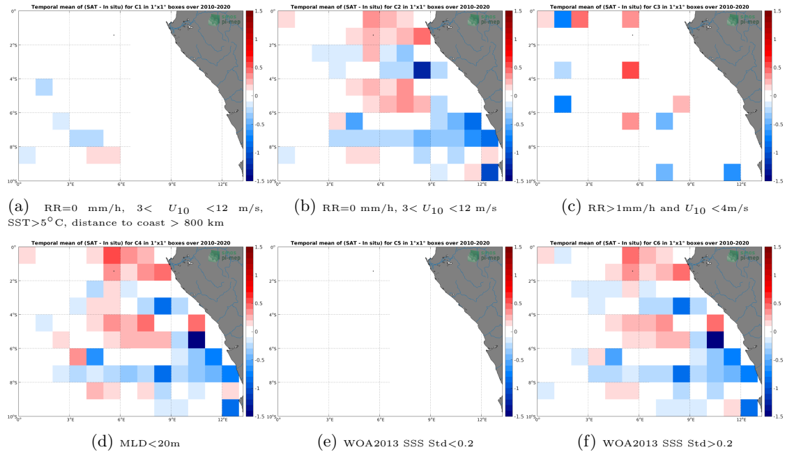
Figure 12: Temporal mean gridded over spatial boxes of size 1^\circ \times 1^\circ of \Delta SSS (CCI SSS L4 Merged-OI v3.2 - 7-day running (ESA) - Argo) for 6 different subdatasets corresponding to:RR=0 mm/h, 3 < U_{10} < 12 m/s, SST >5^\circ C, distance to coast > 800 km (a), RR=0 mm/h, 3 < U_{10} < 12 m/s (b), RR >1 mm/h and U_{10} < 4 m/s (c),MLD <20 m (d),WOA2013 SSS Std <0.2 (e),WOA2013 SSS Std >0.2 (f).
