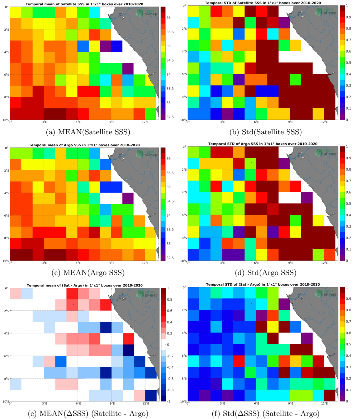
Figure 6: Temporal mean (left) and Std (right) of SSS from CCI SSS L4 Merged-OI v3.2 - 7-day running (ESA) (top), Argo (middle), and of \Delta SSS (Satellite - Argo). Only match-up pairs are used to generate these maps.
