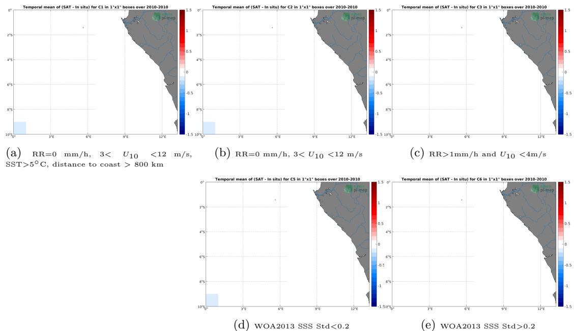
Figure 12: Temporal mean gridded over spatial boxes of size 1^\circ \times 1^\circ of \Delta\text{SSS} (CCI SSS L4 Merged-OI v3.2 - 30-day running (ESA) - TSG (SAMOS)) for 5 different subdatasets corresponding to:RR=0 mm/h, 3 < U_{10} < 12 m/s, SST >5^\circ\text{C} , distance to coast > 800 km (a), RR=0 mm/h, 3 < U_{10} < 12 m/s (b), RR >1 mm/h and U_{10} < 4 m/s (c), WOA2013 SSS Std <0.2 (d), WOA2013 SSS Std >0.2 (e).
