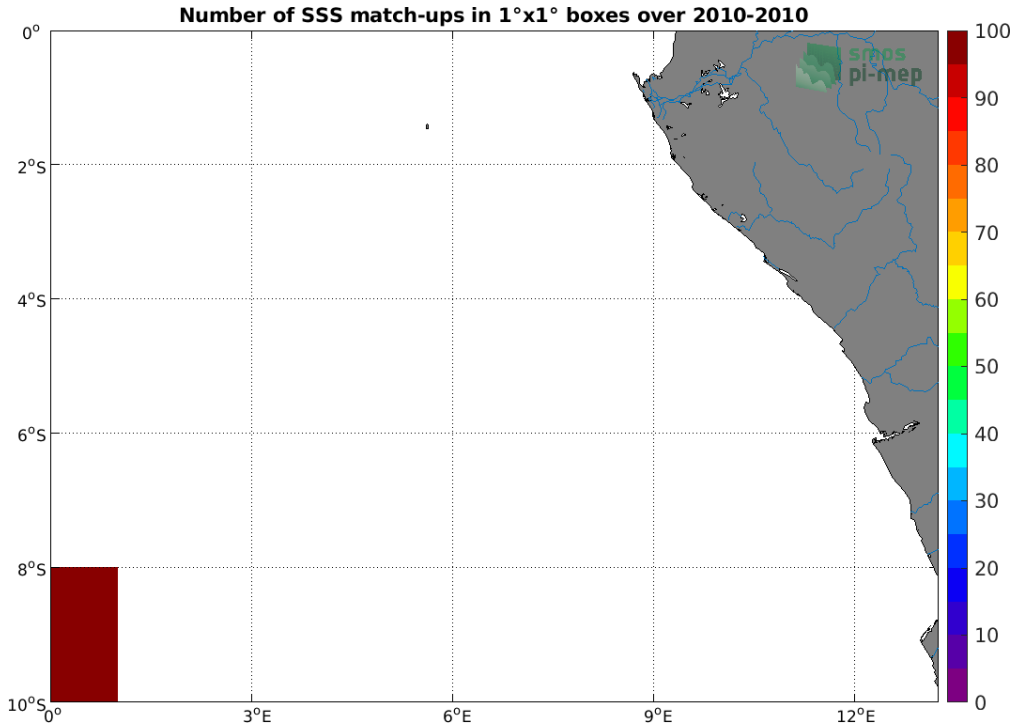
Figure 4: Number of SSS match-ups between TSG (SAMOS) SSS and the CCI SSS L4 Merged-OI v3.2 - 30-day running (ESA) SSS product for the Congo river plume Pi-MEP region over 1°x1° boxes and for the full satellite product period.
