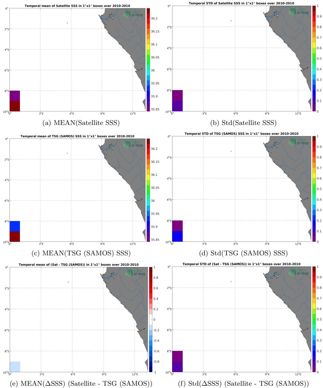
Figure 6: Temporal mean (left) and Std (right) of SSS from CCI SSS L4 Merged-OI v3.2 - 30-day running (ESA) (top), TSG (SAMOS) (middle), and of \Delta SSS (Satellite - TSG (SAMOS)). Only match-up pairs are used to generate these maps.
