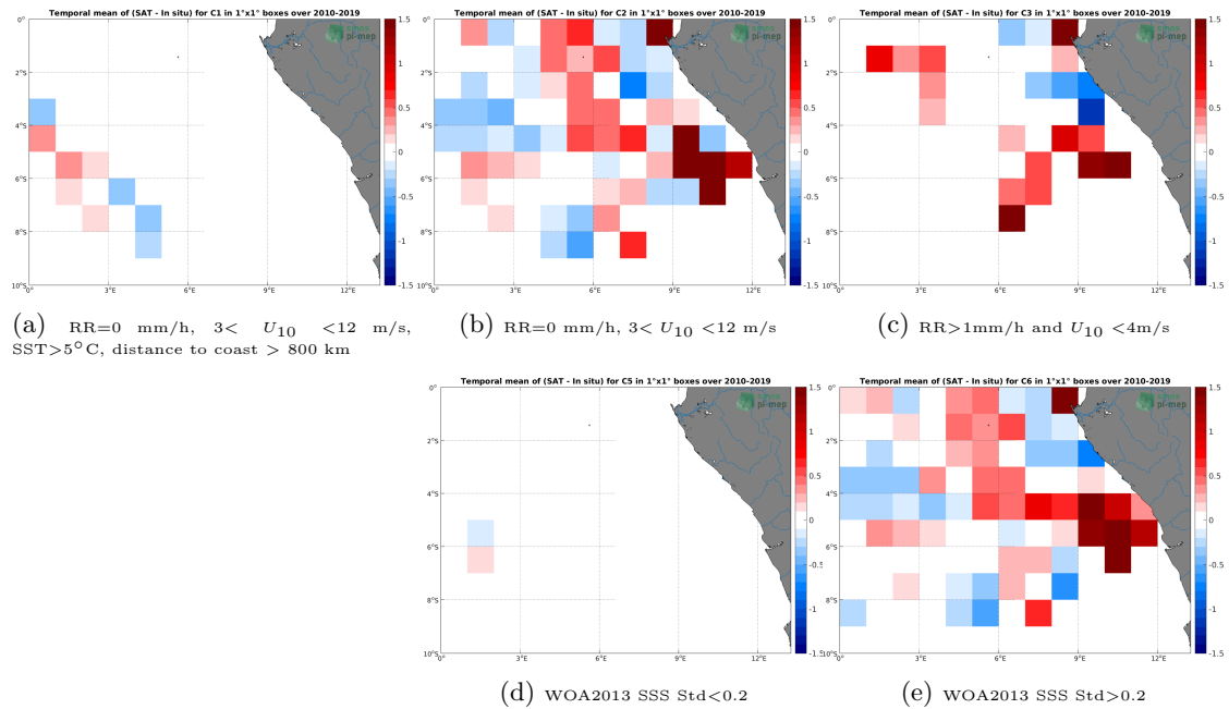
Figure 12: Temporal mean gridded over spatial boxes of size 1^\circ \times 1^\circ of \Delta SSS (CCI SSS L4 Merged-OI v3.2 - 30-day running (ESA) - TSG (GOSUD-Research-vessel)) for 5 different subdatasets corresponding to:RR=0 mm/h, 3 < U_{10} < 12 m/s, SST >5^\circ\text{C} , distance to coast > 800 km (a), RR=0 mm/h, 3 < U_{10} < 12 m/s (b), RR >1 mm/h and U_{10} < 4 m/s (c), WOA2013 SSS Std <0.2 (d), WOA2013 SSS Std >0.2 (e).
