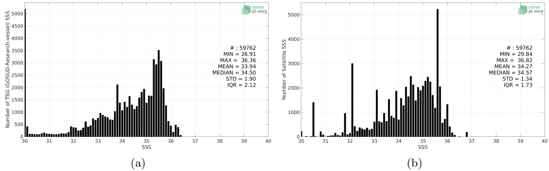
Figure 2: Histograms of SSS from TSG (GOSUD-Research-vessel) (a) and CCI SSS L4 Merged-OI v3.2 - 30-day running (ESA) (b) considering all match-up pairs per bins of 0.1 over the Congo river plume Pi-MEP region and for the full satellite product period.
