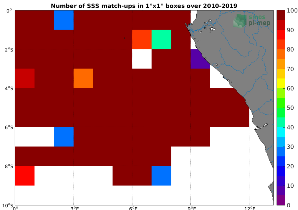
Figure 4: Number of SSS match-ups between TSG (GOSUD-Research-vessel) SSS and the CCI SSS L4 Merged-OI v3.2 - 30-day running (ESA) SSS product for the Congo river plume Pi-MEP region over 1^\circ \times 1^\circ boxes and for the full satellite product period.
