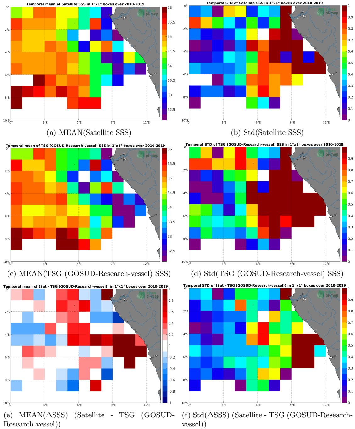
Figure 6: Temporal mean (left) and Std (right) of SSS from CCI SSS L4 Merged-OI v3.2 - 30-day running (ESA) (top), TSG (GOSUD-Research-vessel) (middle), and of \Delta SSS (Satellite - TSG (GOSUD-Research-vessel)). Only match-up pairs are used to generate these maps.
