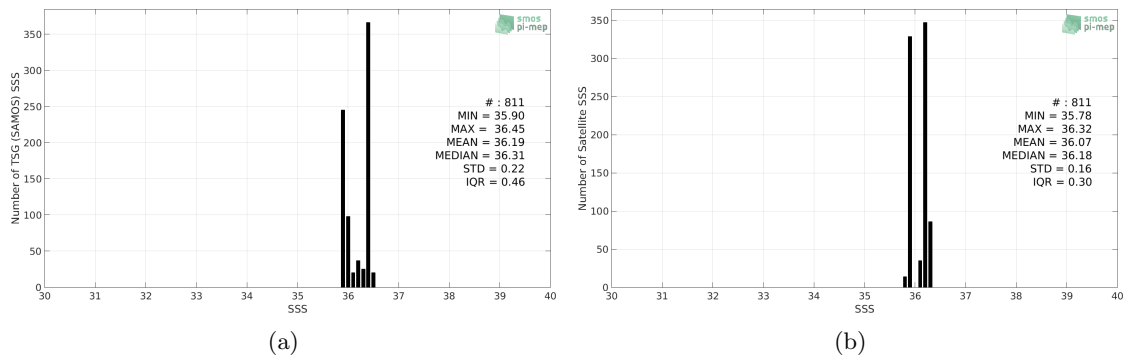
Figure 2: Histograms of SSS from TSG (SAMOS) (a) and CCI SSS L4 Merged-OI v2.31 - 7-day running (ESA) (b) considering all match-up pairs per bins of 0.1 over the Congo river plume Pi-MEP region and for the full satellite product period.
