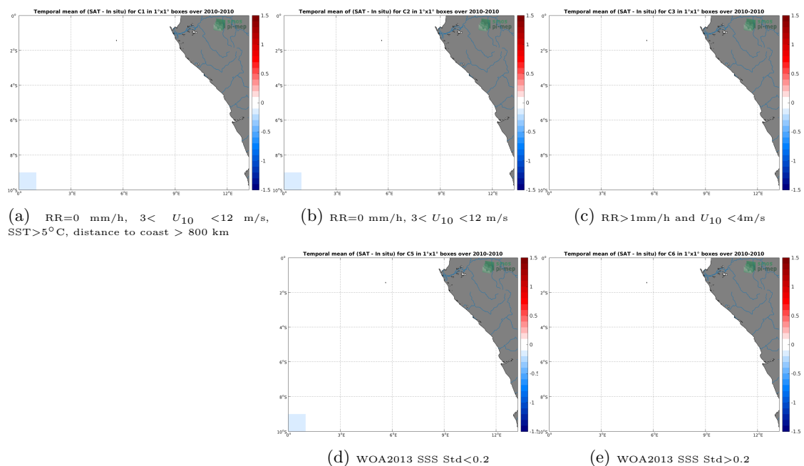
Figure 12: Temporal mean gridded over spatial boxes of size 1^\circ \times 1^\circ of \Delta SSS (CCI SSS L4 Merged-OI v2.31 - 7-day running (ESA) - TSG (SAMOS)) for 5 different subdatasets corresponding to:RR=0 mm/h, 3 < U_{10} < 12 m/s, SST >5^\circ\text{C} , distance to coast > 800 km (a), RR=0 mm/h, 3 < U_{10} < 12 m/s (b), RR >1 mm/h and U_{10} < 4 m/s (c), WOA2013 SSS Std <0.2 (d), WOA2013 SSS Std >0.2 (e).
