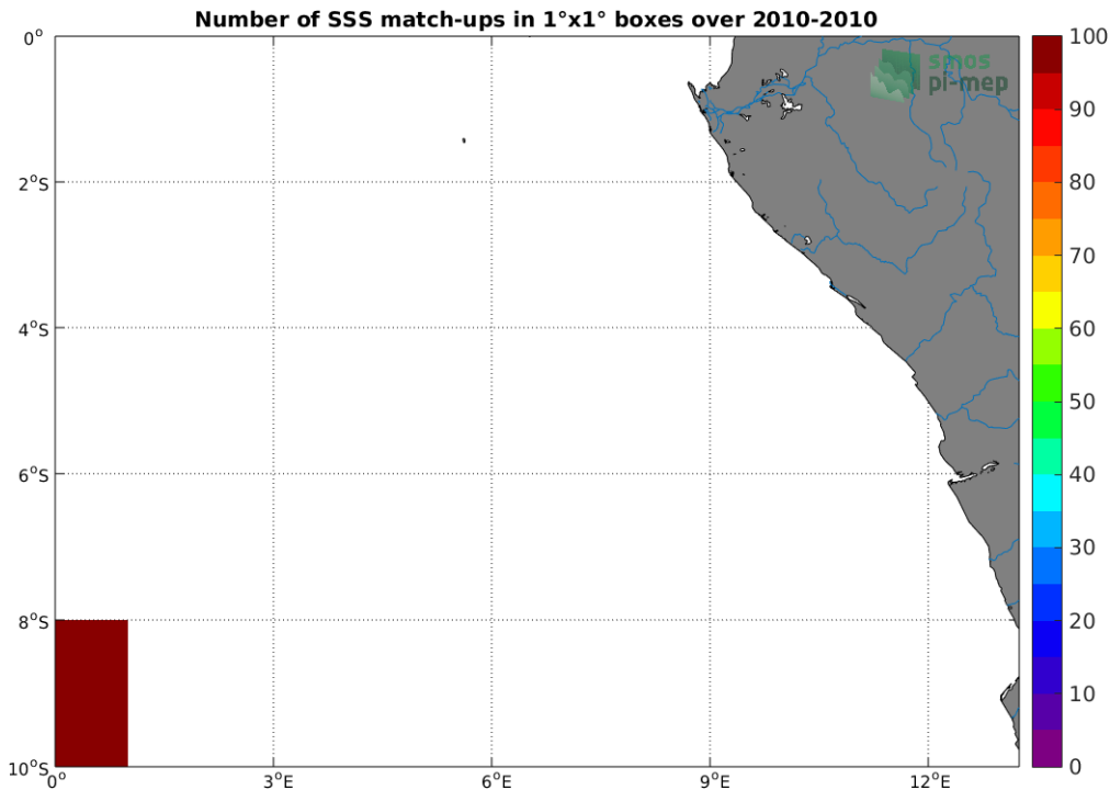
Figure 4: Number of SSS match-ups between TSG (SAMOS) SSS and the CCI SSS L4 Merged-OI v2.31 - 7-day running (ESA) SSS product for the Congo river plume Pi-MEP region over 1°x1° boxes and for the full satellite product period.
