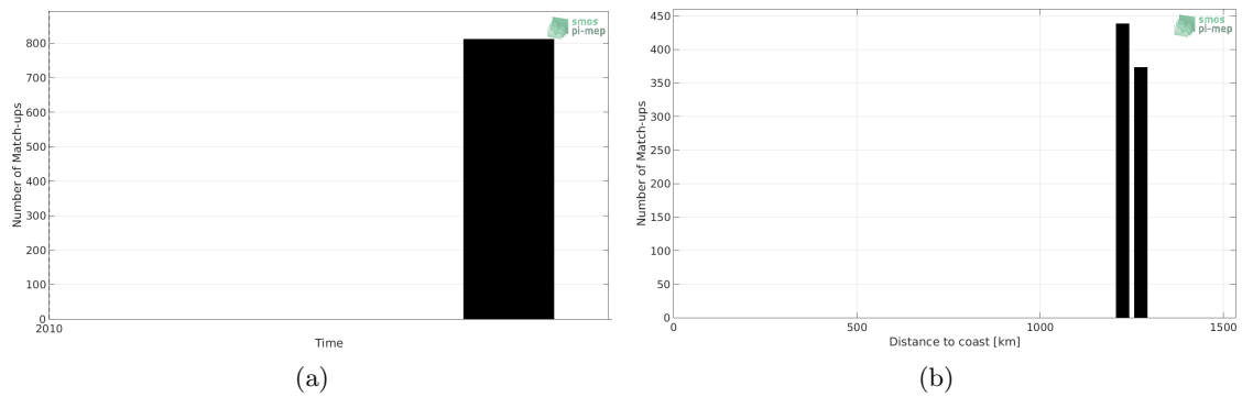
Figure 1: Number of match-ups between TSG (SAMOS) and CCI SSS L4 Merged-OI v2.31 - 7-day running (ESA) SSS as a function of time (a) and as function of the distance to coast (b) over the Congo river plume Pi-MEP region and for the full satellite product period.
