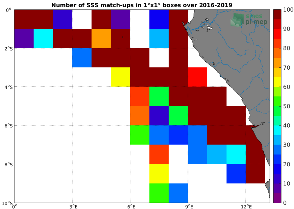
Figure 4: Number of SSS match-ups between TSG (LEGOS-DM) SSS and the CCI SSS L4 Merged-OI v2.31 - 7-day running (ESA) SSS product for the Congo river plume Pi-MEP region over 1^\circ \times 1^\circ boxes and for the full satellite product period.
