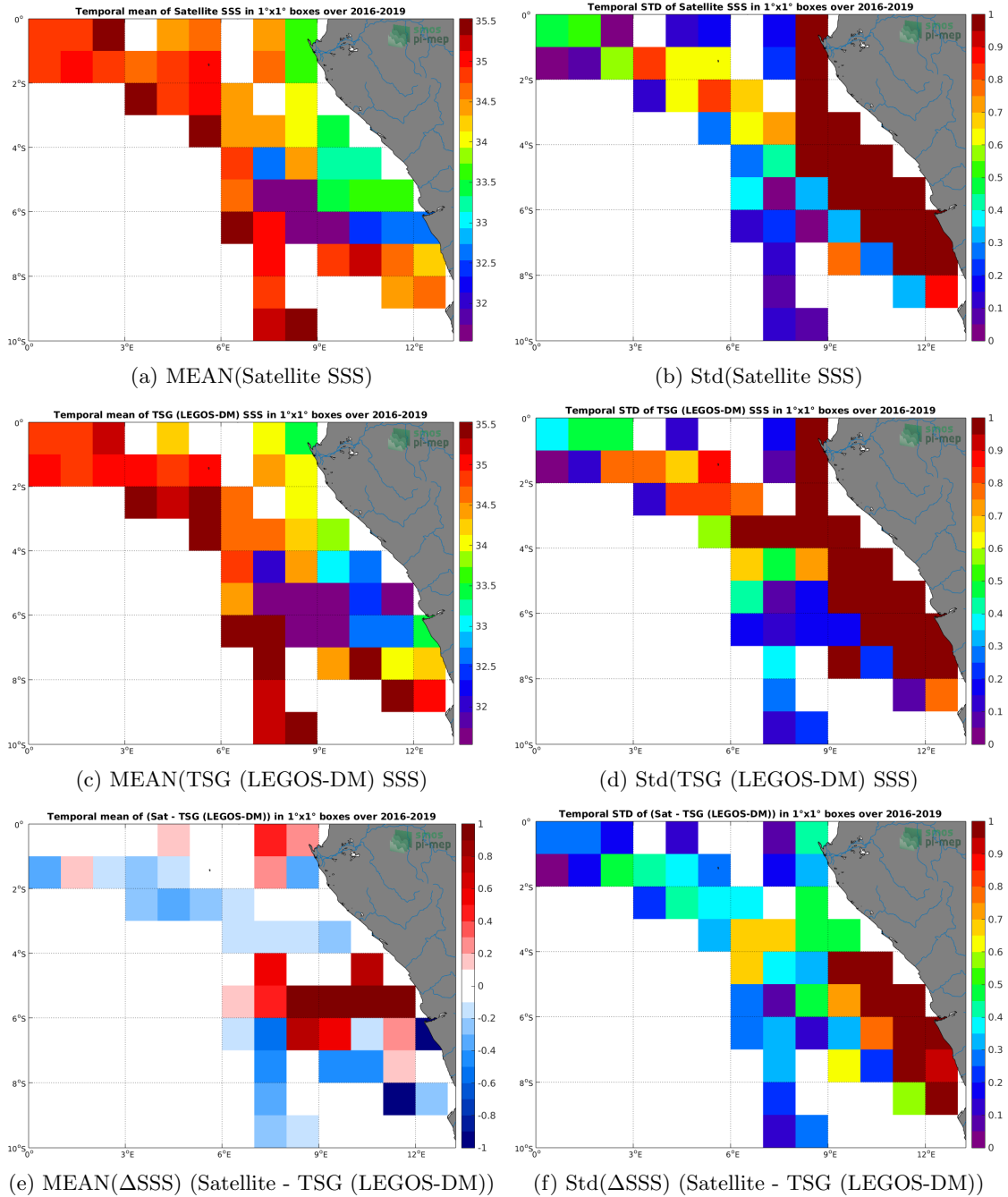
Figure 6: Temporal mean (left) and Std (right) of SSS from CCI SSS L4 Merged-OI v2.31 - 7-day running (ESA) (top), TSG (LEGOS-DM) (middle), and of \Delta SSS (Satellite - TSG (LEGOS-DM)). Only match-up pairs are used to generate these maps.
