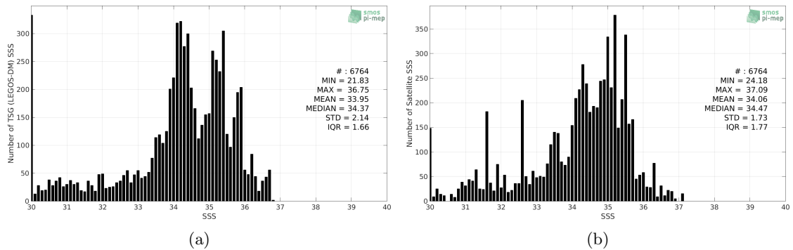
Figure 2: Histograms of SSS from TSG (LEGOS-DM) (a) and CCI SSS L4 Merged-OI v2.31 - 7-day running (ESA) (b) considering all match-up pairs per bins of 0.1 over the Congo river plume Pi-MEP region and for the full satellite product period.
