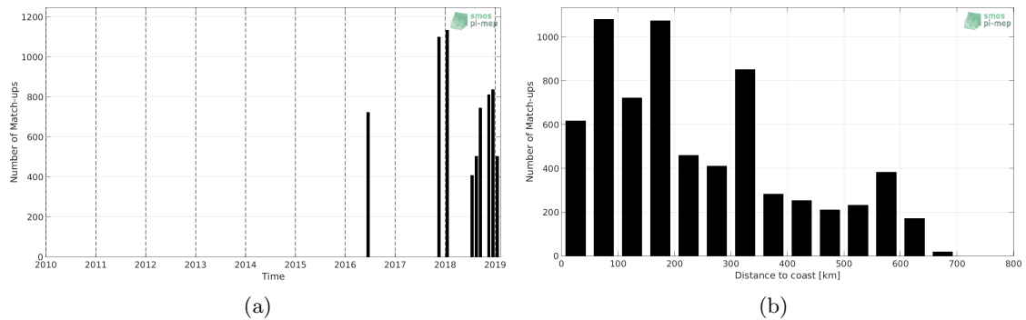
Figure 1: Number of match-ups between TSG (LEGOS-DM) and CCI SSS L4 Merged-OI v2.31 - 7-day running (ESA) SSS as a function of time (a) and as function of the distance to coast (b) over the Congo river plume Pi-MEP region and for the full satellite product period.
