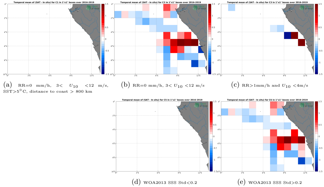
Figure 12: Temporal mean gridded over spatial boxes of size 1^{\circ}\times 1^{\circ} of \Delta\text{SSS} (CCI SSS L4 Merged-OI v2.31 - 7-day running (ESA) - TSG (LEGOS-DM)) for 5 different subdatasets corresponding to:RR=0 mm/h, 3 < U_{10} < 12 m/s, SST >5^{\circ}\text{C} , distance to coast > 800 km (a), RR=0 mm/h, 3 < U_{10} < 12 m/s (b), RR >1 mm/h and U_{10} < 4 m/s (c), WOA2013 SSS Std <0.2 (d), WOA2013 SSS Std >0.2 (e).
