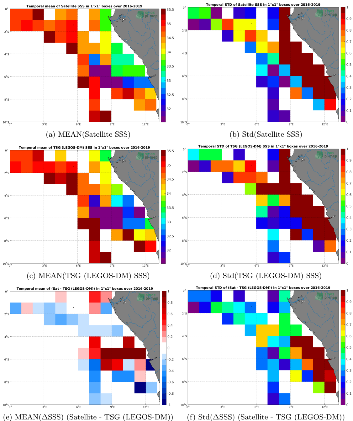
Figure 6: Temporal mean (left) and Std (right) of SSS from CCI L4 Merged-OI v2.31 - 7-day running (ESA) (top), TSG (LEGOS-DM) (middle), and of \Delta SSS (Satellite - TSG (LEGOS-DM)). Only match-up pairs are used to generate these maps.
