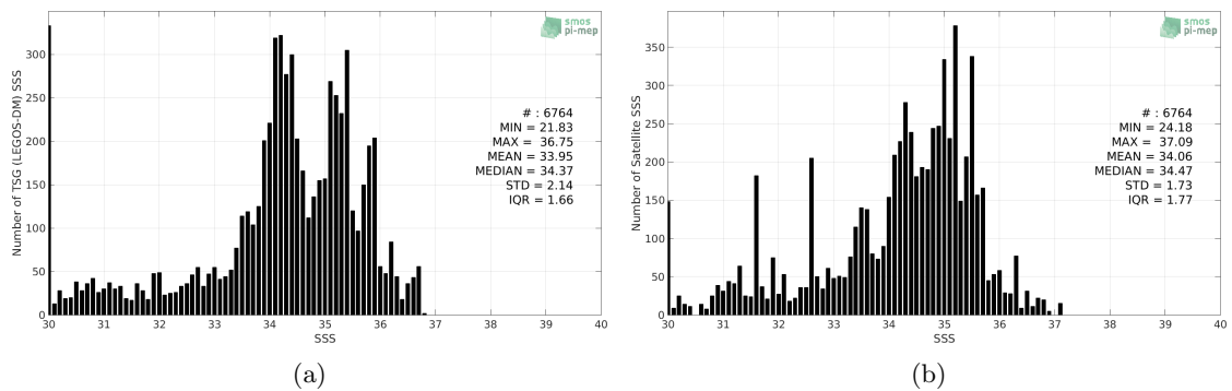
Figure 2: Histograms of SSS from TSG (LEGOS-DM) (a) and CCI L4 Merged-OI v2.31 - 7-day running (ESA) (b) considering all match-up pairs per bins of 0.1 over the Congo river plume Pi-MEP region and for the full satellite product period.
