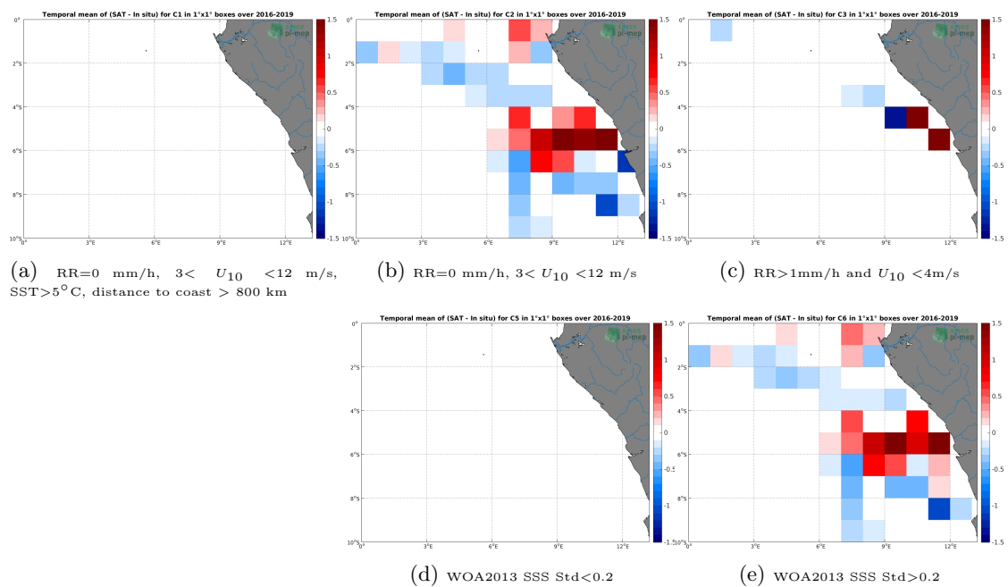
Figure 12: Temporal mean gridded over spatial boxes of size 1^\circ \times 1^\circ of \Delta SSS (CCI L4 Merged-OI v2.31 - 7-day running (ESA) - TSG (LEGOS-DM)) for 5 different subdatasets corresponding to:RR=0 mm/h, 3 < U_{10} < 12 m/s, SST >5^\circ\text{C} , distance to coast > 800 km (a), RR=0 mm/h, 3 < U_{10} < 12 m/s (b), RR >1 mm/h and U_{10} < 4 m/s (c), WOA2013 SSS Std <0.2 (d), WOA2013 SSS Std >0.2 (e).
