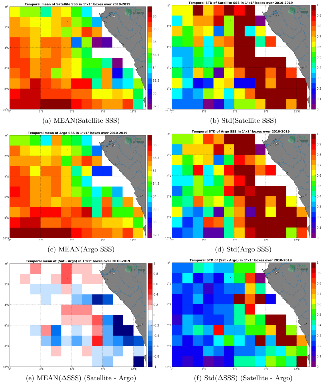
Figure 6: Temporal mean (left) and Std (right) of SSS from CCI SSS L4 Merged-OI v2.31 - 7-day running (ESA) (top), Argo (middle), and of \Delta SSS (Satellite - Argo). Only match-up pairs are used to generate these maps.
