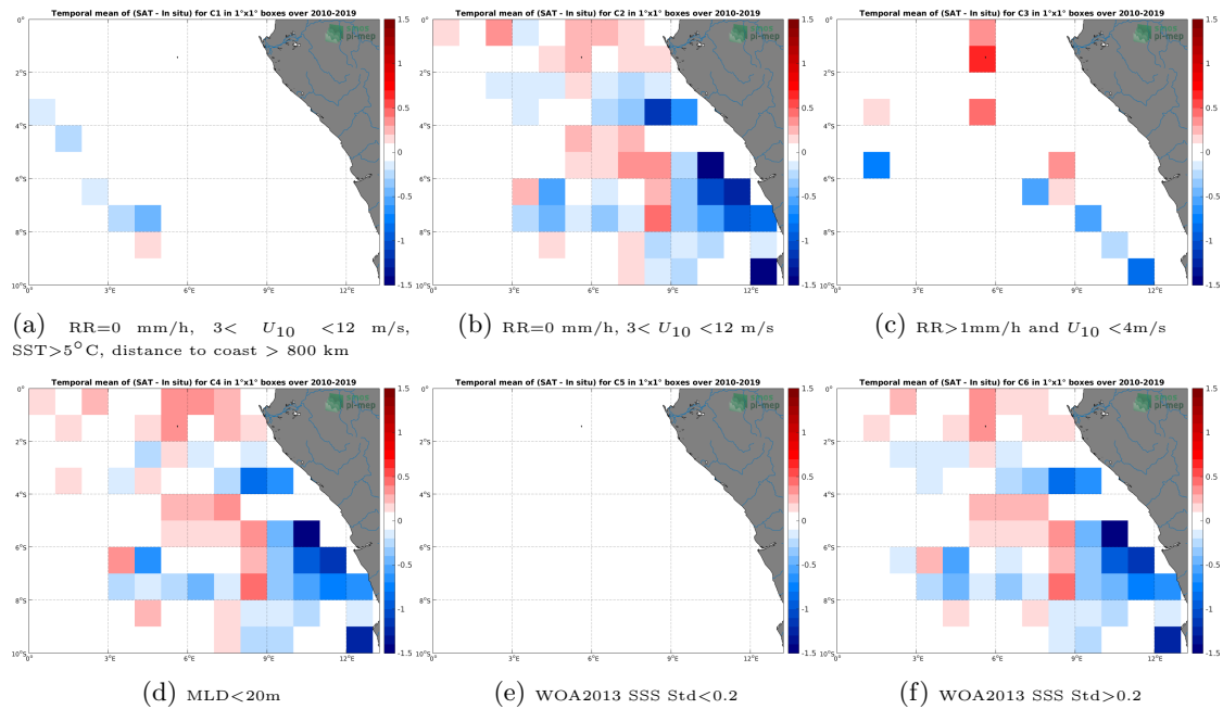
Figure 12: Temporal mean gridded over spatial boxes of size 1^\circ \times 1^\circ of \Delta SSS (CCI SSS L4 Merged-OI v2.31 - 7-day running (ESA) - Argo) for 6 different subdatasets corresponding to:RR=0 mm/h, 3 < U_{10} < 12 m/s, SST >5^\circ\text{C} , distance to coast > 800 km (a), RR=0 mm/h, 3 < U_{10} < 12 m/s (b), RR >1 mm/h and U_{10} < 4 m/s (c),MLD <20 m (d),WOA2013 SSS Std <0.2 (e),WOA2013 SSS Std >0.2 (f).
