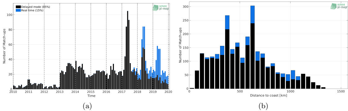
Figure 1: Number of match-ups between Argo and CCI SSS L4 Merged-OI v2.31 - 7-day running (ESA) SSS as a function of time (a) and as function of the distance to coast (b) over the Congo river plume Pi-MEP region and for the full satellite product period.
