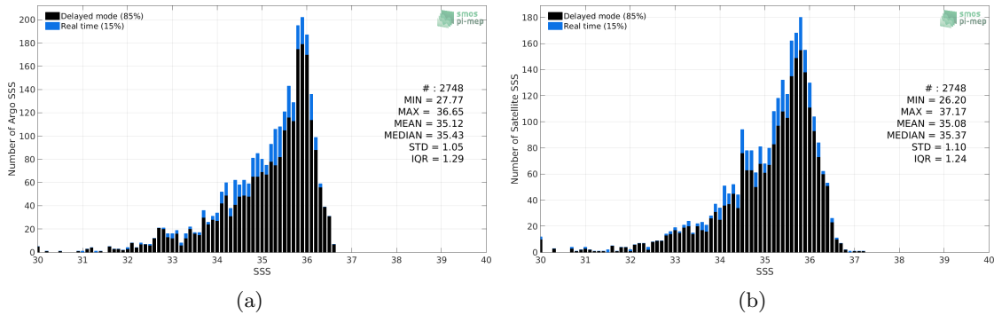
Figure 2: Histograms of SSS from Argo (a) and CCI SSS L4 Merged-OI v2.31 - 7-day running (ESA) (b) considering all match-up pairs per bins of 0.1 over the Congo river plume Pi-MEP region and for the full satellite product period.
