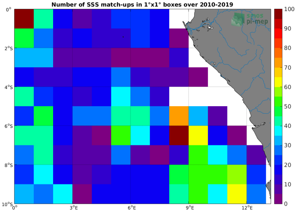
Figure 4: Number of SSS match-ups between Argo SSS and the CCI SSS L4 Merged-OI v2.31 - 7-day running (ESA) SSS product for the Congo river plume Pi-MEP region over 1^\circ \times 1^\circ boxes and for the full satellite product period.
