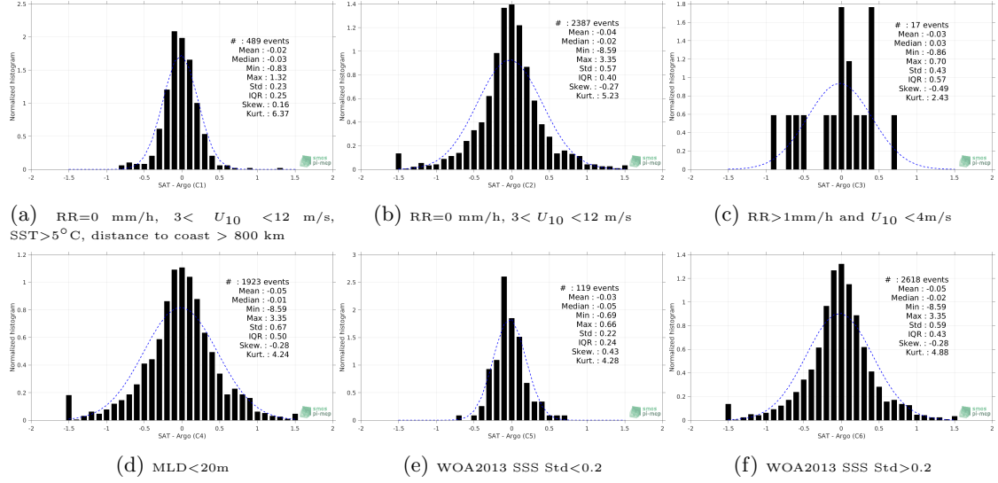
Figure 13: Normalized histogram of \Delta SSS (CCI SSS L4 Merged-OI v2.31 - 7-day running (ESA) - Argo) for 6 different subdatasets corresponding to: RR=0 mm/h, 3 < U_{10} < 12 m/s, SST>5°C, distance to coast > 800 km (a), RR=0 mm/h, 3 < U_{10} < 12 m/s (b), RR>1mm/h and U_{10} < 4 m/s (c), MLD<20m (d), WOA2013 SSS Std<0.2 (e), WOA2013 SSS Std>0.2 (f).
