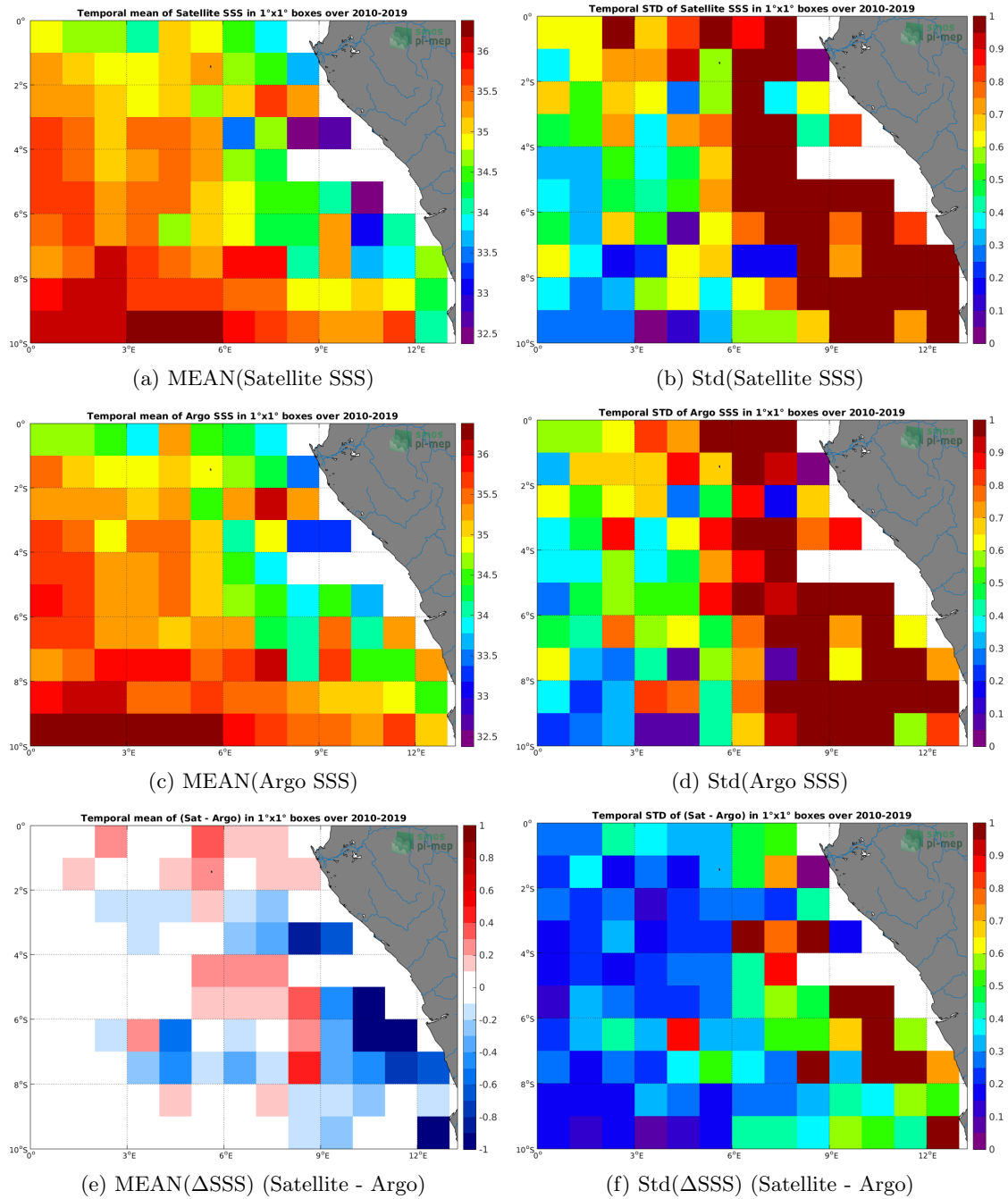
Figure 6: Temporal mean (left) and Std (right) of SSS from CCI L4 Merged-OI v2.31 - 7-day running (ESA) (top), Argo (middle), and of \Delta SSS (Satellite - Argo). Only match-up pairs are used to generate these maps.
