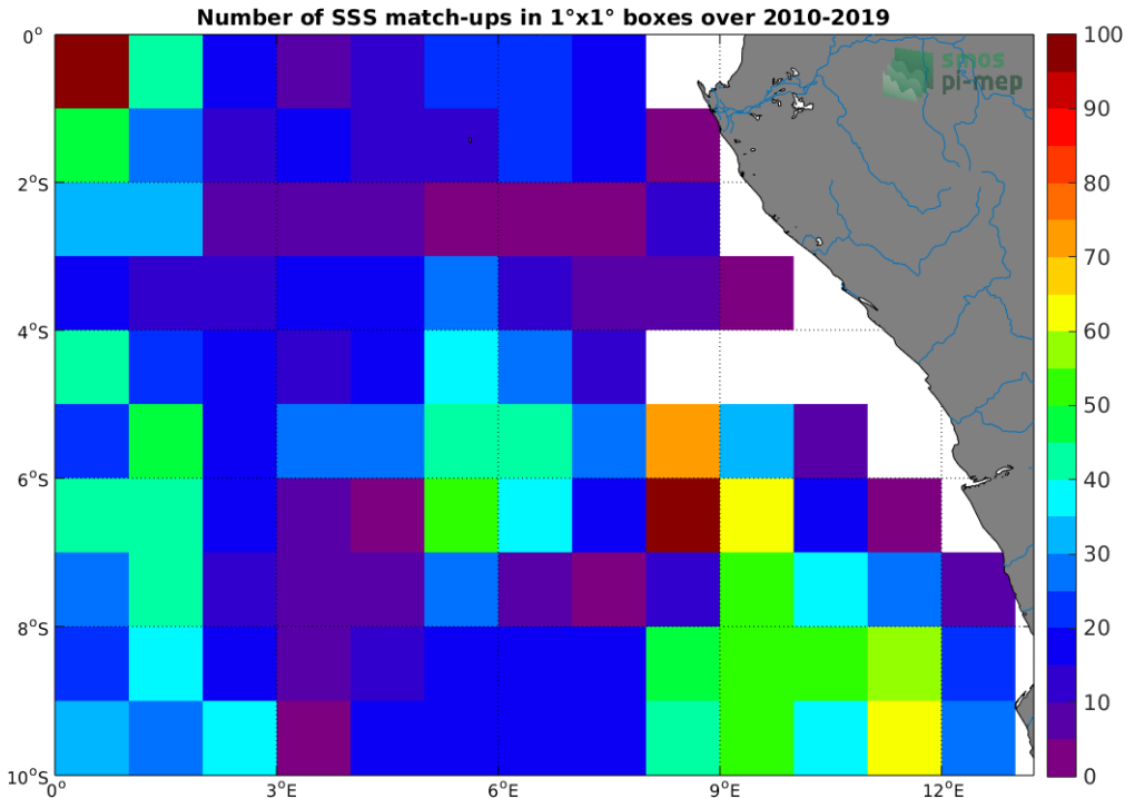
Figure 4: Number of SSS match-ups between Argo SSS and the CCI L4 Merged-OI v2.31 - 7-day running (ESA) SSS product for the Congo river plume Pi-MEP region over 1°x1° boxes and for the full satellite product period.
