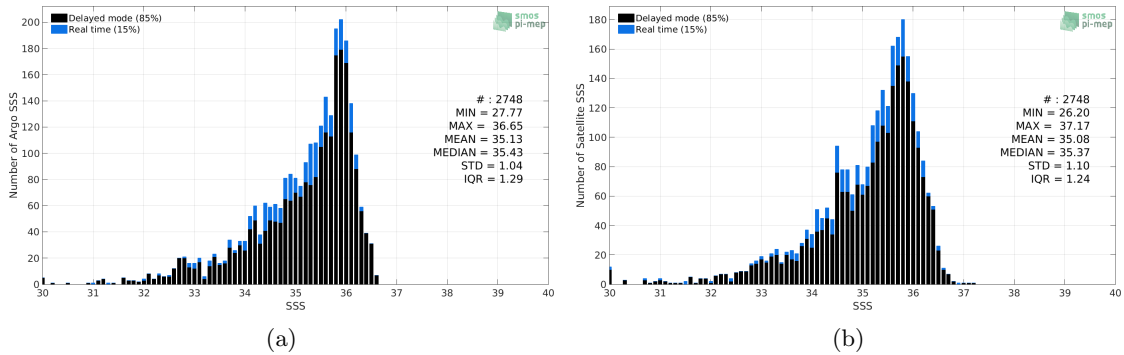
Figure 2: Histograms of SSS from Argo (a) and CCI L4 Merged-OI v2.31 - 7-day running (ESA) (b) considering all match-up pairs per bins of 0.1 over the Congo river plume Pi-MEP region and for the full satellite product period.
