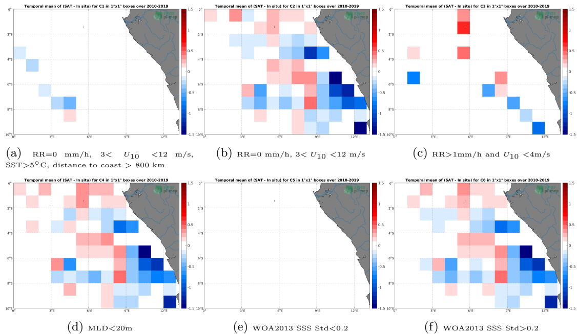
Figure 12: Temporal mean gridded over spatial boxes of size 1^\circ \times 1^\circ of \Delta SSS (CCI L4 Merged-OI v2.31 - 7-day running (ESA) - Argo) for 6 different subdatasets corresponding to:RR=0 mm/h, 3 < U_{10} < 12 m/s, SST >5^\circ\text{C} , distance to coast > 800 km (a), RR=0 mm/h, 3 < U_{10} < 12 m/s (b), RR >1 mm/h and U_{10} < 4 m/s (c),MLD <20 m (d),WOA2013 SSS Std <0.2 (e),WOA2013 SSS Std >0.2 (f).
