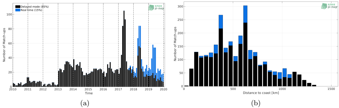
Figure 1: Number of match-ups between Argo and CCI L4 Merged-OI v2.31 - 7-day running (ESA) SSS as a function of time (a) and as function of the distance to coast (b) over the Congo river plume Pi-MEP region and for the full satellite product period.
