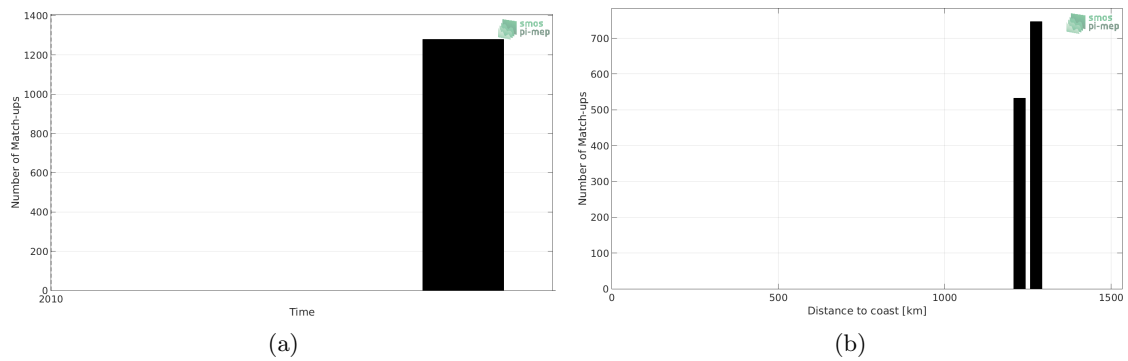
Figure 1: Number of match-ups between TSG (SAMOS) and CCI L4 Merged-OI v2.31 - 30-day running (ESA) SSS as a function of time (a) and as function of the distance to coast (b) over the Congo river plume Pi-MEP region and for the full satellite product period.
