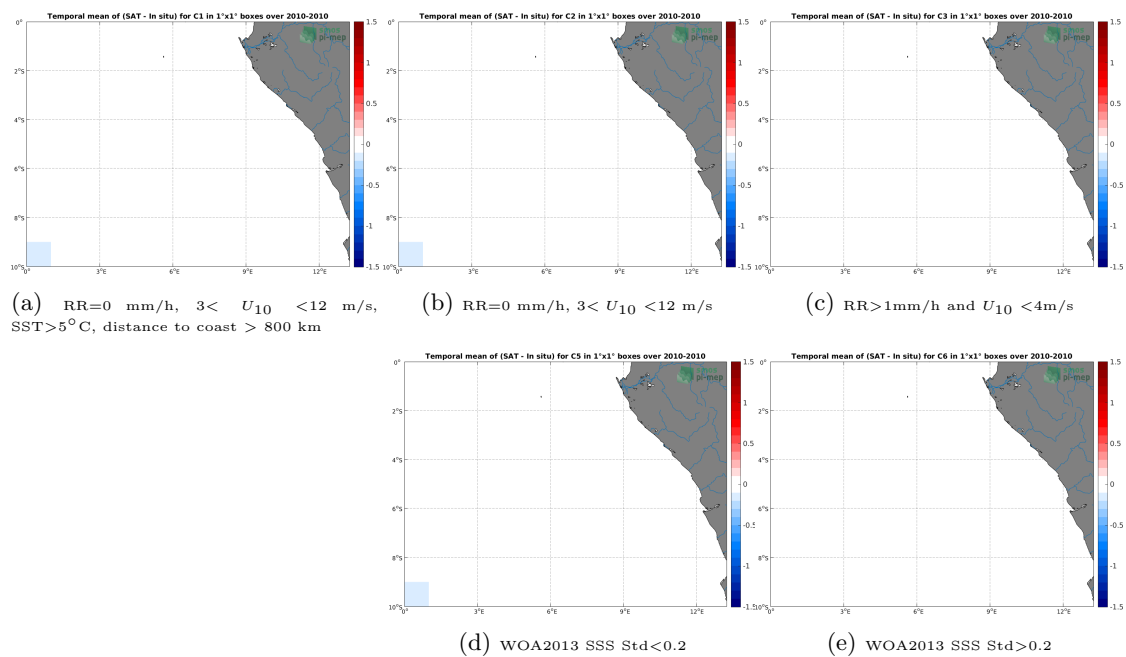
Figure 12: Temporal mean gridded over spatial boxes of size 1^\circ \times 1^\circ of \Delta SSS (CCI L4 Merged-OI v2.31 - 30-day running (ESA) - TSG (SAMOS)) for 5 different subdatasets corresponding to:RR=0 mm/h, 3 < U_{10} < 12 m/s, SST >5^\circ\text{C} , distance to coast > 800 km (a), RR=0 mm/h, 3 < U_{10} < 12 m/s (b), RR >1 mm/h and U_{10} < 4 m/s (c), WOA2013 SSS Std <0.2 (d), WOA2013 SSS Std >0.2 (e).
