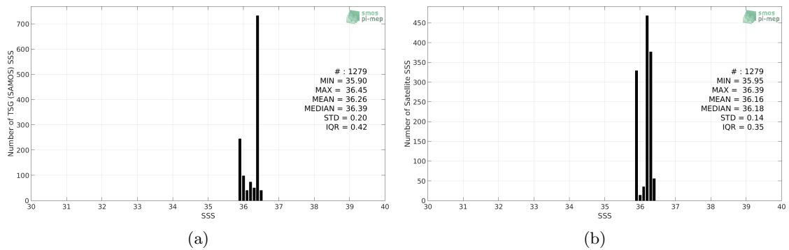
Figure 2: Histograms of SSS from TSG (SAMOS) (a) and CCI L4 Merged-OI v2.31 - 30-day running (ESA) (b) considering all match-up pairs per bins of 0.1 over the Congo river plume Pi-MEP region and for the full satellite product period.
