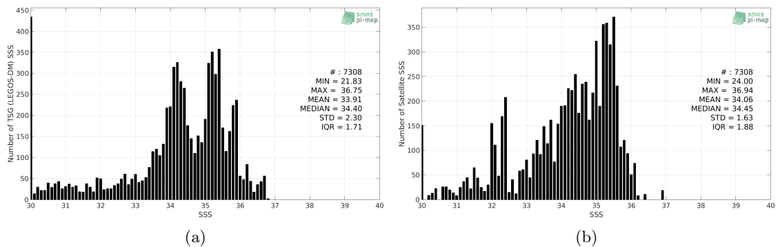
Figure 2: Histograms of SSS from TSG (LEGOS-DM) (a) and CCI L4 Merged-OI v2.31 - 30-day running (ESA) (b) considering all match-up pairs per bins of 0.1 over the Congo river plume Pi-MEP region and for the full satellite product period.
