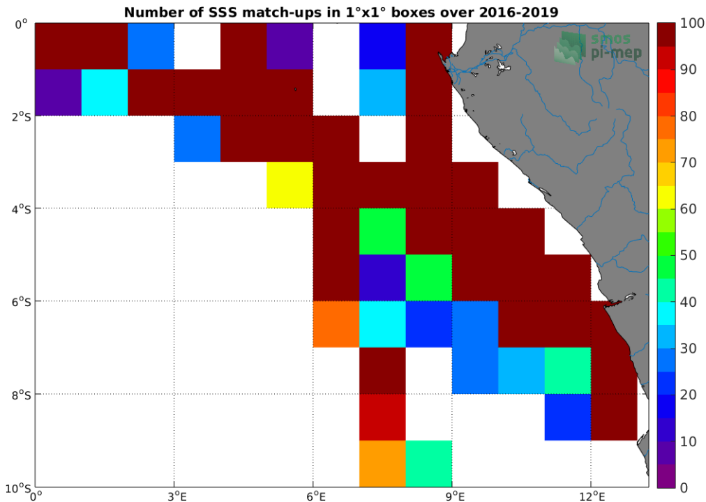
Figure 4: Number of SSS match-ups between TSG (LEGOS-DM) SSS and the CCI L4 Merged-OI v2.31 - 30-day running (ESA) SSS product for the Congo river plume Pi-MEP region over 1°x1° boxes and for the full satellite product period.
