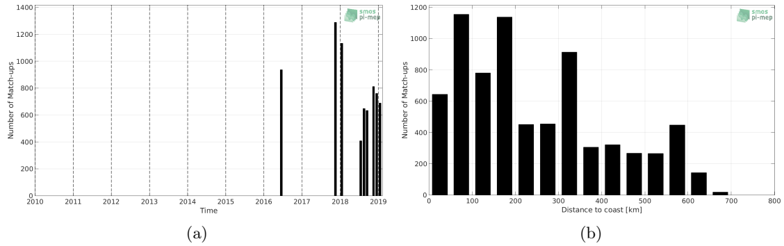
Figure 1: Number of match-ups between TSG (LEGOS-DM) and CCI L4 Merged-OI v2.31 - 30-day running (ESA) SSS as a function of time (a) and as function of the distance to coast (b) over the Congo river plume Pi-MEP region and for the full satellite product period.
