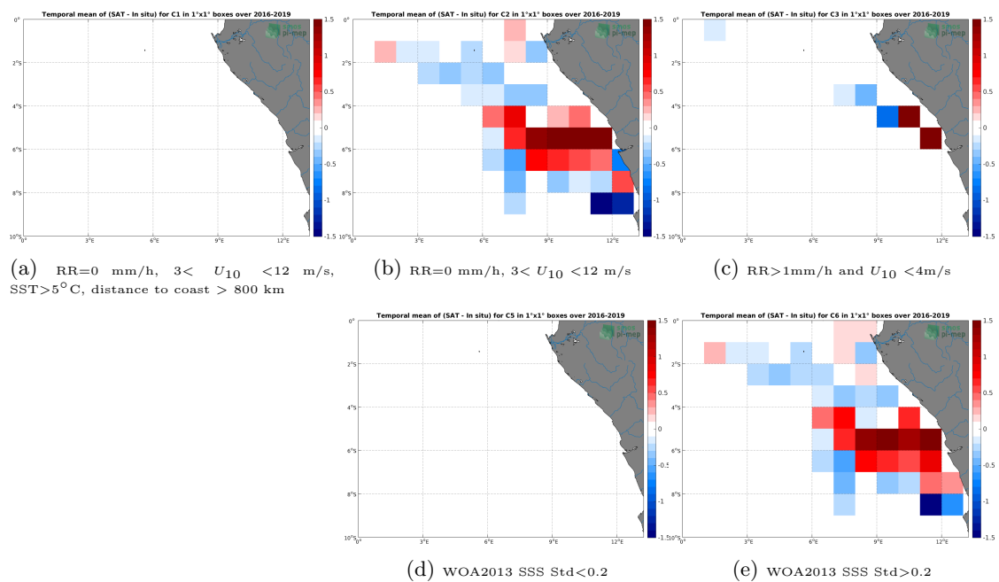
Figure 12: Temporal mean gridded over spatial boxes of size 1^\circ \times 1^\circ of \Delta SSS (CCI L4 Merged-OI v2.31 - 30-day running (ESA) - TSG (LEGOS-DM)) for 5 different subdatasets corresponding to:RR=0 mm/h, 3 < U_{10} < 12 m/s, SST >5^\circ C, distance to coast > 800 km (a), RR=0 mm/h, 3 < U_{10} < 12 m/s (b), RR >1 mm/h and U_{10} < 4 m/s (c), WOA2013 SSS Std <0.2 (d), WOA2013 SSS Std >0.2 (e).
